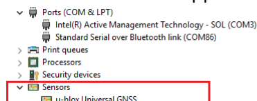
Figure 8: Device Manager
