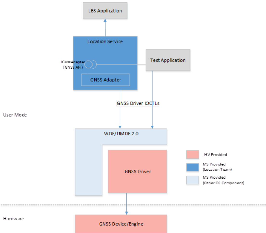
Figure 2: Universal GNSS driver architecture
