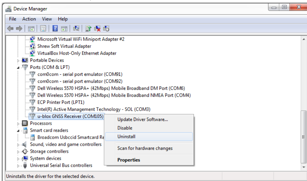
Figure 26: Uninstall the CDC-ACM driver from Device Manager
