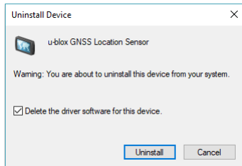
Figure 16: Selection to delete all the driver files for the device
