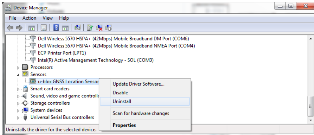
Figure 29: Uninstalling legacy Sensor driver from Device Manager
