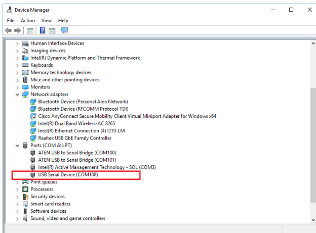
Figure 5: Loaded CDC-ACM driver in Windows 10
