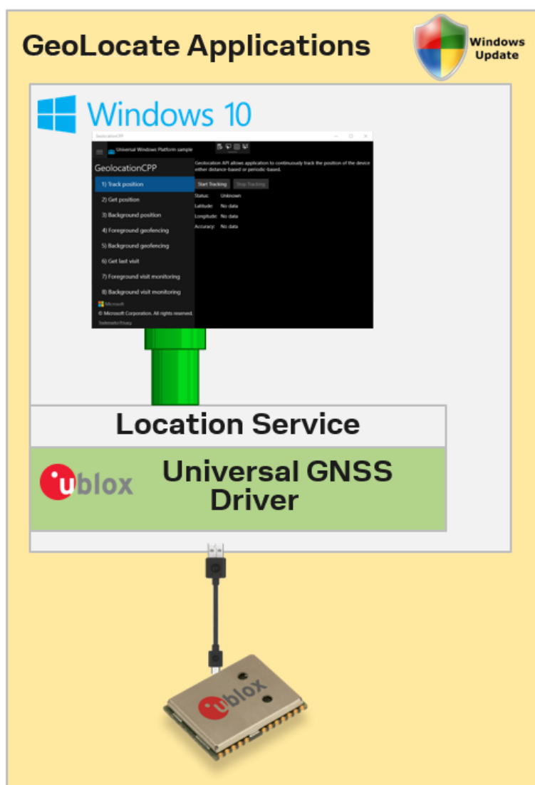
Figure 1: Standard driver application
