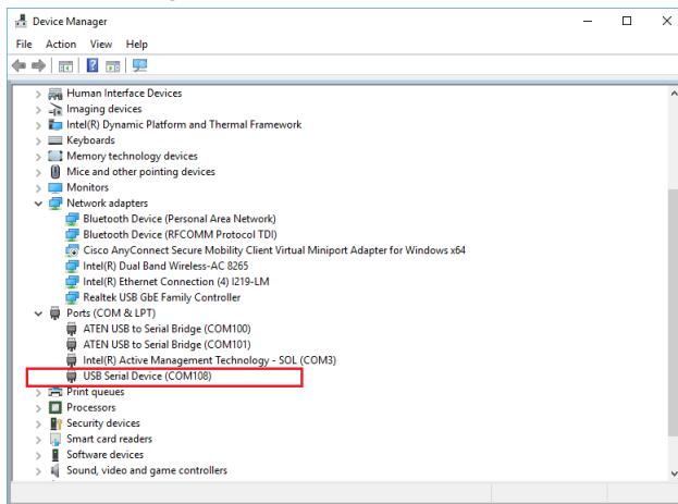
Figure 25: Updated CDC-ACM driver from Windows Update
