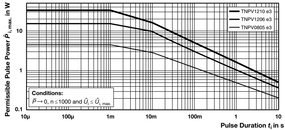
Maximum Pulse Load \hat{P}_{i, \max} . Single Pulses
