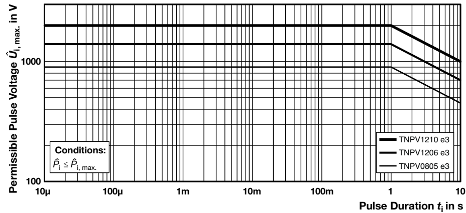
Maximum Pulse Voltage \hat{U}_{i, \max}
