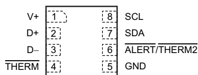
Figure 5-1. DQF Package 8-Pin WSON Top View
