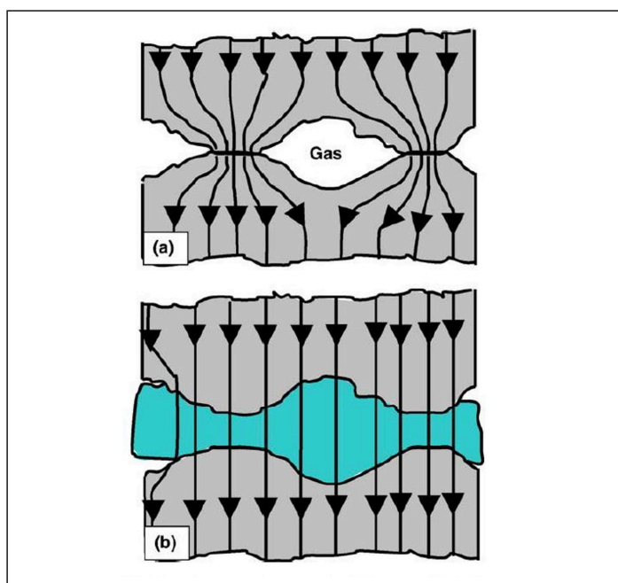
Figure 5 A schematic of two contacting bodies: (a) in direct contact and (b) separated by a thermal interface material. The arrows denote the heat flow across the interface.
