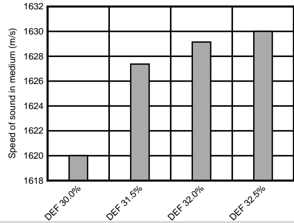
Figure 56. Speed of Sound of Various Diesel Exhaust Fluid (DEF) Concentrations
