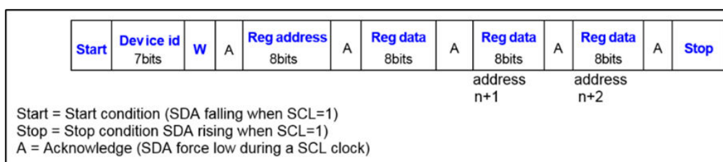
Figure 18. I 2 C write operation
