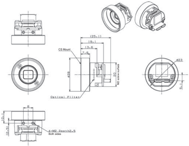
STC-S133UVC-BSCS(DBSCS)
