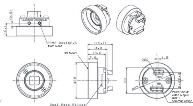
STC-S133N(P)/ICS
