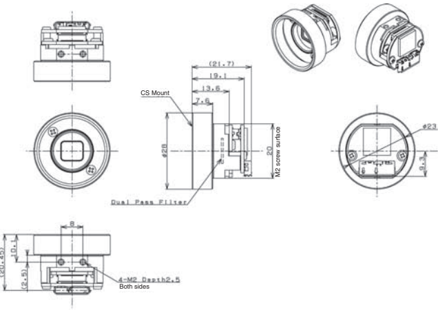
STC-S133UVC-BLCS(DBLCS)
