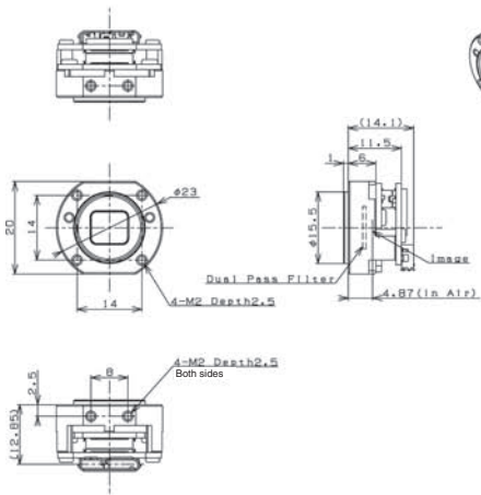
STC-S133UVC-BL(DBL)
