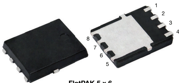
FlatPAK 5 x 6
