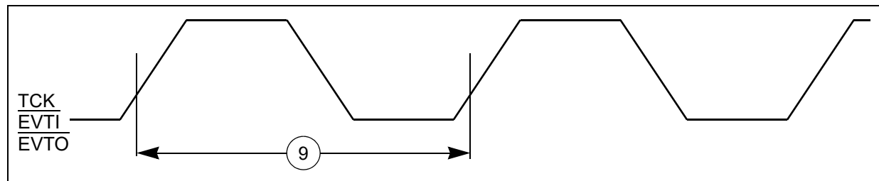
Figure 20. Nexus event trigger and test clock timings
