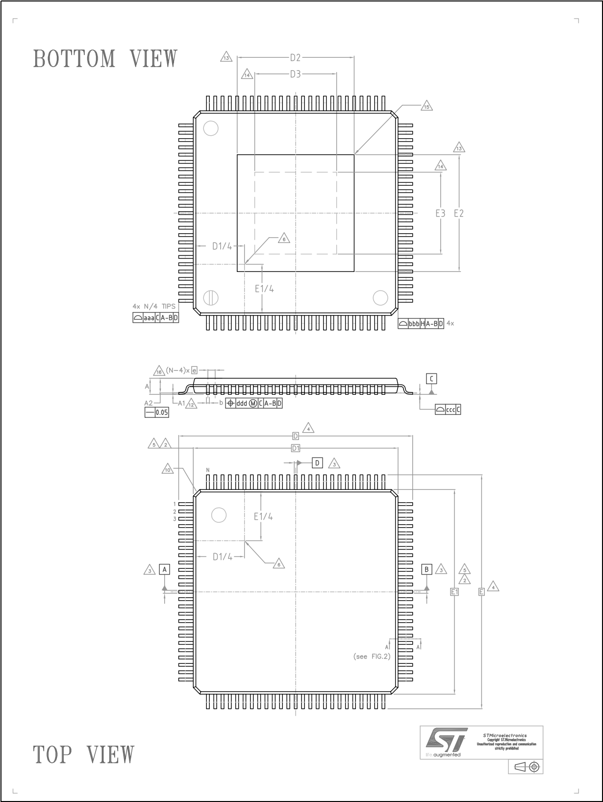
Figure 28. eTQFP100 package outline
