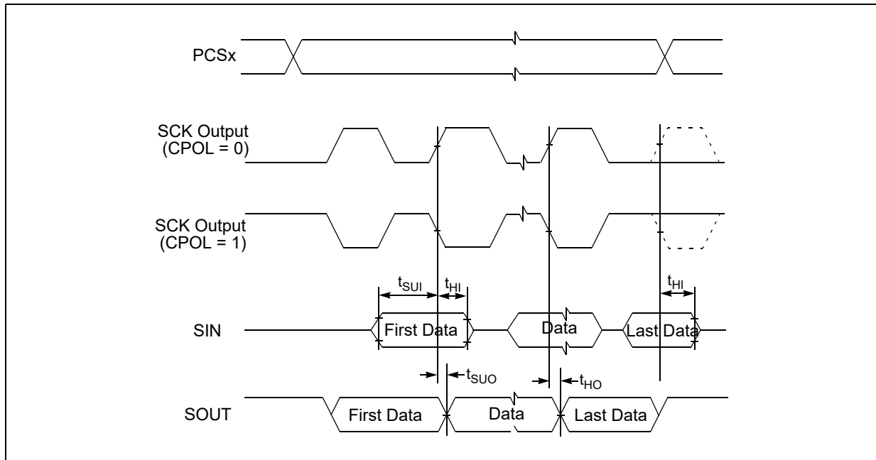
Figure 26. DSPI CMOS master mode – modified timing, CPHA = 1
