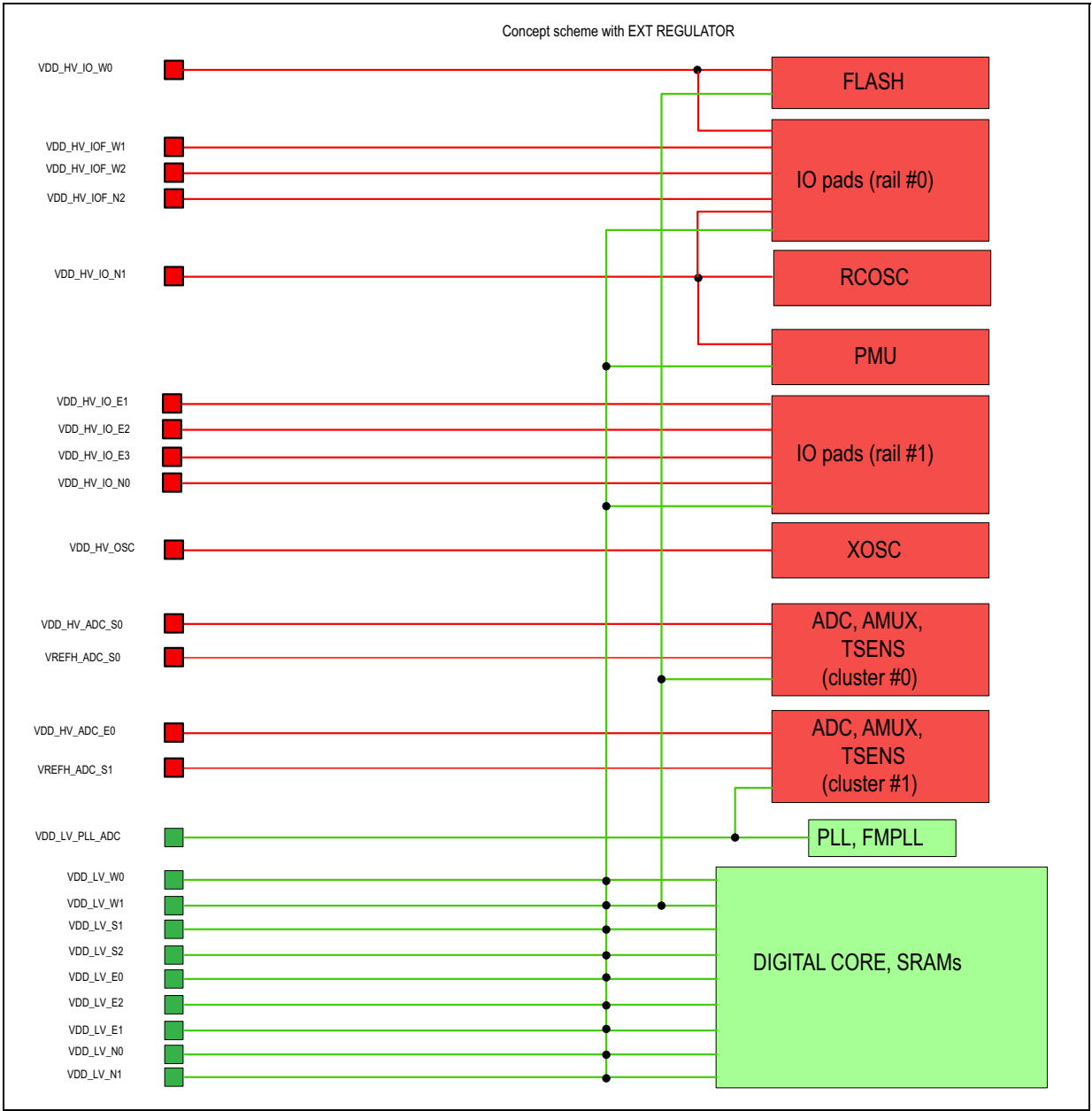
Figure 8. Concept scheme of the power connections
