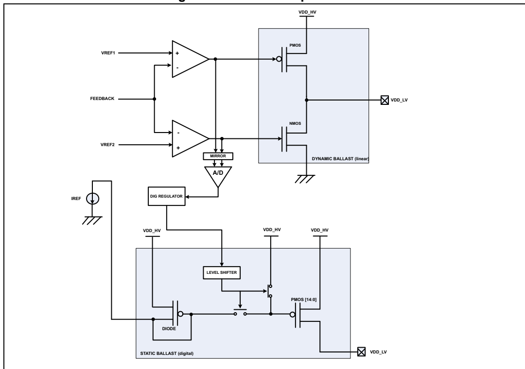
Figure 11. PMU concept scheme
