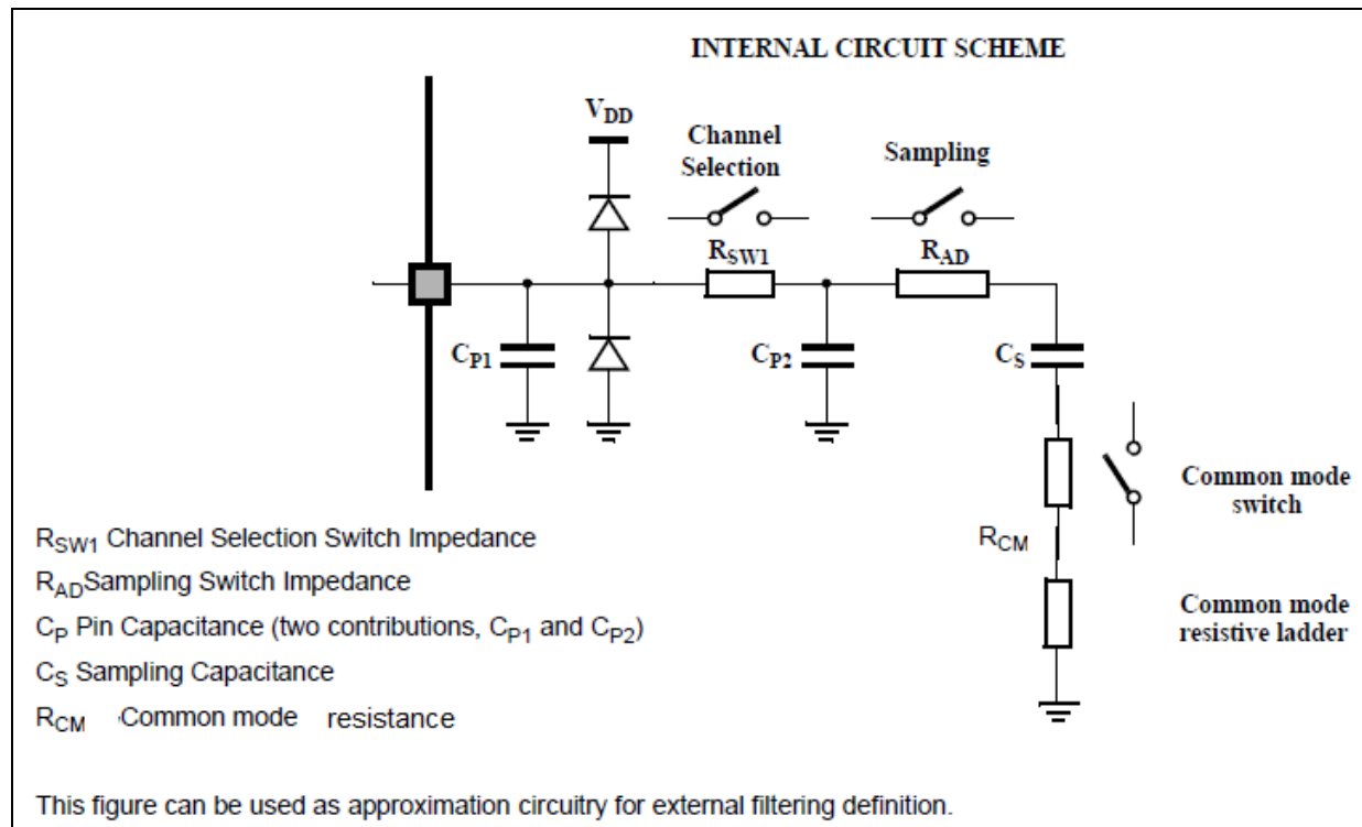
Figure 16. ADC analog input circuit
