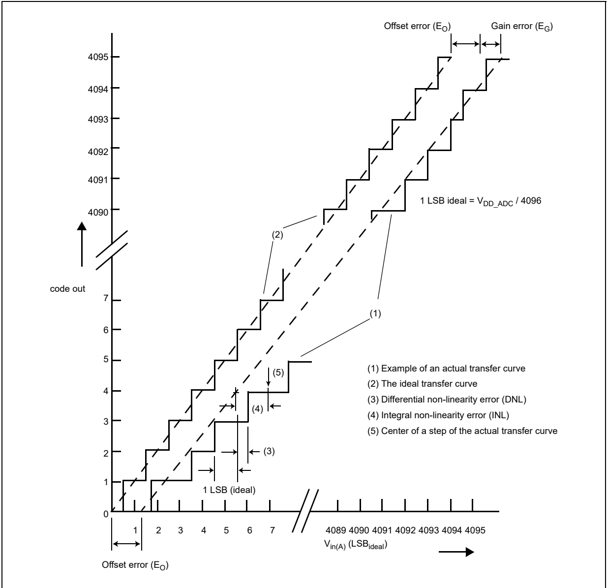
Figure 15. ADC characteristic and error definitions
