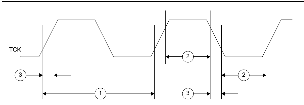
Figure 17. JTAG test clock input timing
