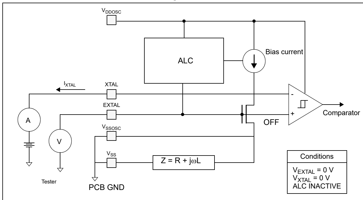
Figure 14. Test circuit
