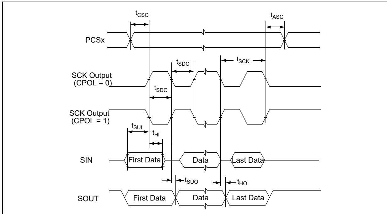
Figure 22. DSPI CMOS master mode – classic timing, CPHA = 0
