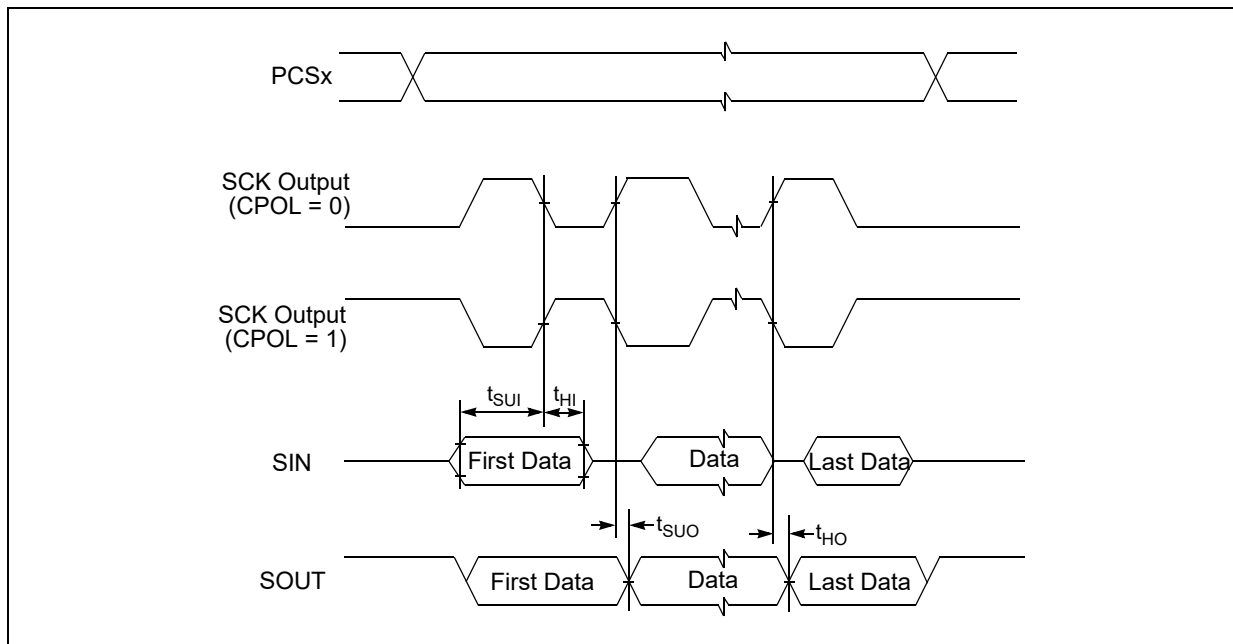
Figure 23. DSPI CMOS master mode – classic timing, CPHA = 1
