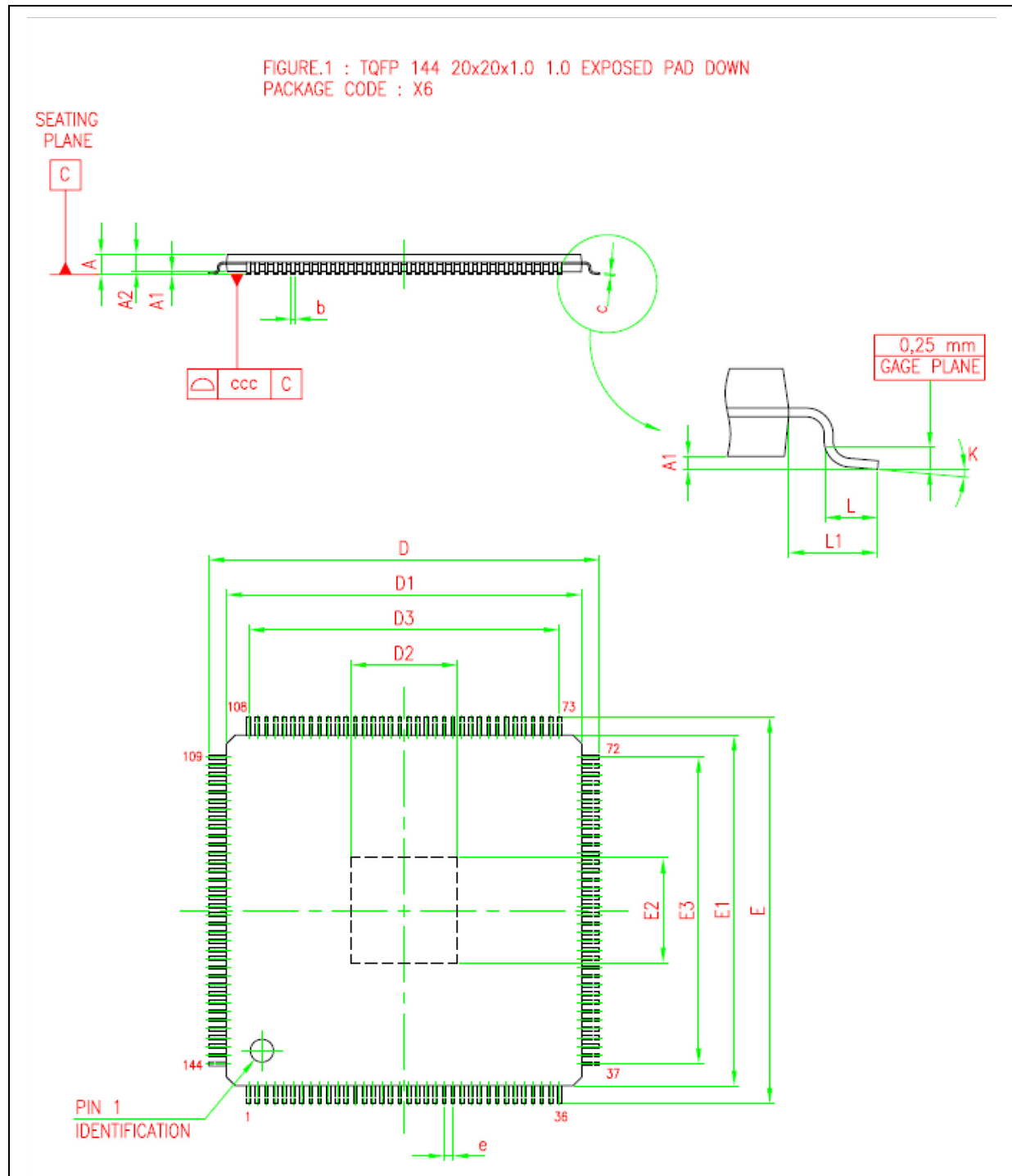
Figure 29. eTQFP144 package outline
