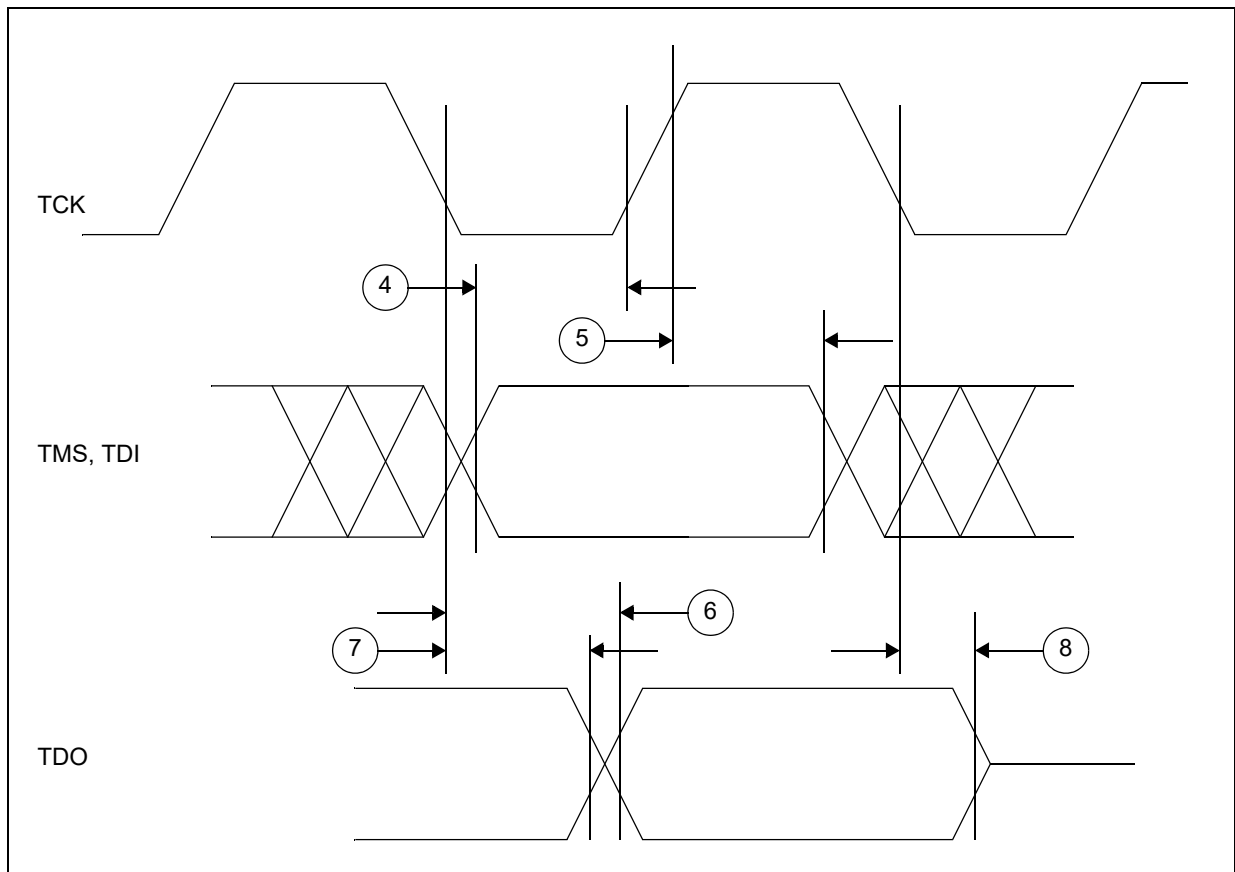
Figure 18. JTAG test access port timing
