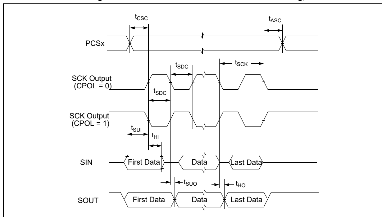
Figure 25. DSPI CMOS master mode – modified timing, CPHA = 0
