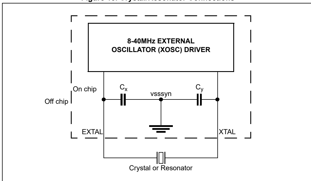
Figure 13. Crystal/Resonator Connections
