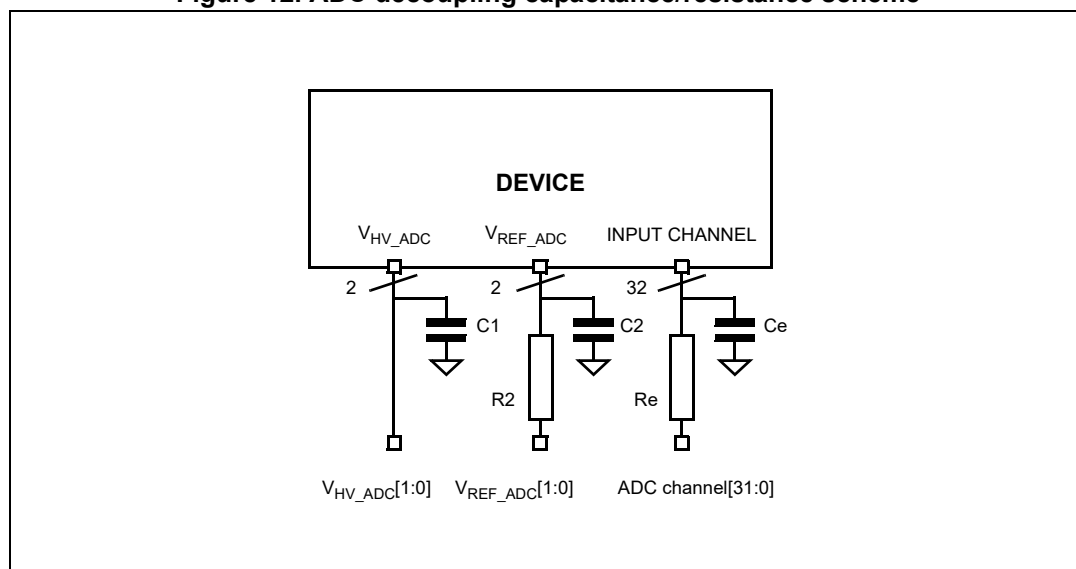
Figure 12. ADC decoupling capacitance/resistance scheme
