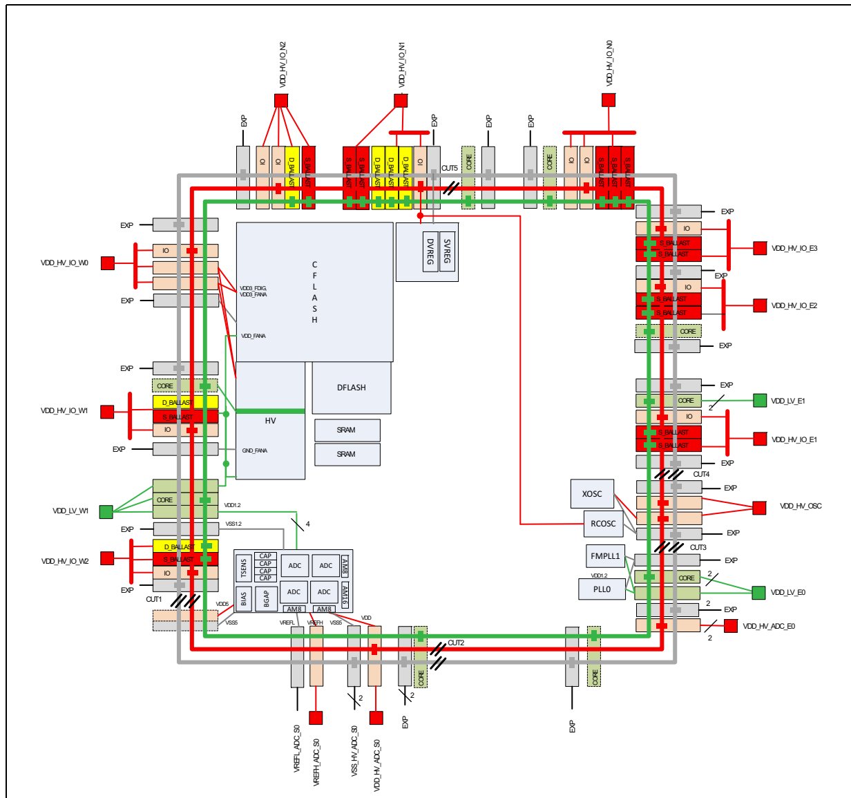
Figure 10. Power supply scheme for eTQFP100
