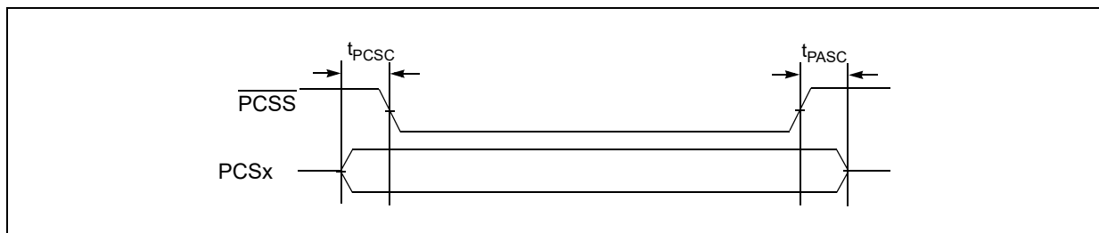
Figure 27. DSPI PCS strobe (PCSS) timing (master mode)
