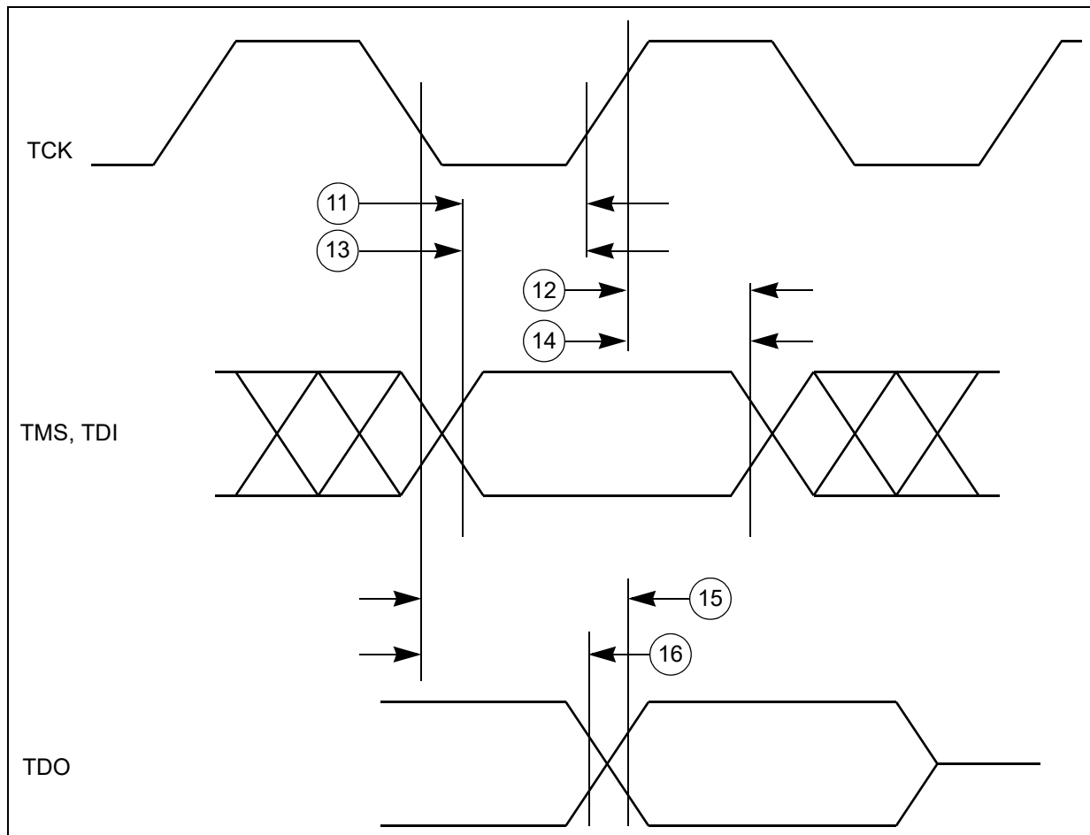
Figure 21. Nexus TDI, TMS, TDO timing
