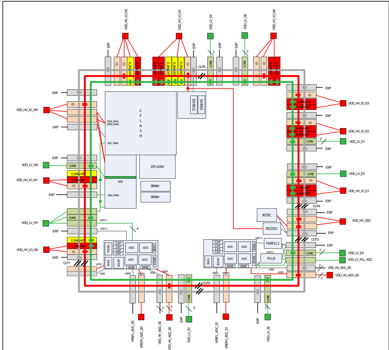
Figure 9. Power supply scheme for eTQFP144
