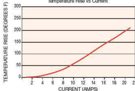
SH-100 High Current Probes Temperature Rise vs Current
