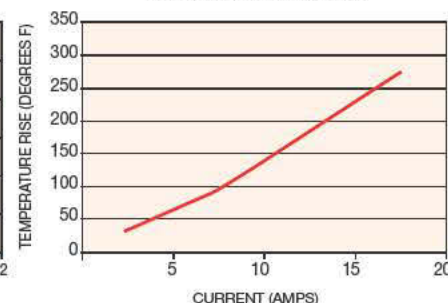
SHE-100 High Current Probes Temperature Rise vs Current
