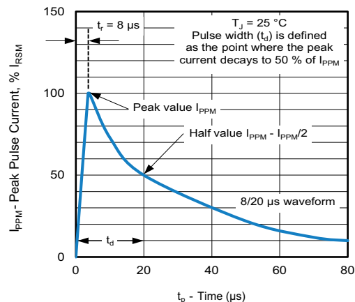
Fig. 4 - Pulse Waveform
