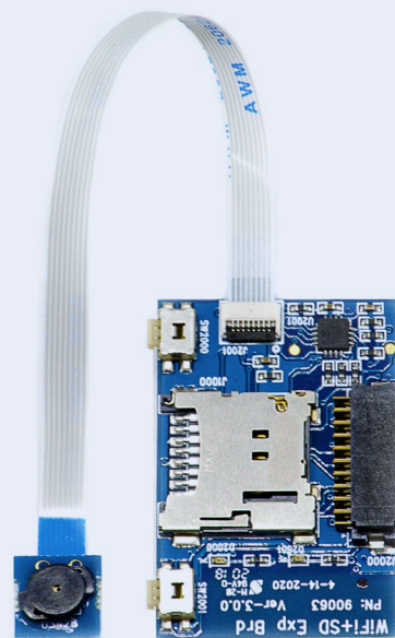
Add-On Board with optional Chirp Ultrasonic Time-of-Flight Sensor
