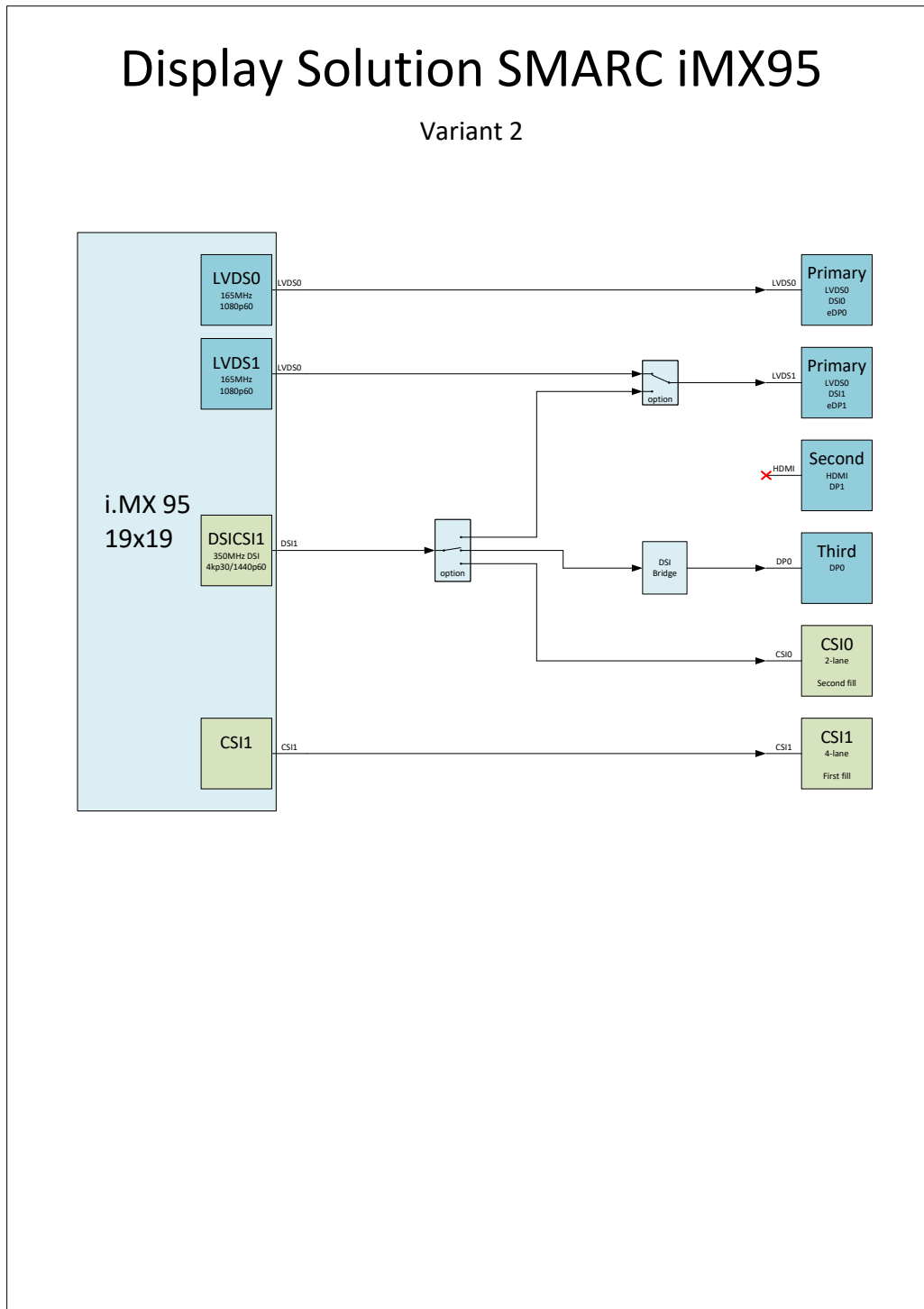
Figure 2: Display Solution Block Diagram - Variant 2
