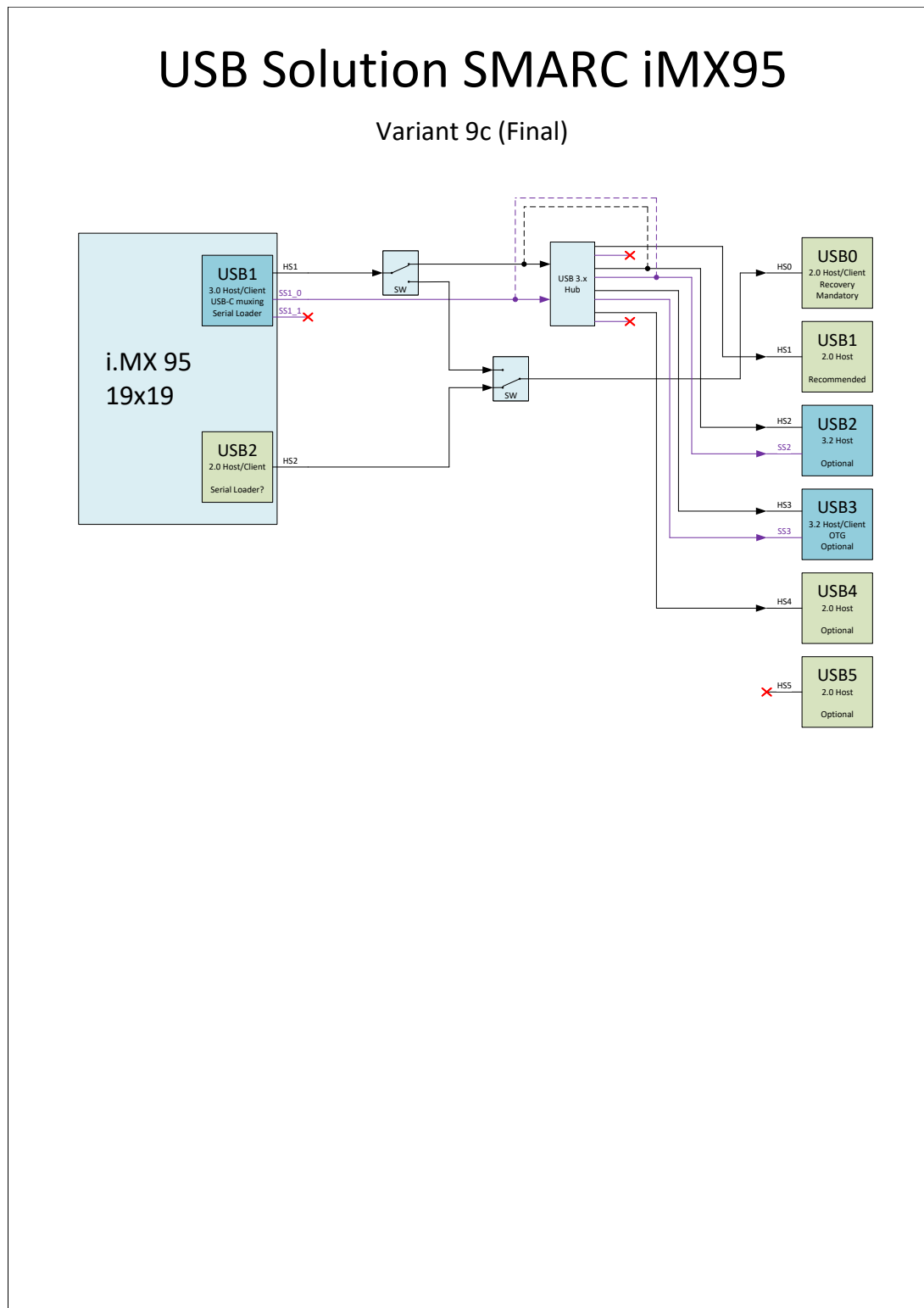
Figure 3: USB Solution Block Diagram
