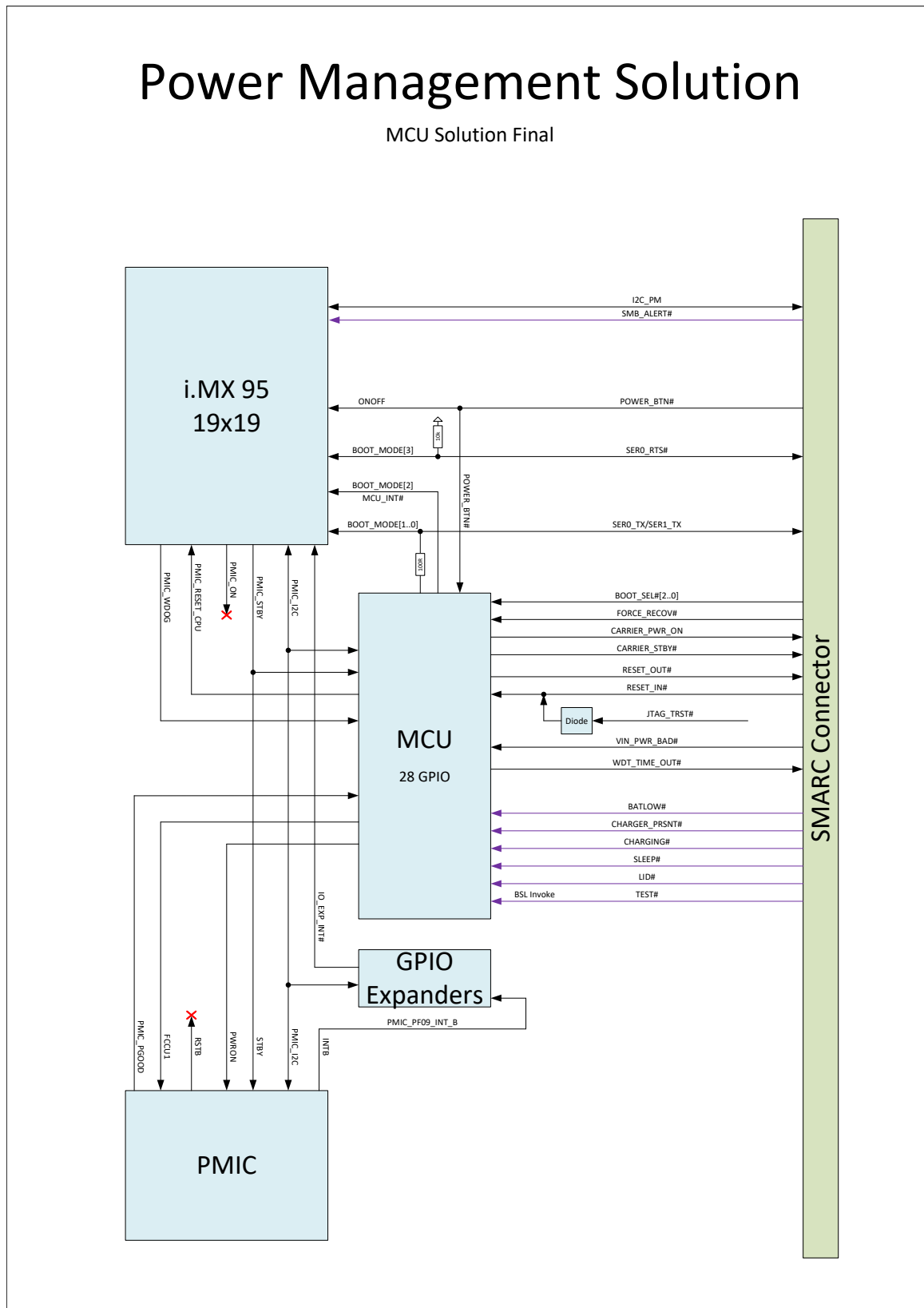
Figure 4: Power Management Solution Block Diagram
