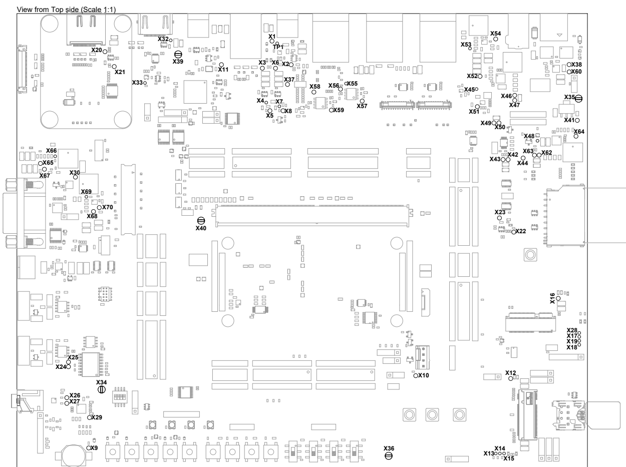
Figure 4: SMARC Development Board Test Points
