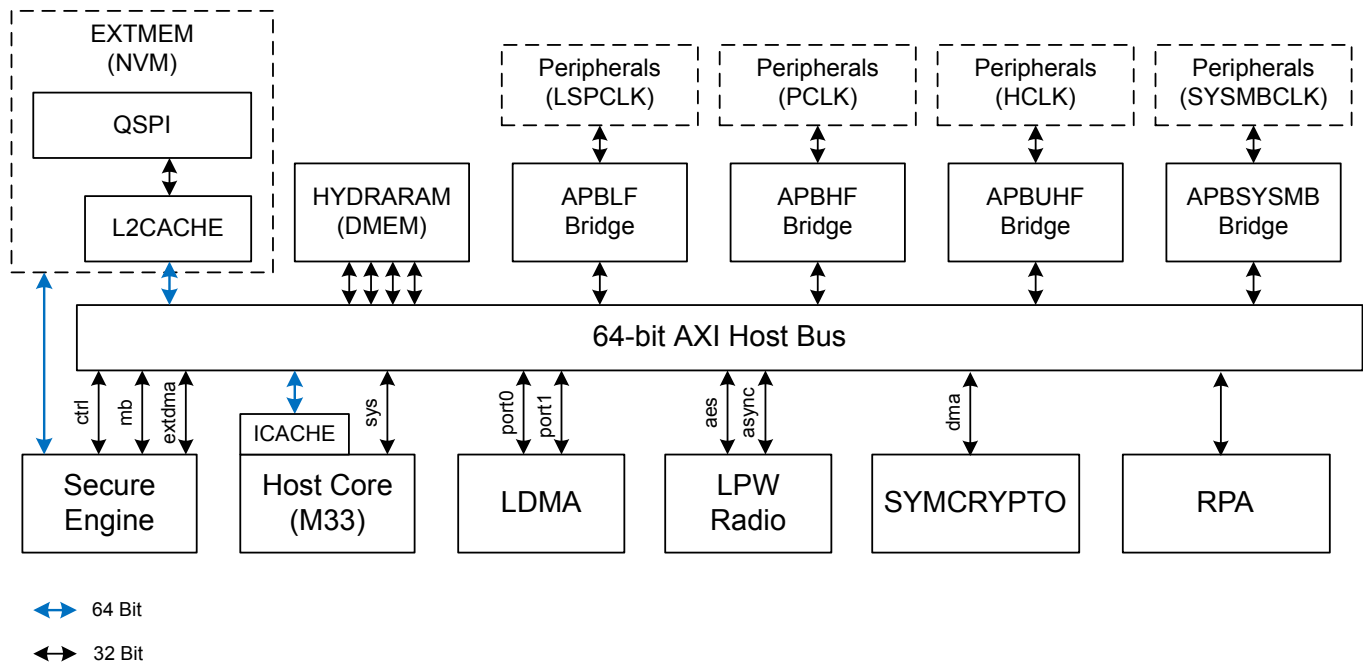
Figure 4.1. SiXG301 Host Bus System
