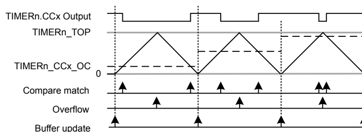
Figure 20.33. TIMER Up/Down-count PWM Generation
