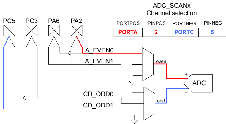
Figure 23.11. Differential Port/Pin Selection Even-Positive, Odd-Negative
