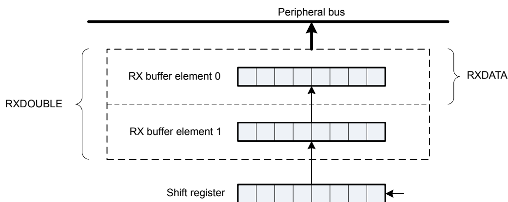
Figure 22.14. I2C Receive Buffer Operation
