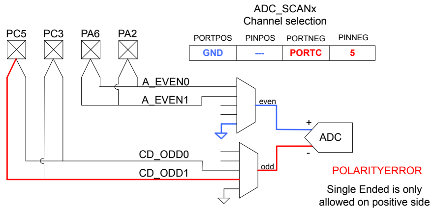
Figure 23.10. Single-Ended Port/Pin Selection Polarity Error
