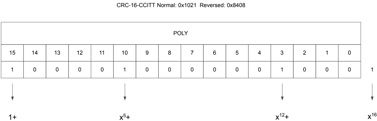
Figure 15.2. Polynomial Representation
