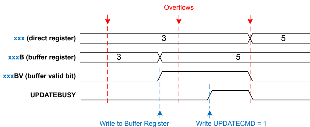
Figure 20.13. TIMER Buffered Output Timing with UPDATEMODE = CMD
