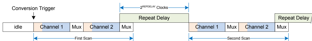
Figure 23.7. Continuous Two-Channel Conversions with Repeat Delay Example
