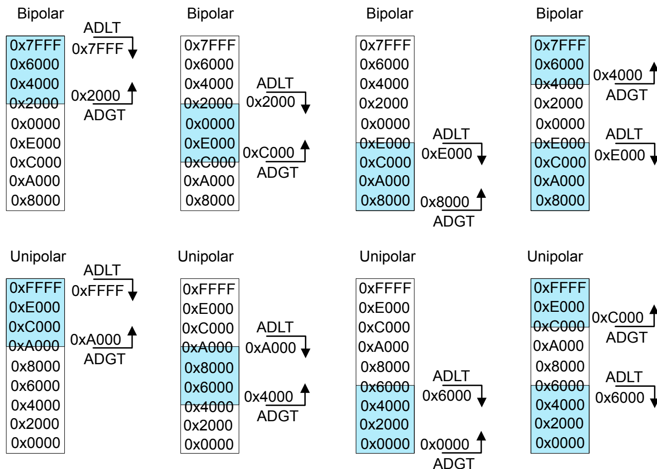
Figure 23.16. Window Comparison Examples
