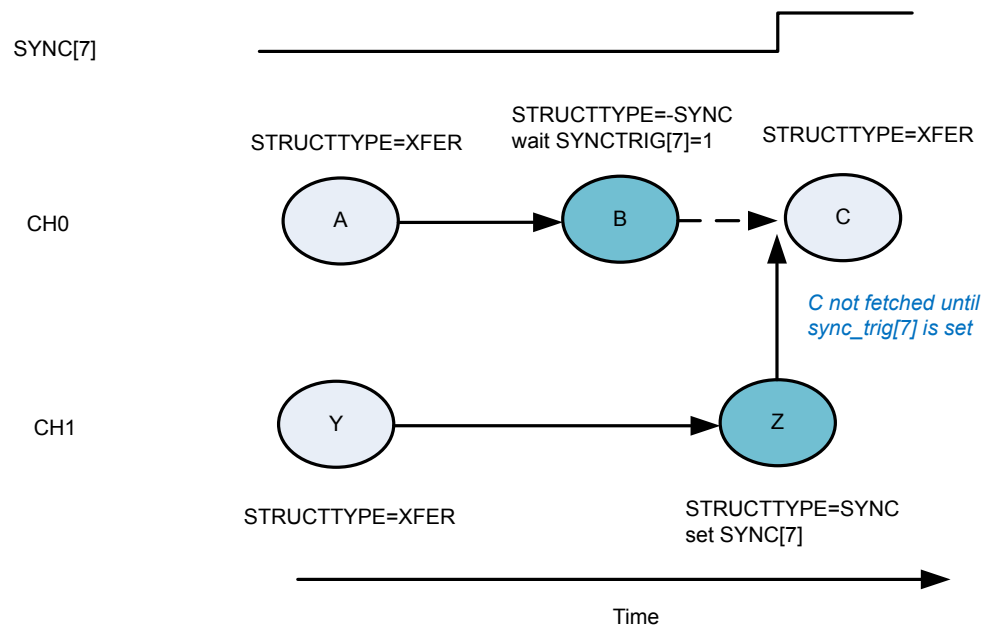
Figure 26.10. Simple Intra-channel Synchronization Example
