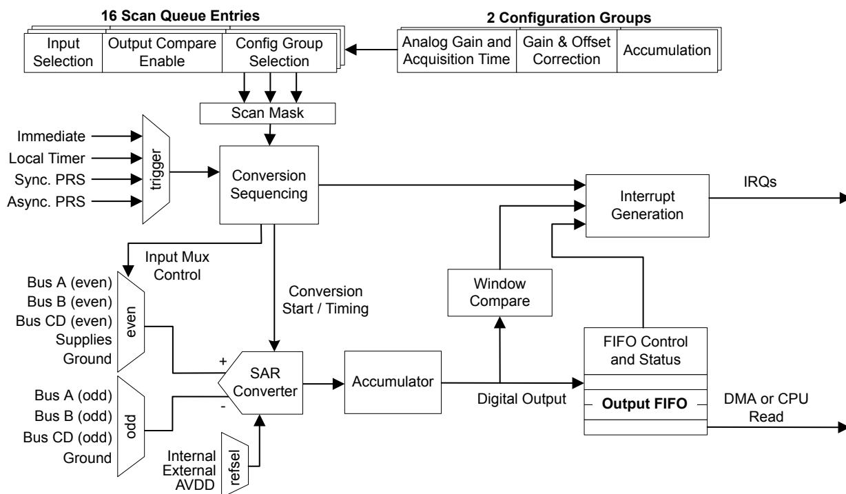
Figure 23.1. ADC Overview
