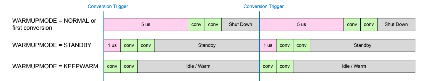
Figure 23.3. Start-up Timing
