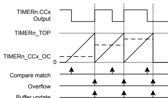
Figure 20.21. TIMER Up-count PWM Generation
