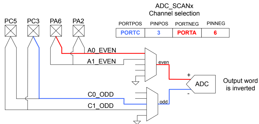
Figure 23.12. Differential Port/Pin Selection Odd-Positive, Even-Negative
