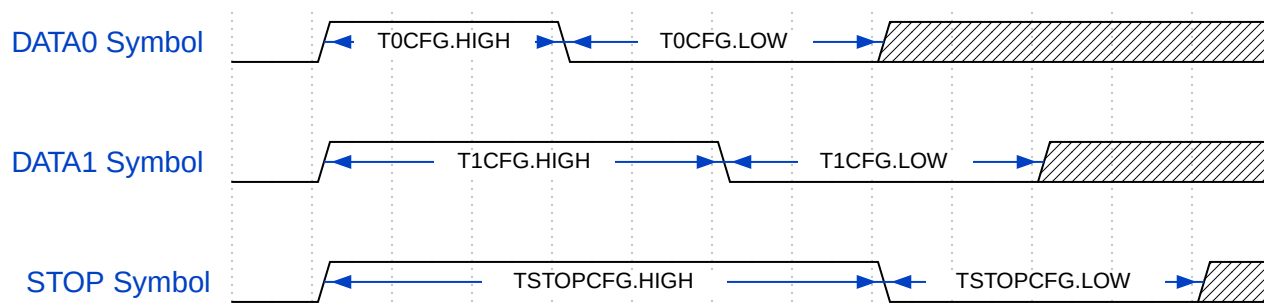
Figure 28.7. Typical Parallel Symbols
