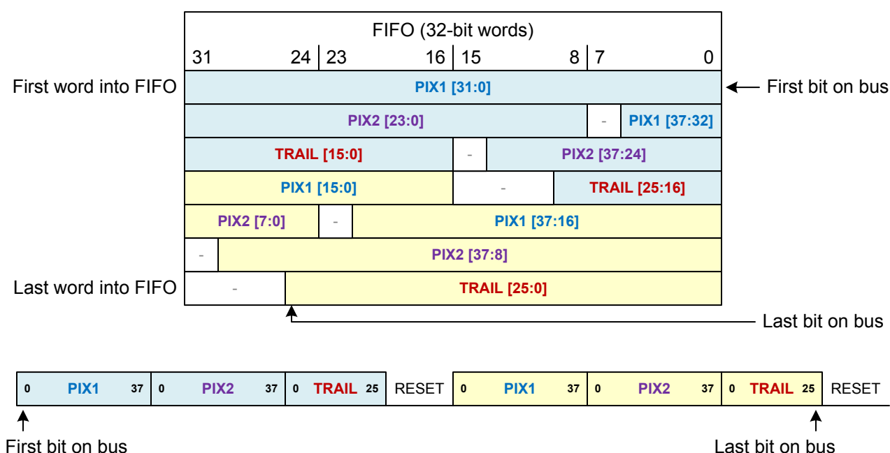
Figure 28.8. LSB-first with 8-bit Memory Alignment
