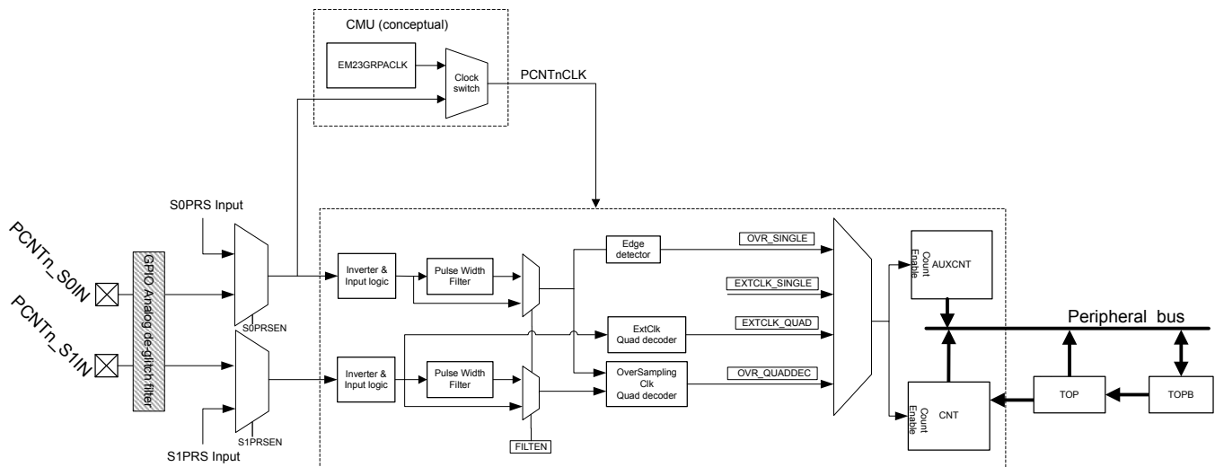
Figure 29.1. PCNT Overview
