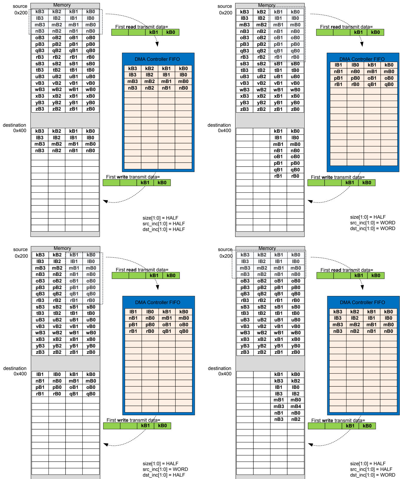
Figure 26.4. Memory-to-Memory Transfer HALF Size Examples
