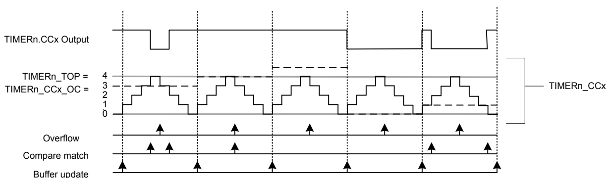
Figure 20.37. TIMER Up/Down-count PWM Generation
