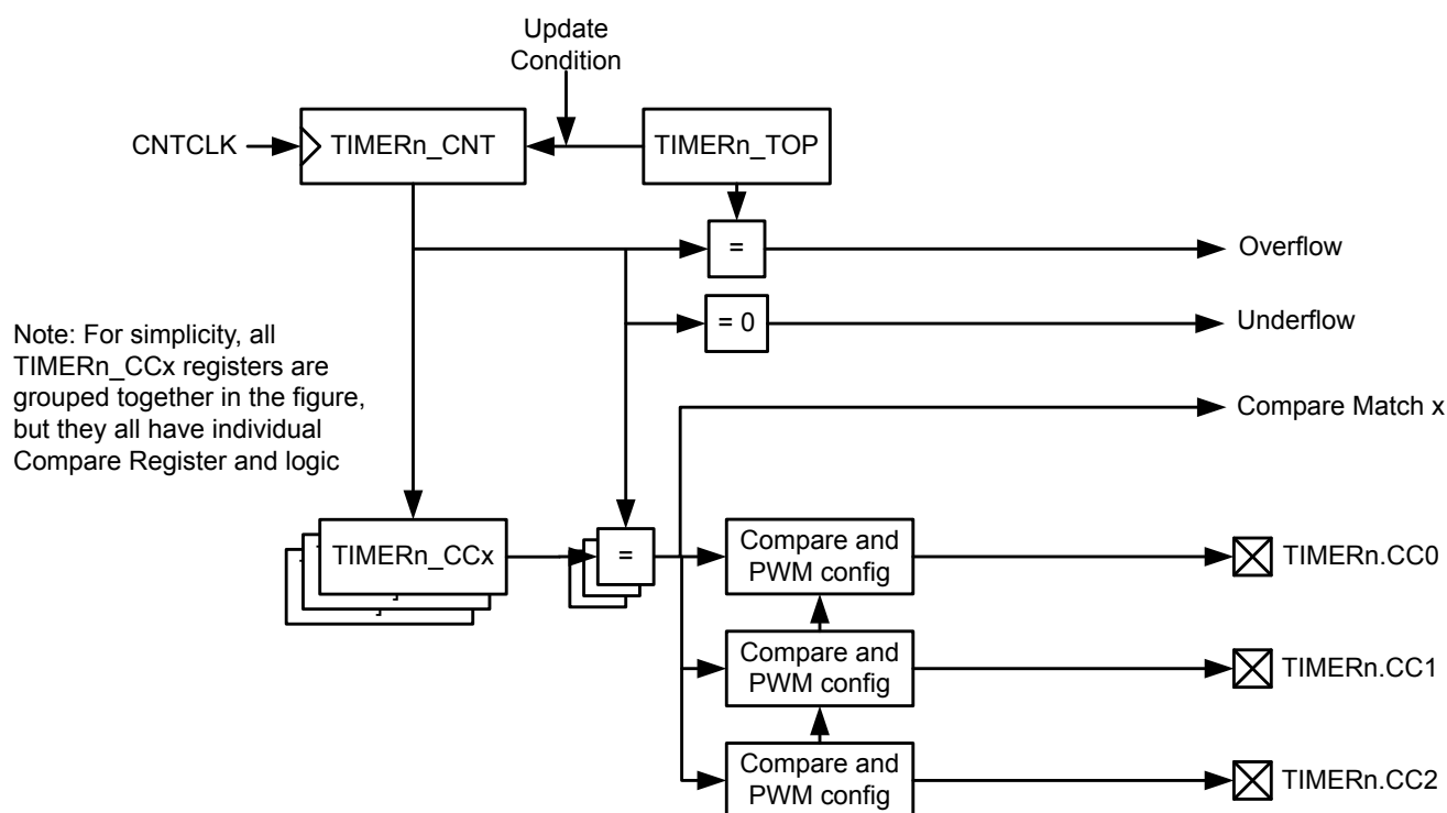
Figure 20.16. TIMER Block Diagram Showing Comparison Functionality
