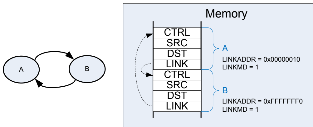
Figure 26.12. Infinite Ping-Pong Example
