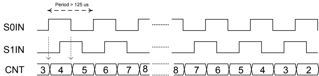
Figure 29.5. PCNT Oversampling Quadrature Decoder 2X Mode
