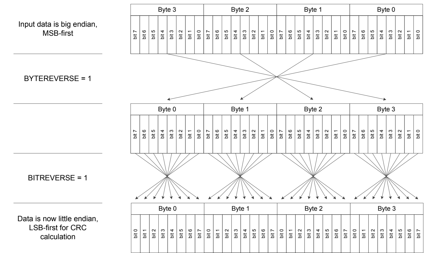
Figure 15.3. Data Ordering Example - 32-bit MSB -first to LSB-first
