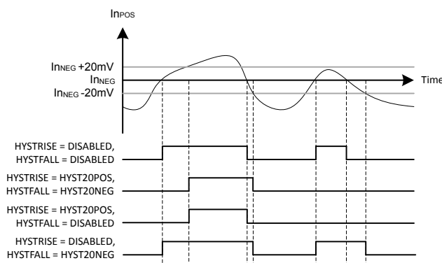
Figure 24.2. Hysteresis
