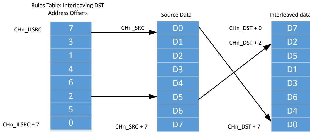
Figure 26.6. Destination Interleaving RELATIVE8 Example
