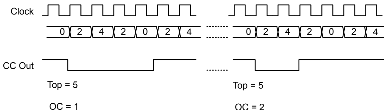
Figure 20.38. TIMER CC Out in 2x Mode
