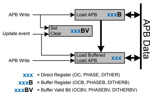
Figure 20.12. TIMER Buffered Output Register Function Detail
