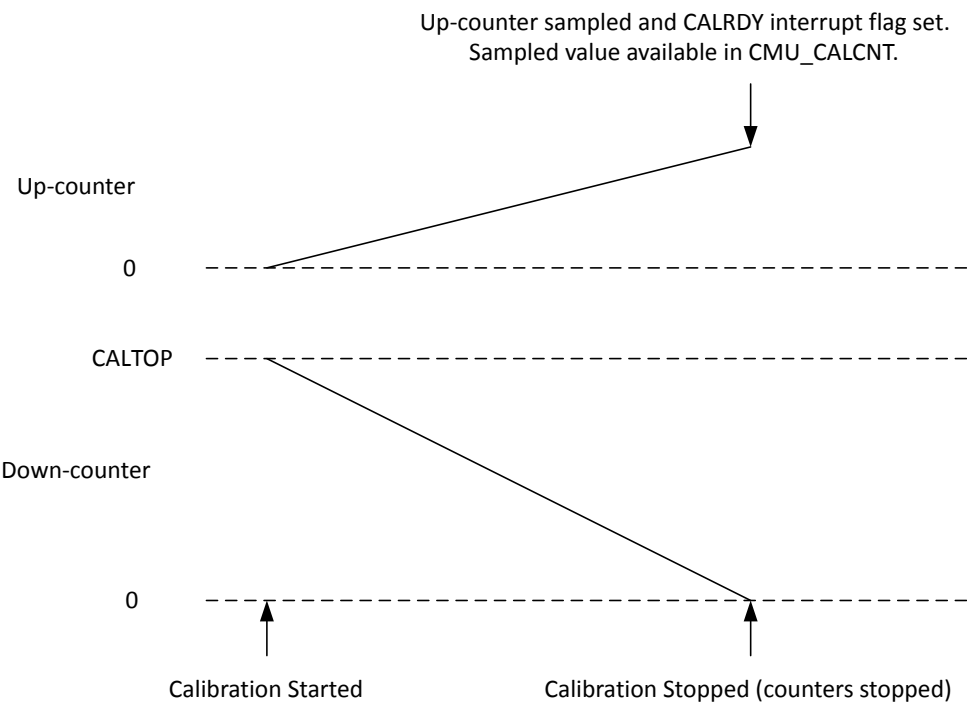
Figure 8.8. Single Calibration (CONT=0)
