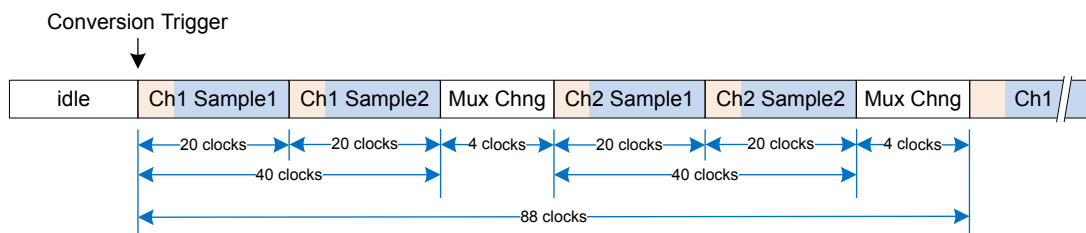
Figure 23.6. Continuous Two-Channel Conversions with Accumulation Example
