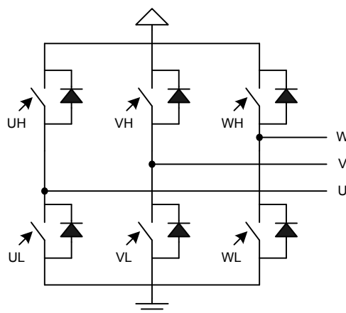
Figure 20.44. TIMER Triple Half-Bridge
