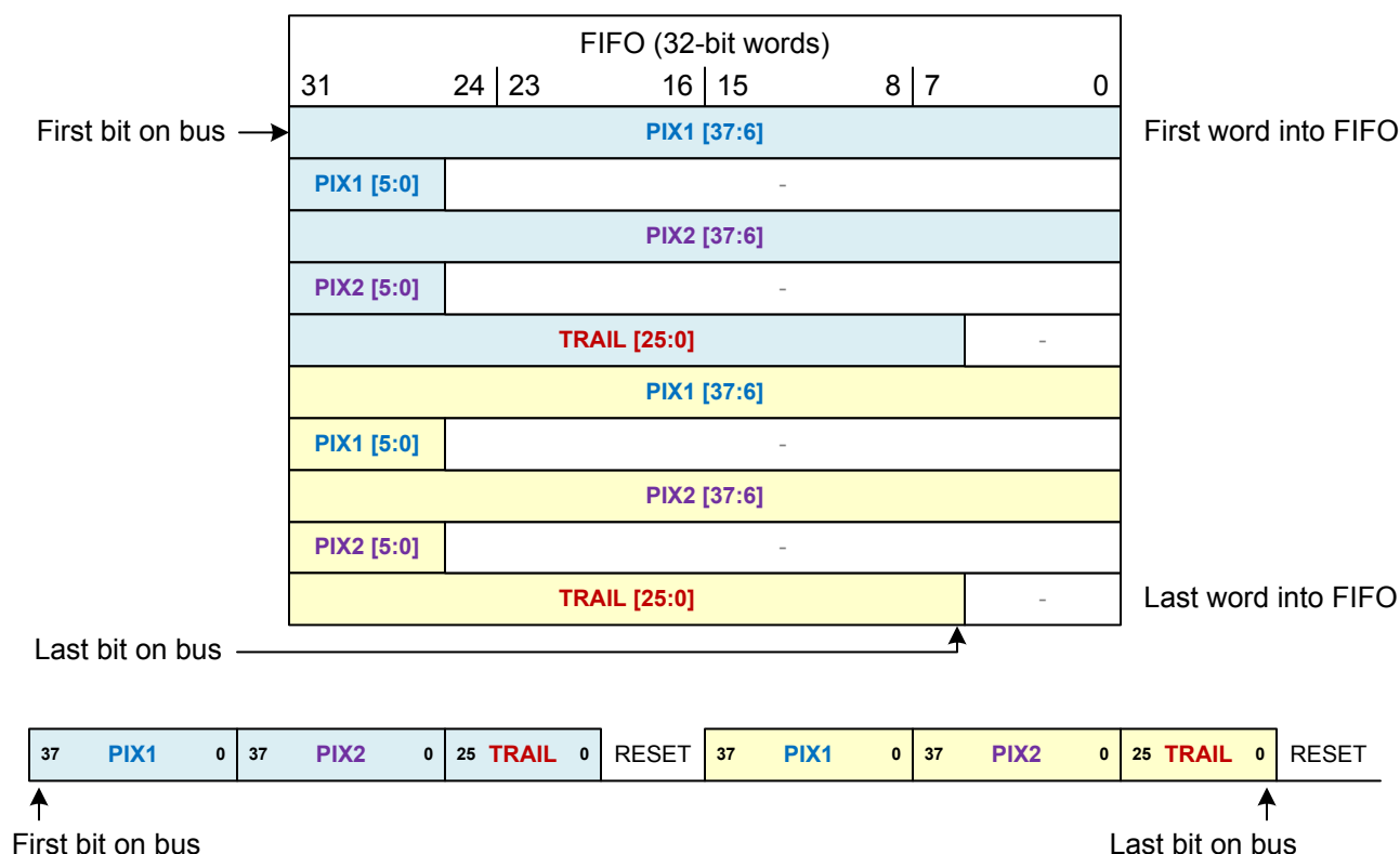
Figure 28.11. MSB-first with 32-bit Memory Alignment
