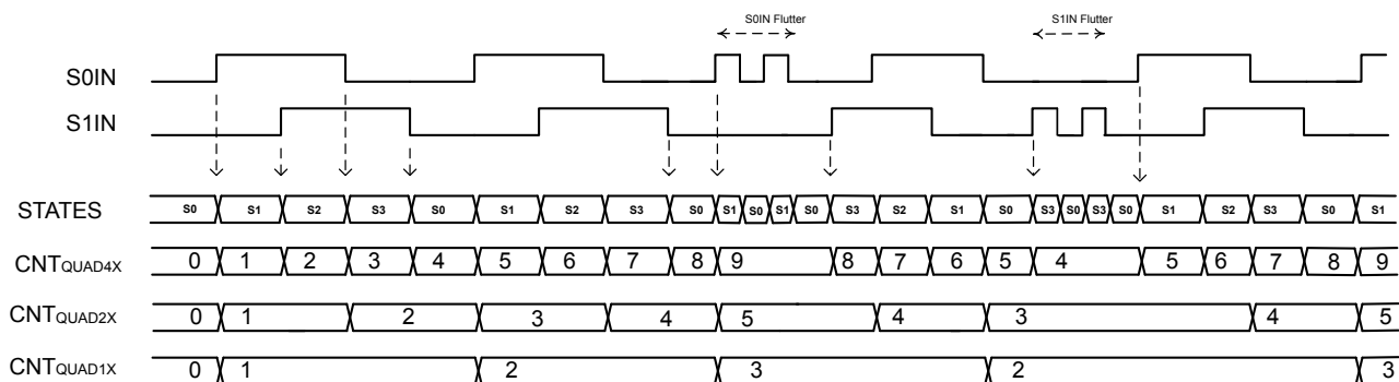
Figure 29.7. PCNT Oversampling Quadrature Decoder with Flutter Removal
