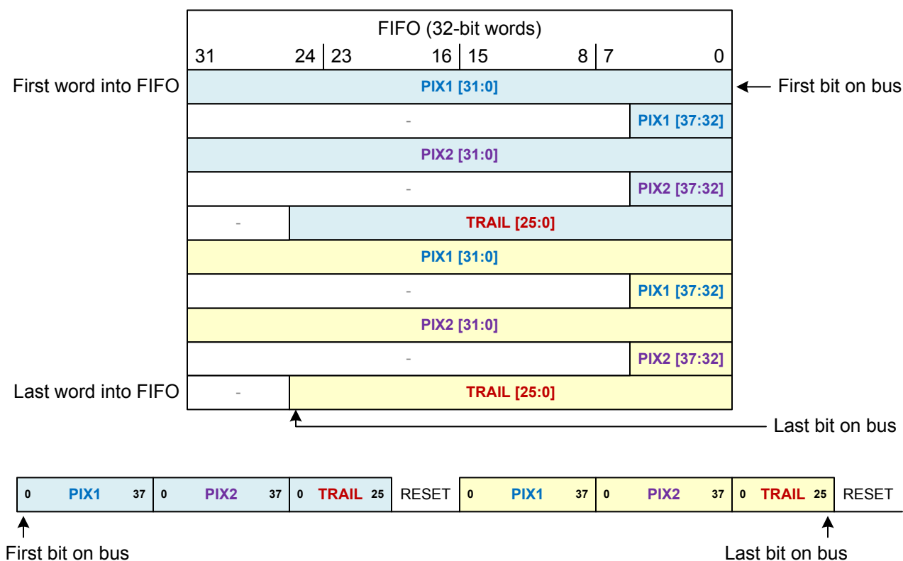
Figure 28.10. LSB-first with 32-bit Memory Alignment
