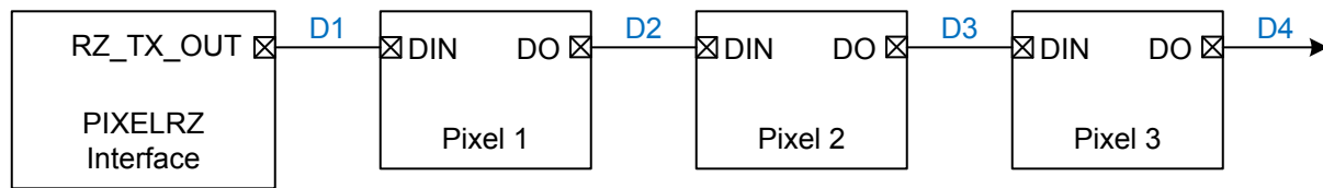
Figure 28.2. Sequential LED Connections
