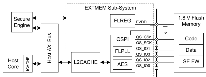
Figure 5.1. EXTMEM Overview
