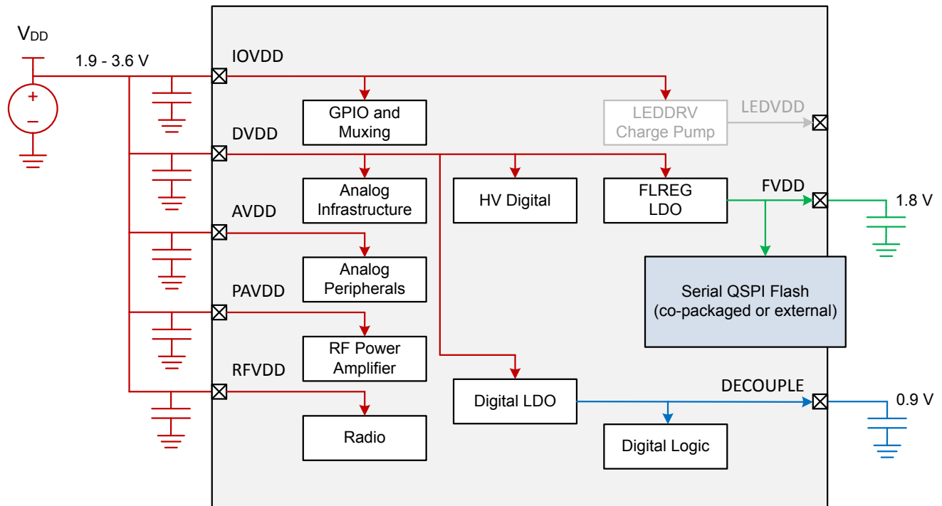
Figure 13.3. Single 1.9 - 3.6 V Supply
