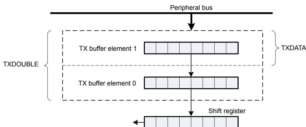
Figure 22.13. I2C Transmit Buffer Operation
