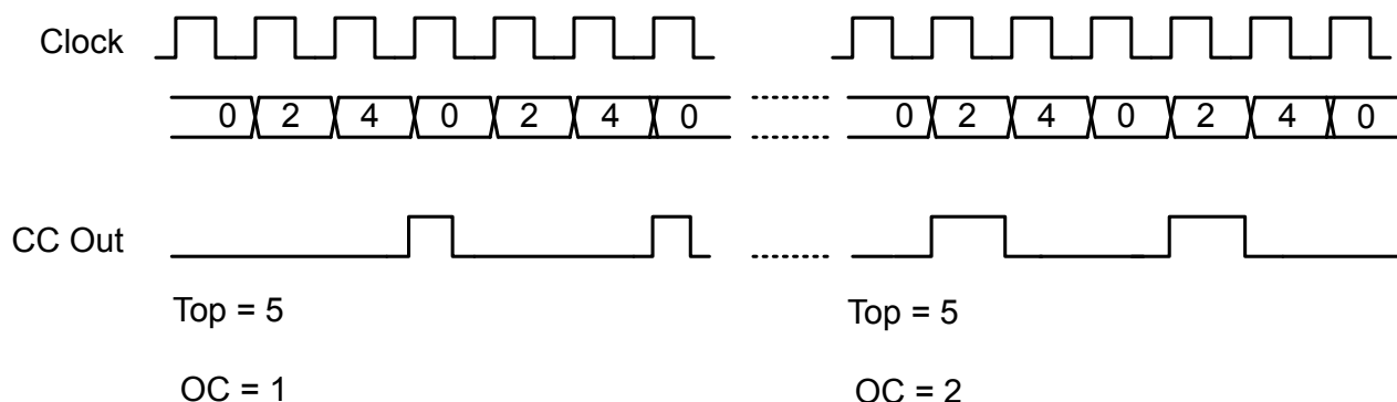
Figure 20.29. TIMER CC Out in 2x Mode
