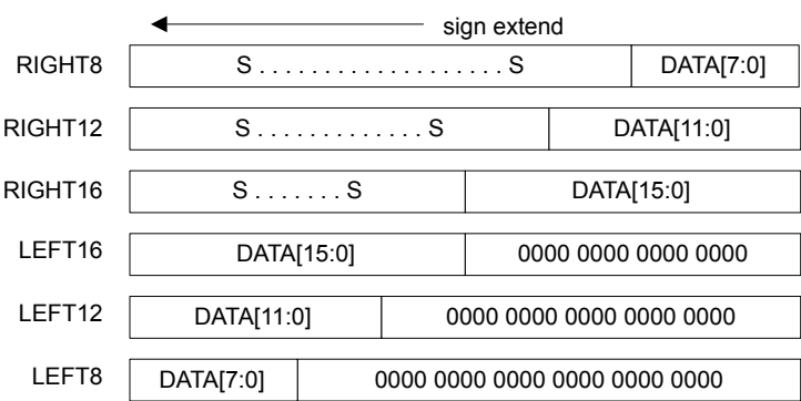
Figure 23.14. Data Alignment
