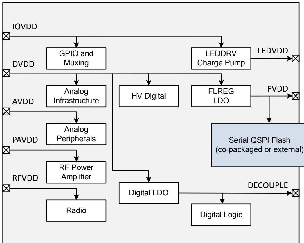
Figure 13.1. Power Distribution
