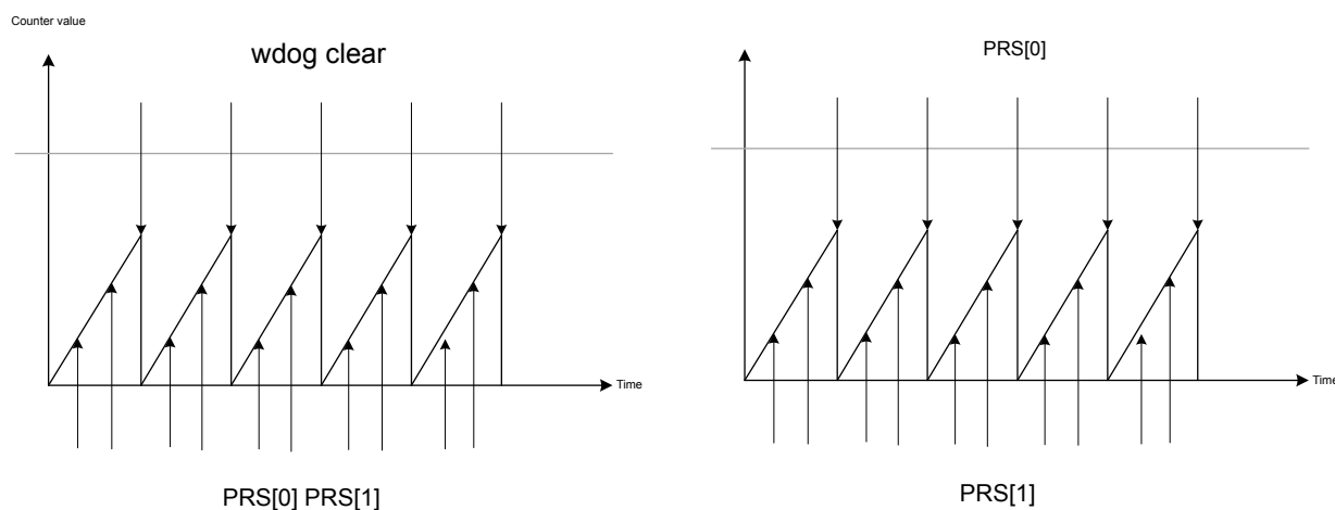
Figure 30.3. PRS Edge Monitoring in WDOG
