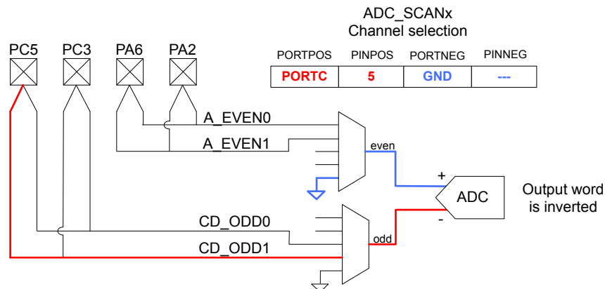
Figure 23.9. Single-Ended Port/Pin Selection Odd Channel
