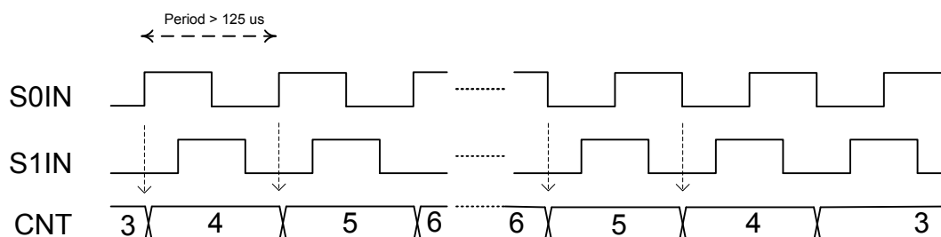
Figure 29.4. PCNT Oversampling Quadrature Decoder 1X Mode
