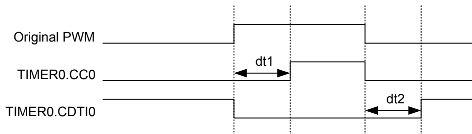
Figure 20.46. TIMER Polarity of Both Signals are Set as Active-High
