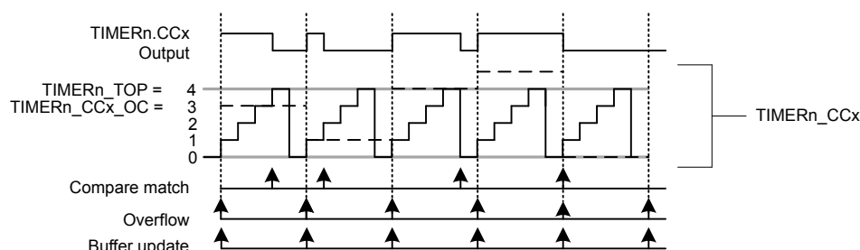
Figure 20.25. TIMER Up-count PWM Generation Detail
