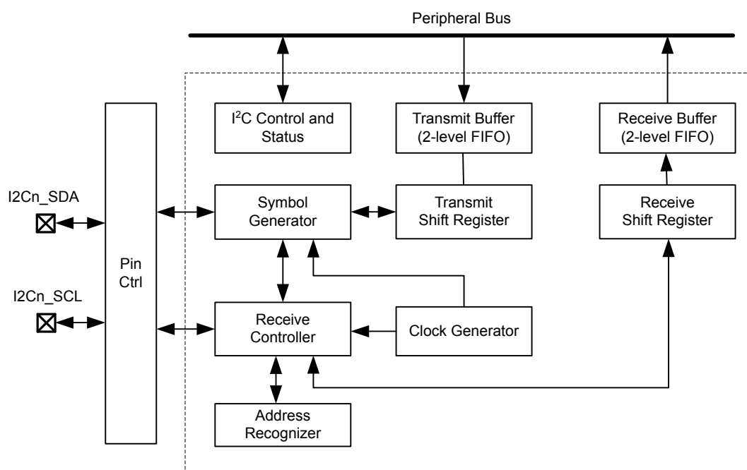
Figure 22.1. I2C Overview
