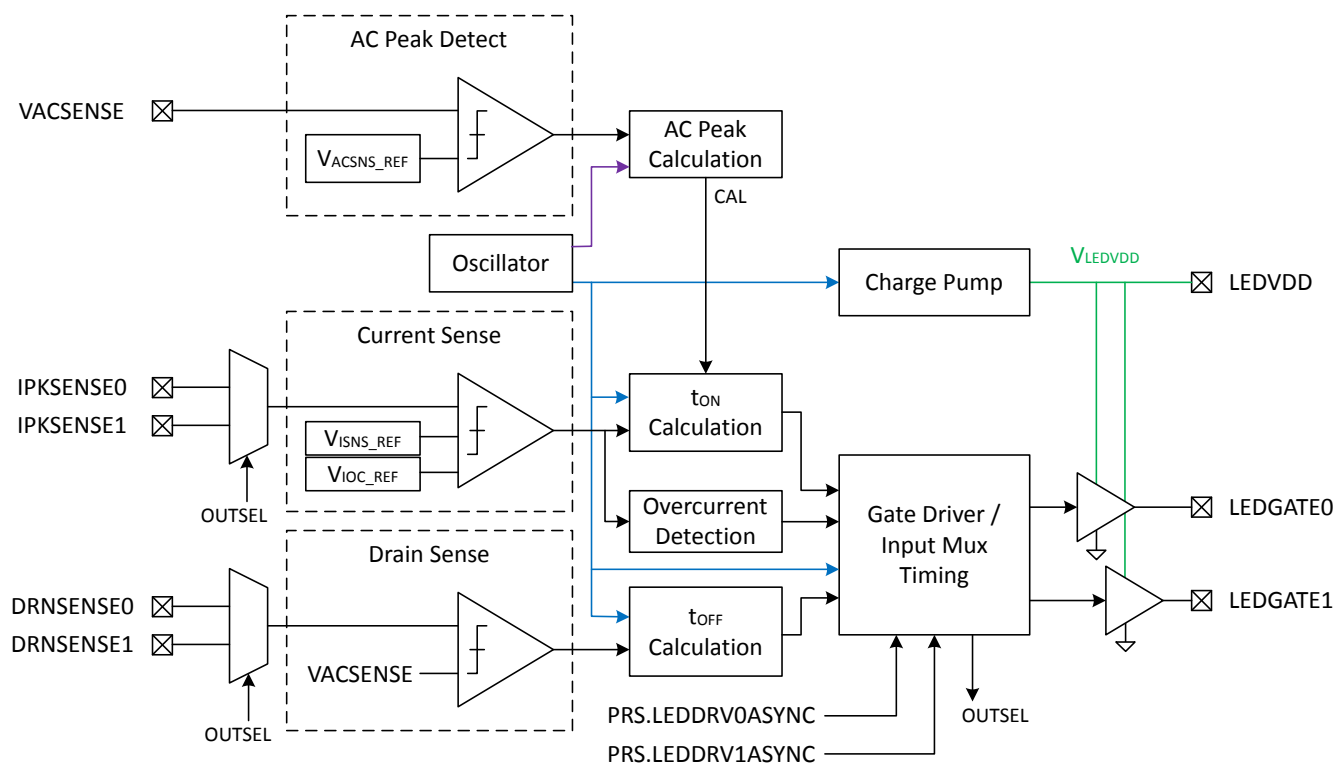
Figure 27.1. LEDDRV Overview
