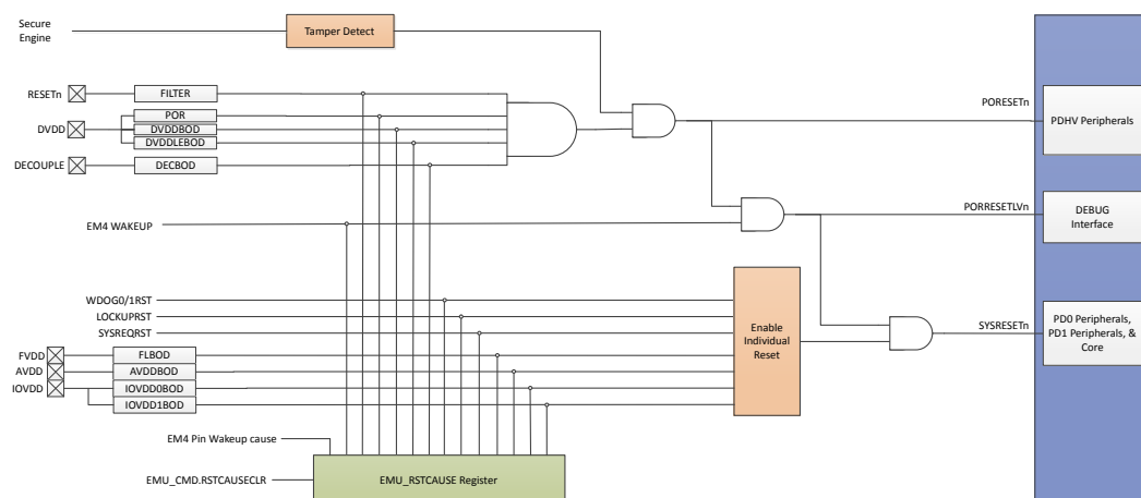
Figure 13.5. Reset Tree
