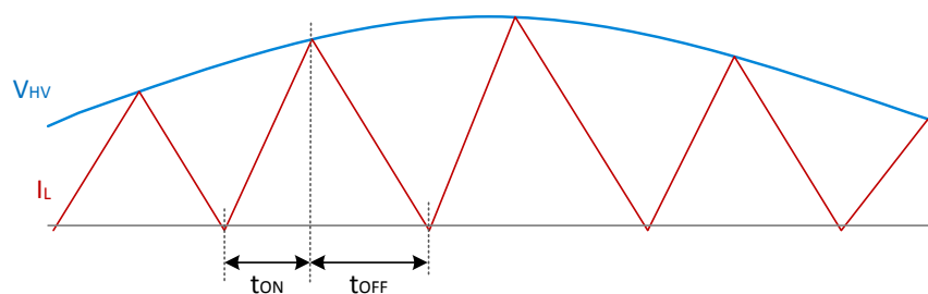
Figure 27.3. Inductor Current
