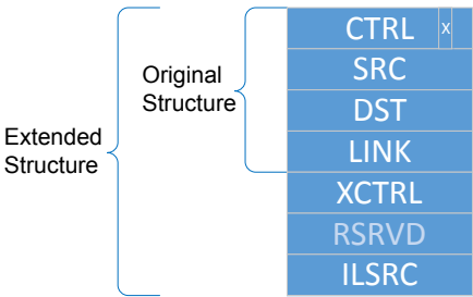
Figure 26.5. Struct and extended struct
