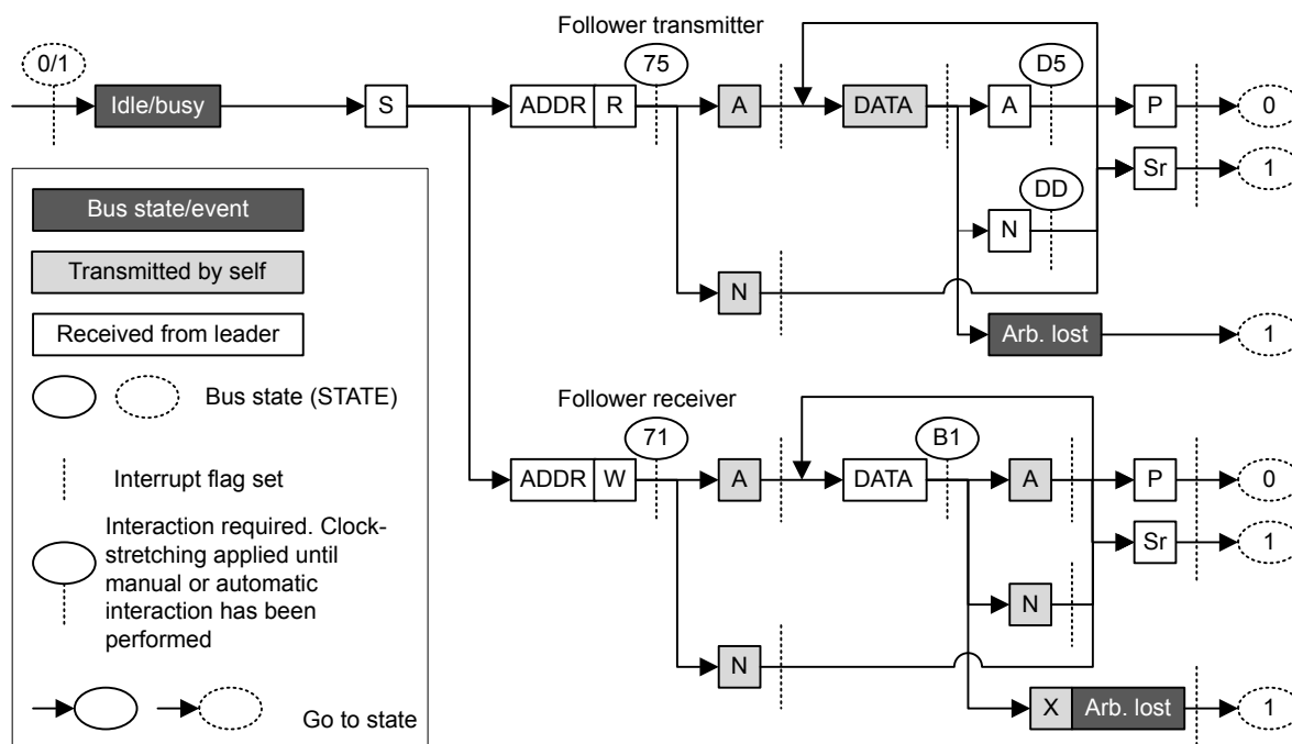
Figure 22.16. I2C Follower State Machine
