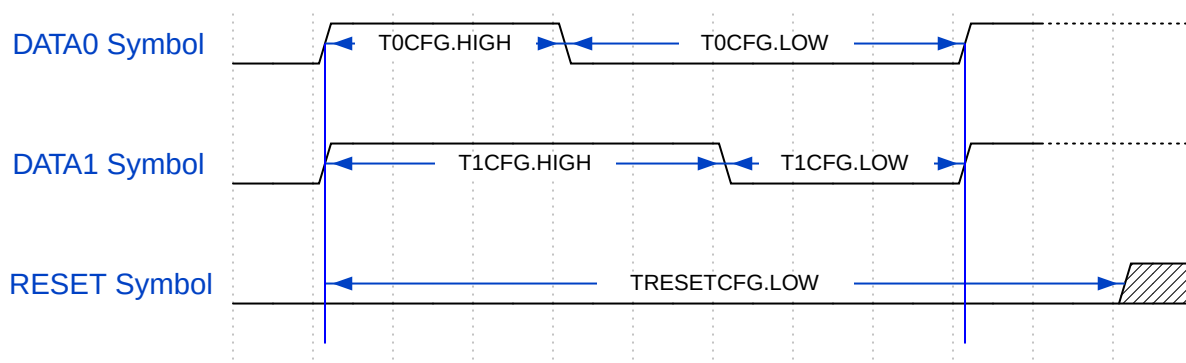
Figure 28.4. Typical Sequential Symbols
