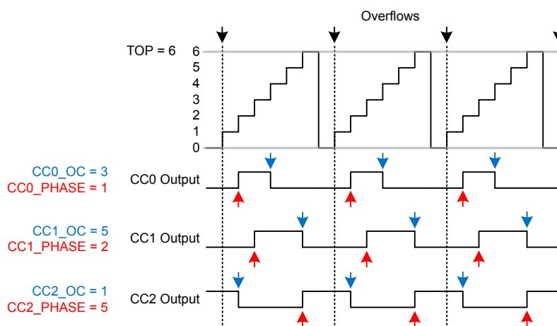
Figure 20.27. Phase Adjustment Example
