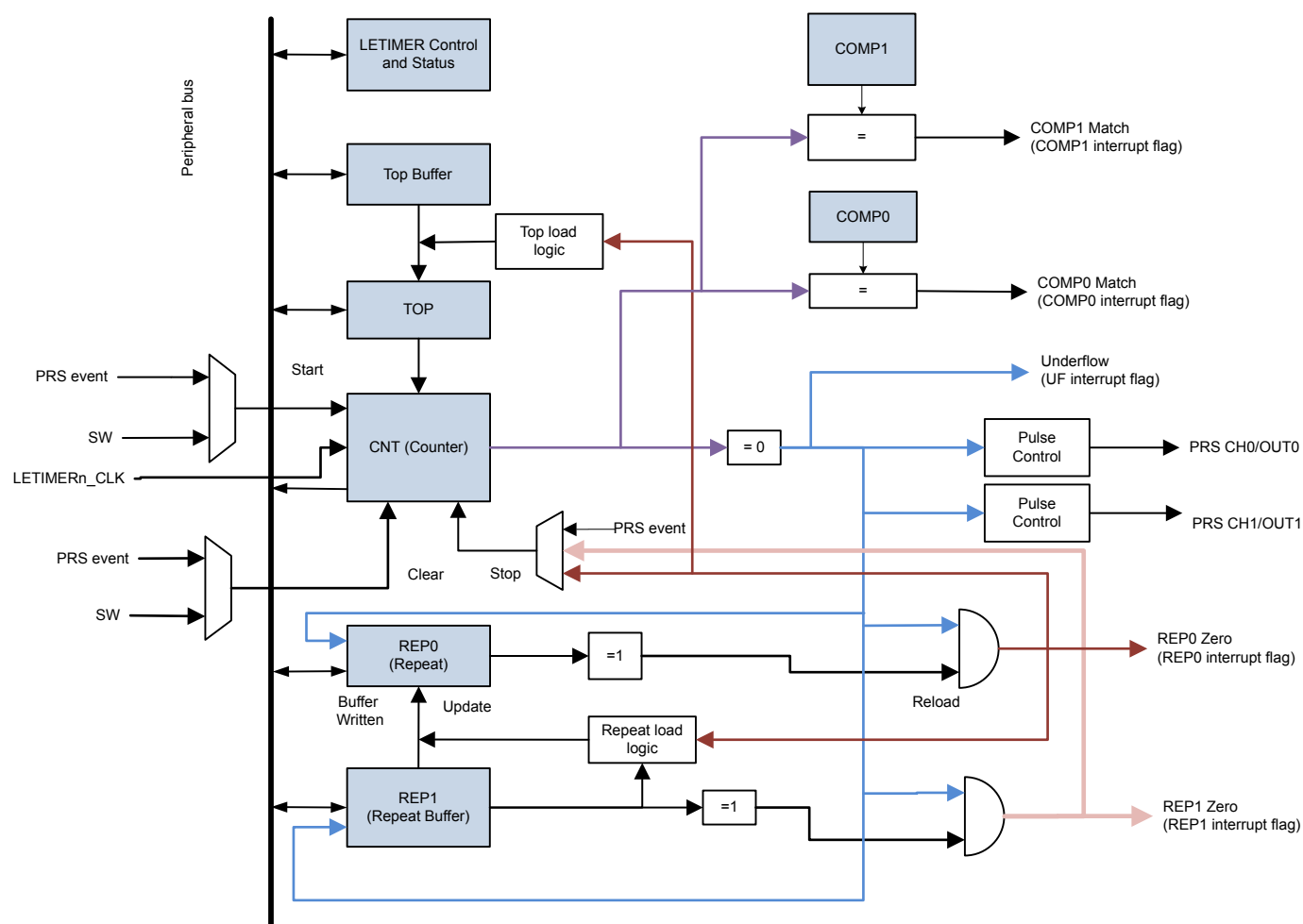
Figure 19.1. LETIMER Overview
