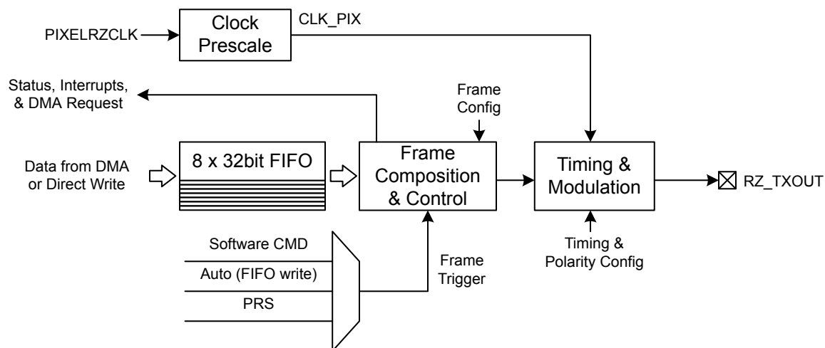
Figure 28.1. PIXELRZ Block Diagram
