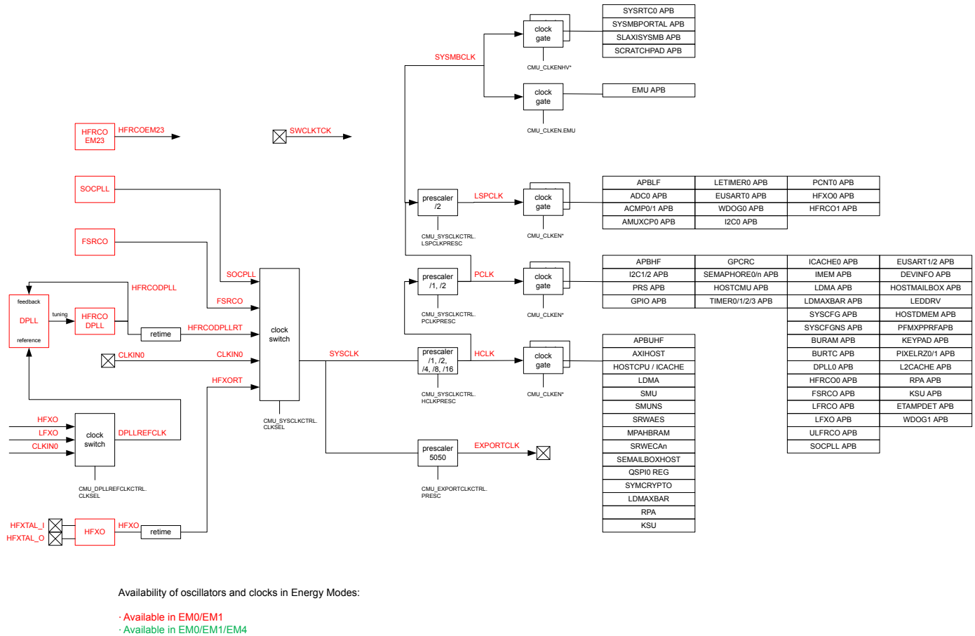
Figure 8.1. Bus Clocks
