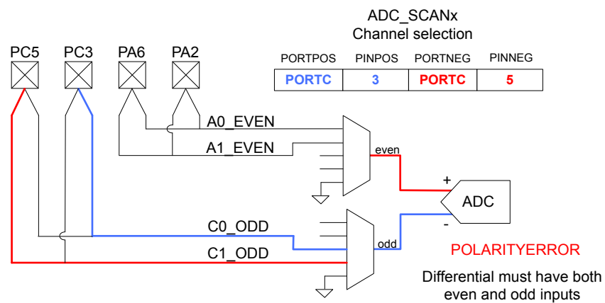
Figure 23.13. Differential Port/Pin Selection Polarity Error
