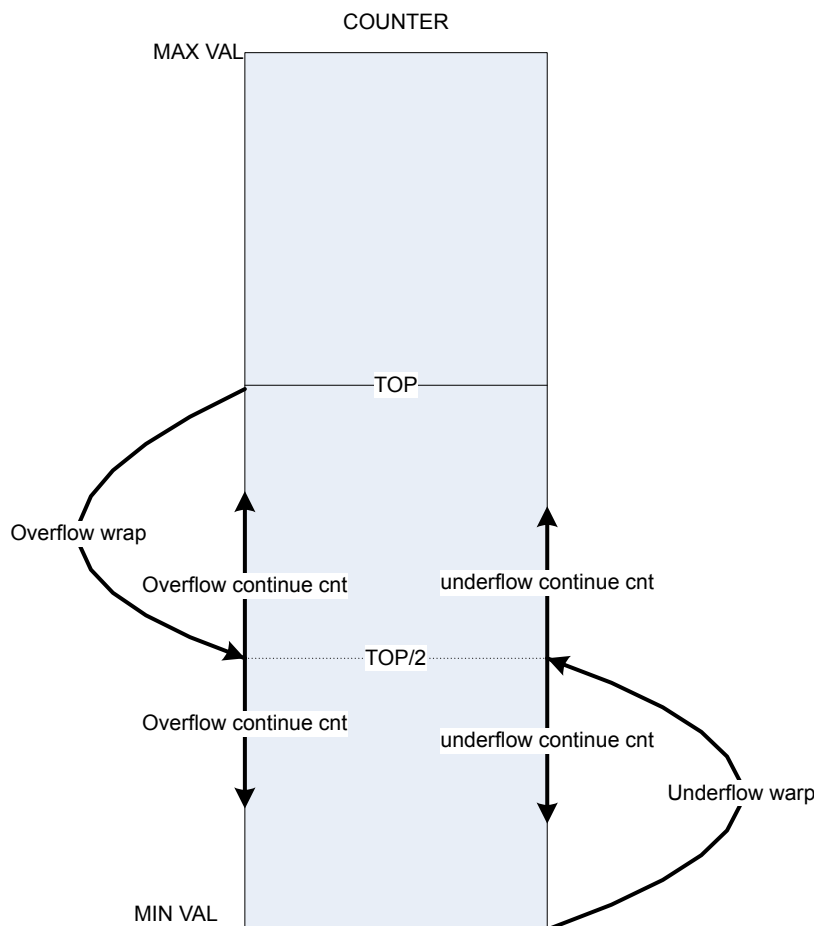
Figure 29.8. PCNT Hysteresis Behavior of Counter
