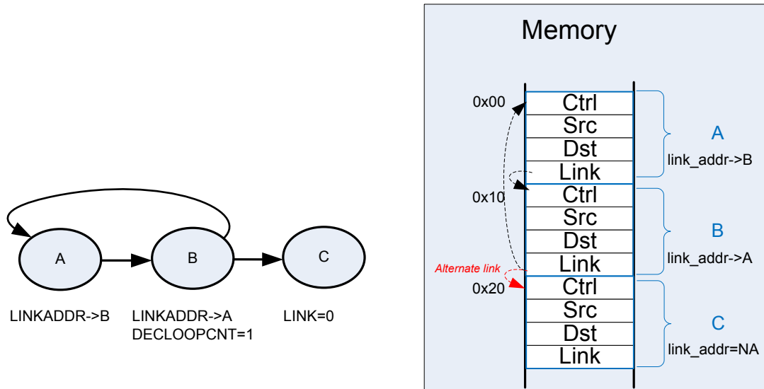
Figure 26.9. Descriptor List with Looping
