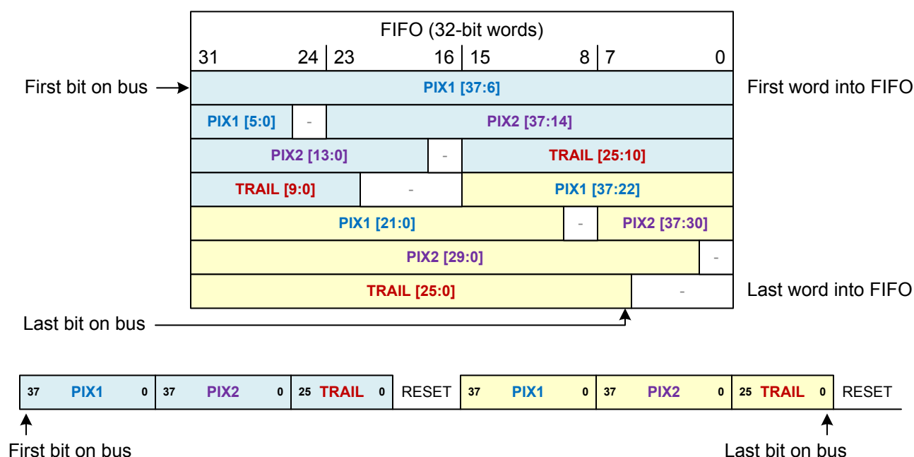
Figure 28.9. MSB-first with 8-bit Memory Alignment
