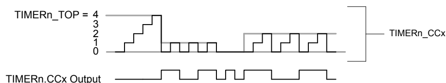
Figure 20.20. TIMER Up-count Frequency Generation Detail
