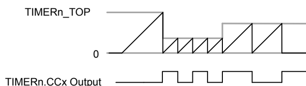
Figure 20.18. TIMER Up-count Frequency Generation
