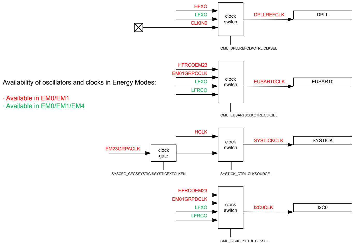
Figure 8.4. Mixed-Frequency Peripheral Clocks
