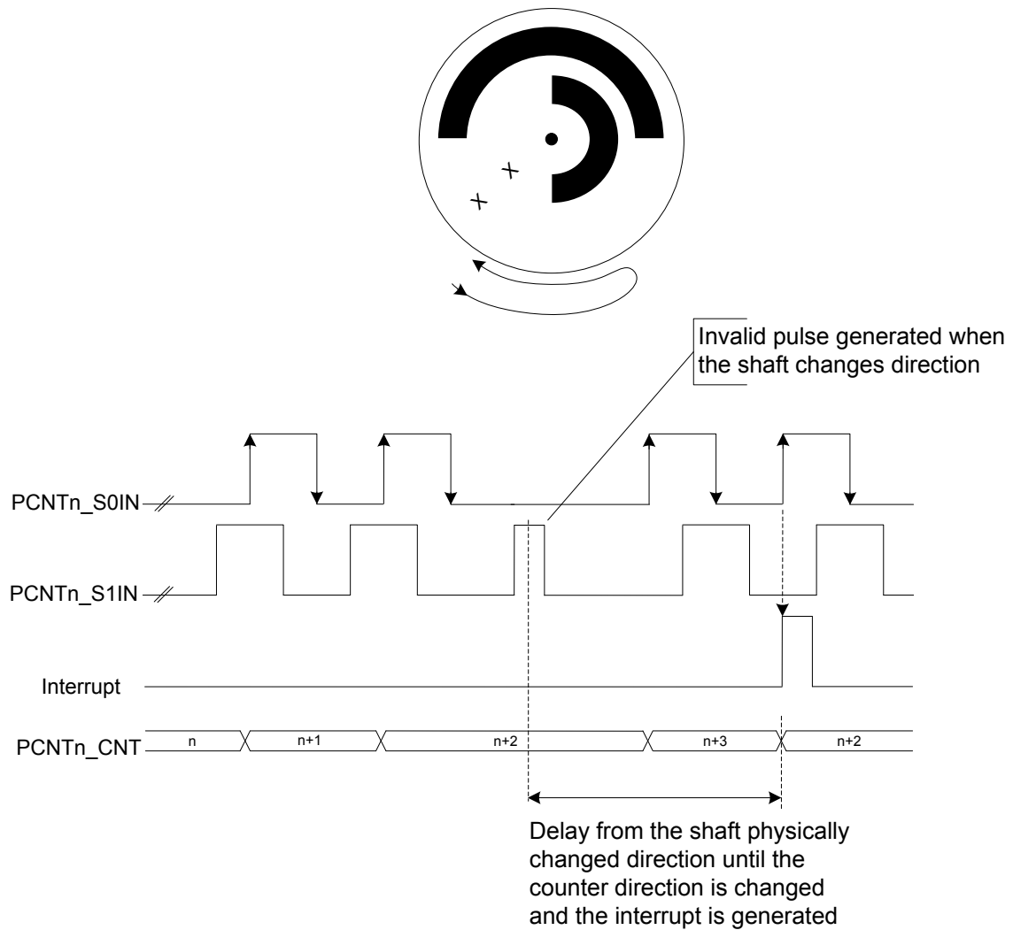
Figure 29.12. PCNT Direction Change Interrupt (DIRCNG) Generation
