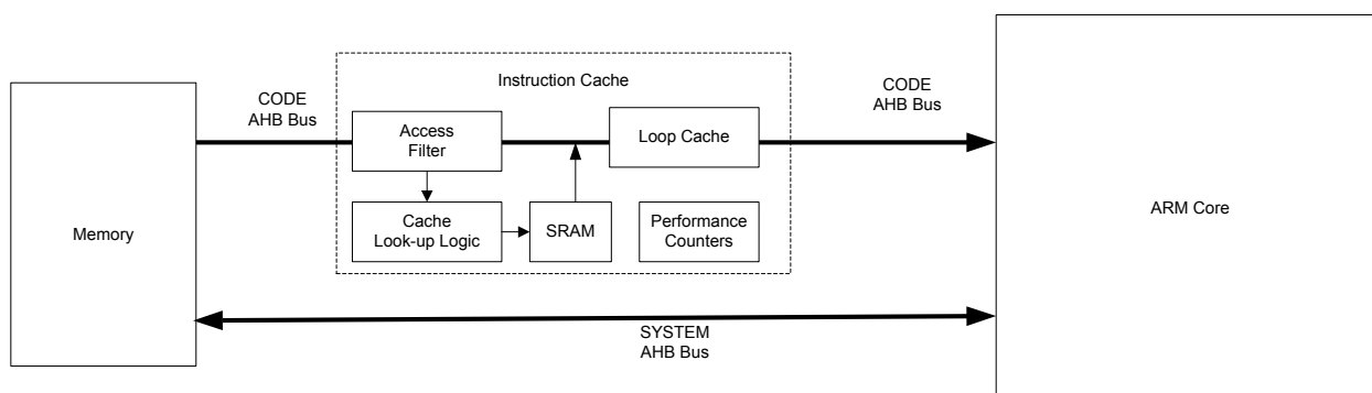
Figure 5.3. Instruction Cache Block Diagram
