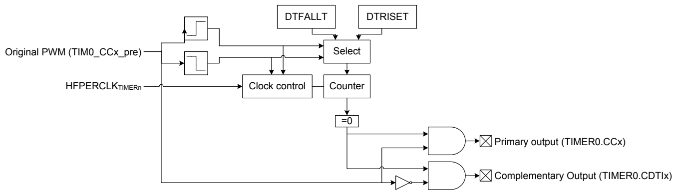
Figure 20.45. TIMER Overview of Dead-Time Insertion Block for a Single PWM Channel
