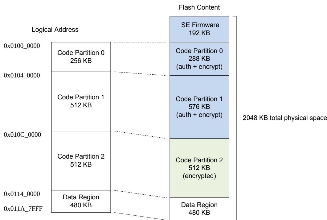
Figure 5.2. Flash Partitioning
