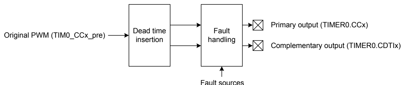
Figure 20.43. TIMER Dead-Time Insertion Unit Overview
