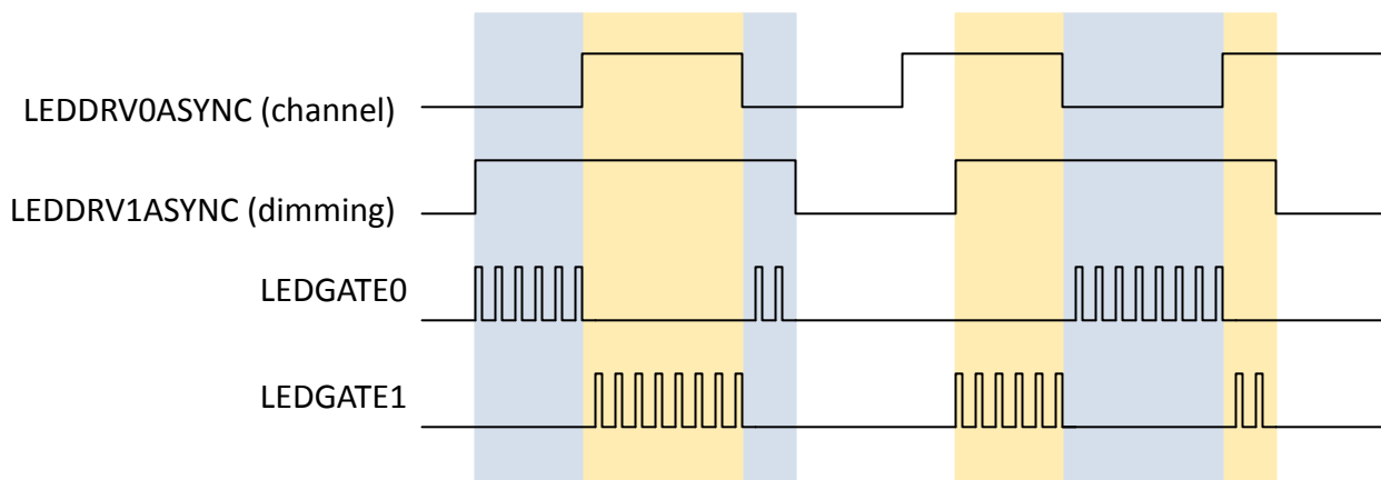
Figure 27.6. PWM Control
