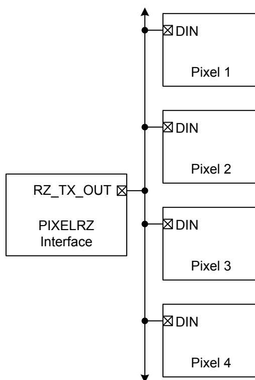
Figure 28.5. Parallel LED Connections
