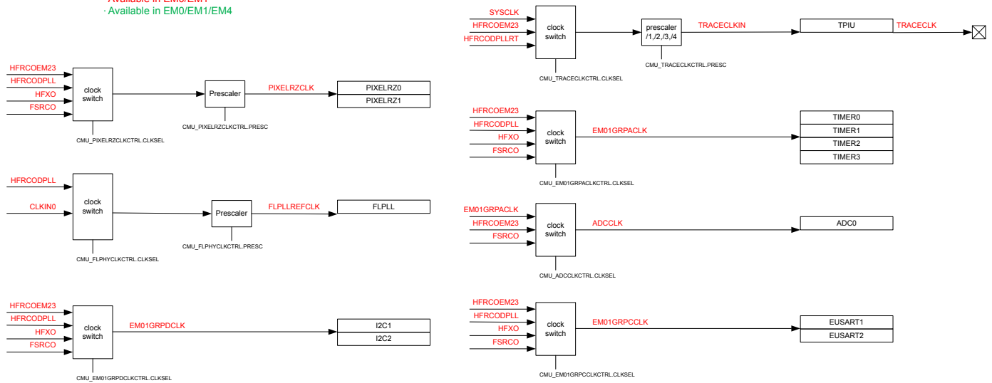
Figure 8.2. High-Frequency Peripheral Clocks
