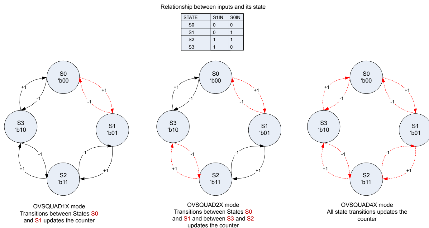
Figure 29.3. PCNT State Transitions for Different Oversampling Quadrature Decoder Modes
