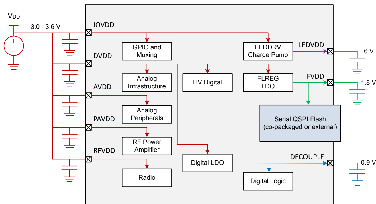
Figure 13.2. Single 3.0 - 3.6 V Supply
