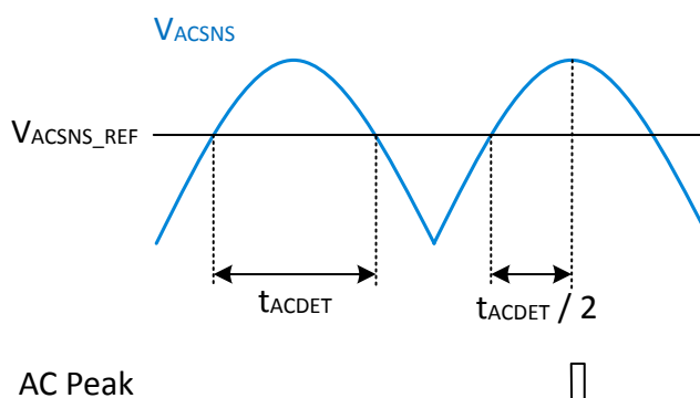
Figure 27.4. AC Peak Detection
