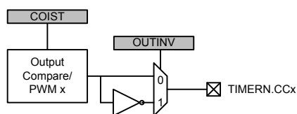
Figure 20.17. TIMER Output Logic
