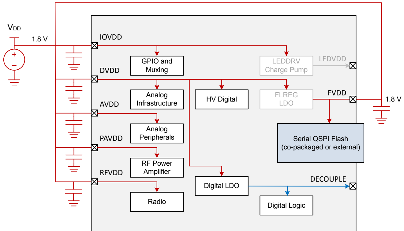
Figure 13.4. Single 1.8 V Supply
