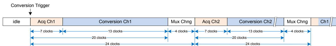
Figure 23.5. Continuous Two-Channel Conversion Example
