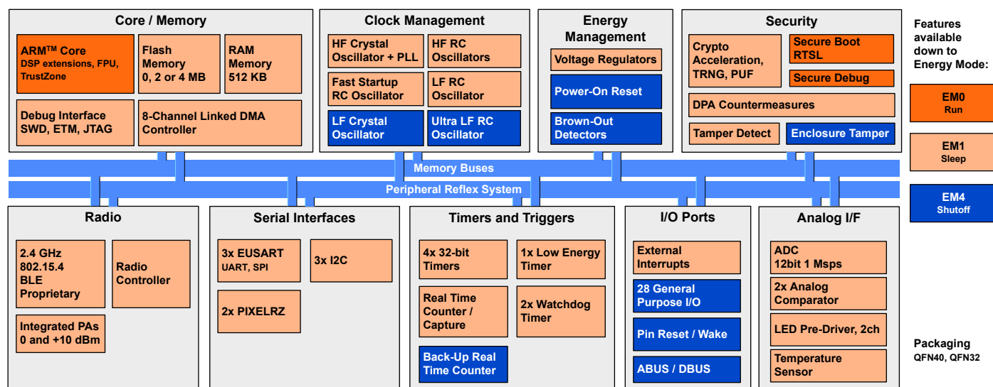
Figure 2.1. SiXG301 System-On-Chip Block Diagram
