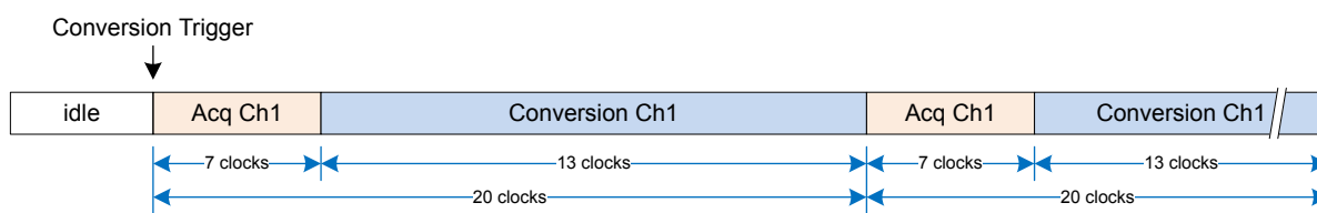
Figure 23.4. Continuous Single-Channel Conversion Example
