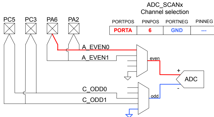
Figure 23.8. Single-Ended Port/Pin Selection Even Channel
