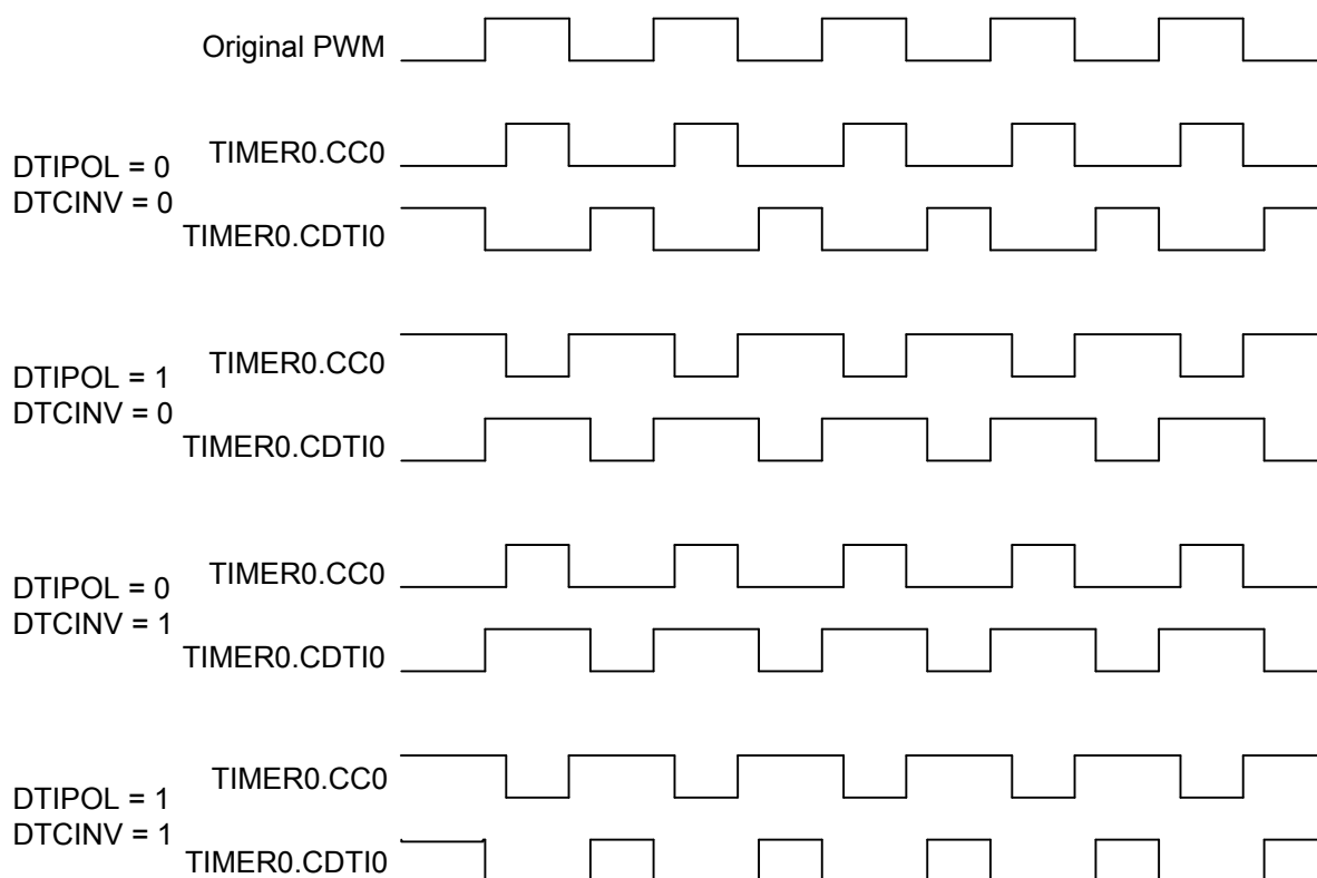
Figure 20.47. TIMER Output Polarities
