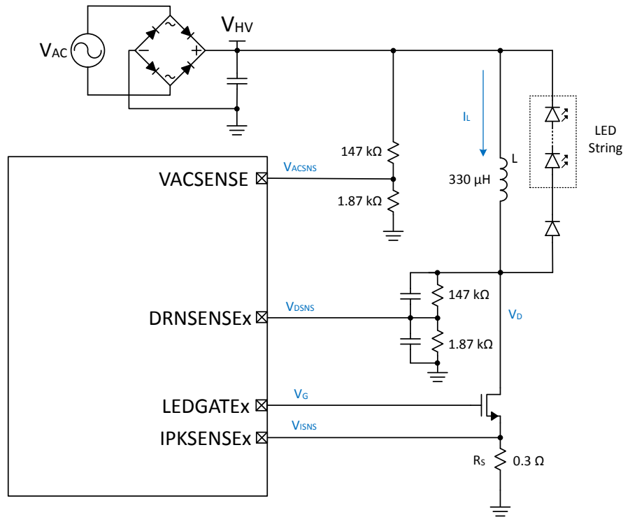
Figure 27.2. Example LED Schematic (One Channel)
