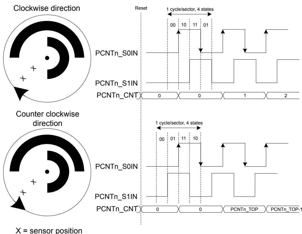
Figure 29.2. PCNT Quadrature Coding
