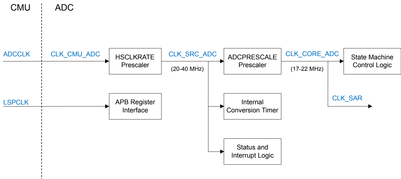
Figure 23.2. Clocking
