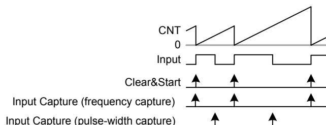
Figure 20.15. TIMER Period and/or Pulse Width Capture
