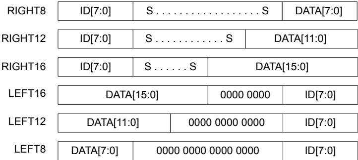
Figure 23.15. Data Alignment With ID
