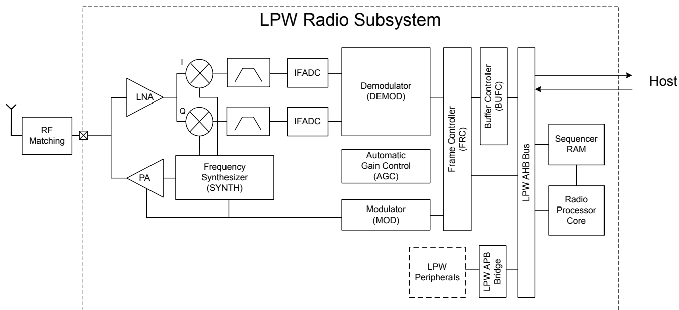
Figure 6.1. LPW Radio Subsystem Overview
