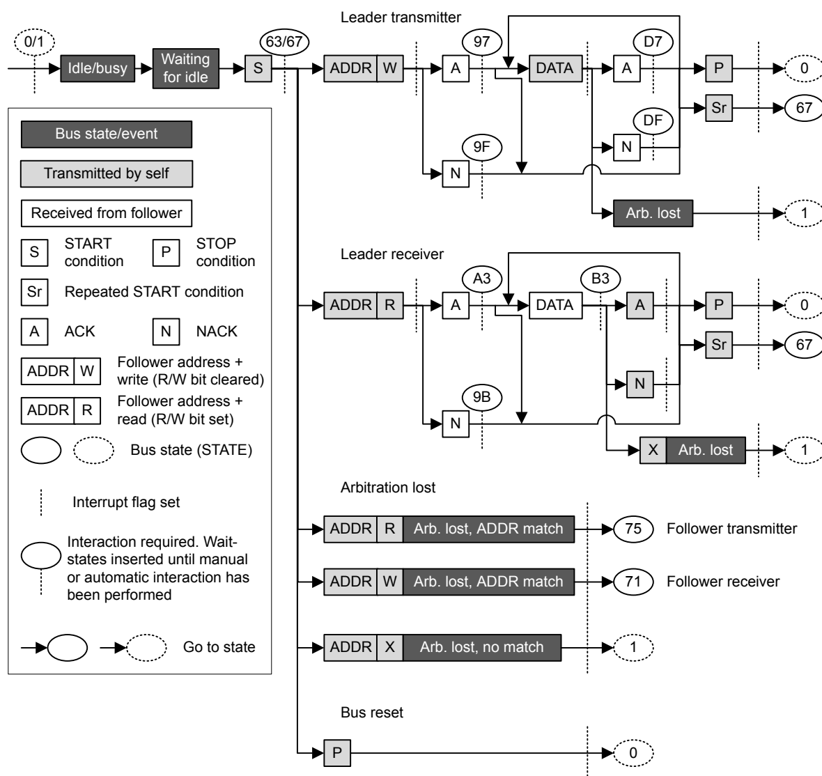
Figure 22.15. I2C Leader State Machine
