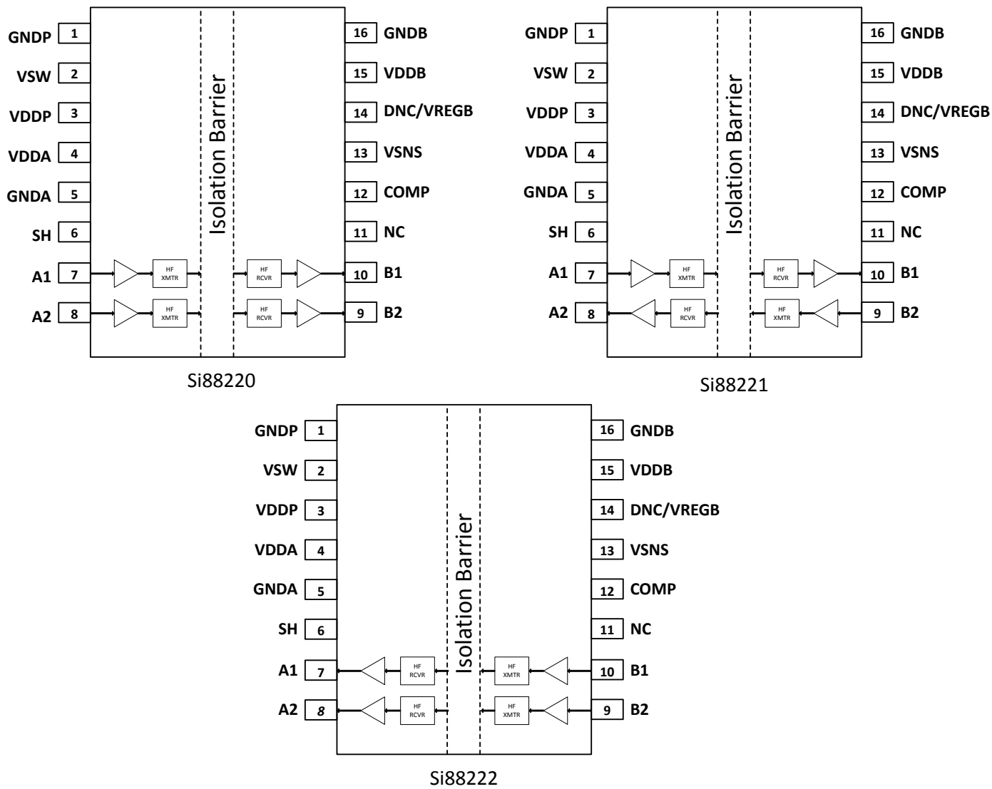
Figure 6.1. Si8822x Pin Configurations
