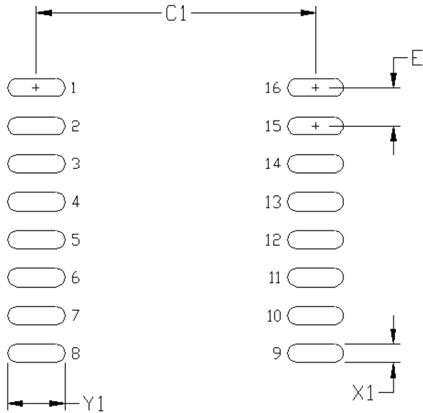
Figure 8.2. 16-Pin SOIC Land Pattern
