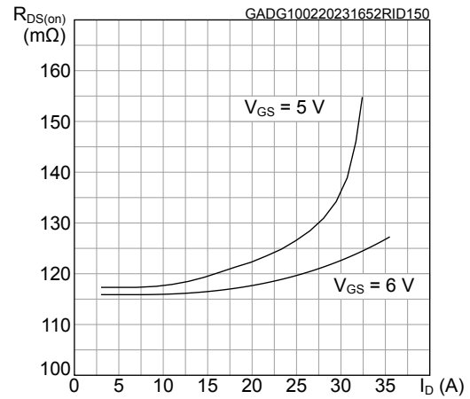
Figure 14. Typical drain-source on-resistance ( T_C = 150^\circ\text{C} )
