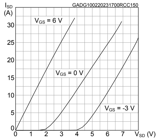
Figure 16. Typical reverse conduction characteristics ( T_C = 150^\circ\text{C} )
