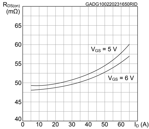
Figure 13. Typical drain-source on-resistance ( T_C = 25^\circ\text{C} )
