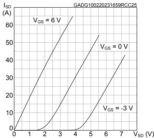
Figure 15. Typical reverse conduction characteristics ( T_C = 25^\circ\text{C} )
