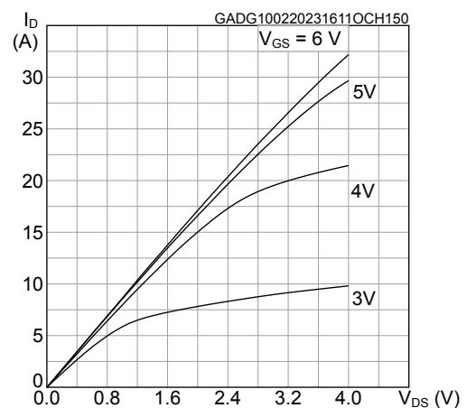
Figure 6. Typical output characteristics ( T_C = 150^\circ\text{C} )
