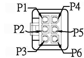
Output cable plug pin assignment
