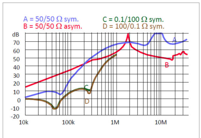
Figure 7. Typical Attenuation/Insertion loss Curves.
