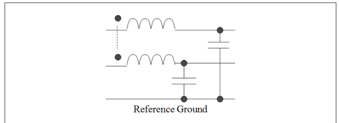
Figure 6. Common Mode Filtering.
