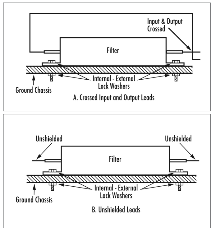
Figure 9. Separation of Input and Output Leads (Reference 7).
