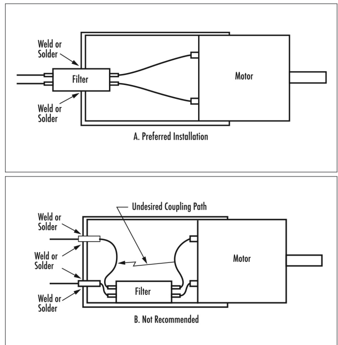
Figure 8. Lead Isolation (Reference 7).
