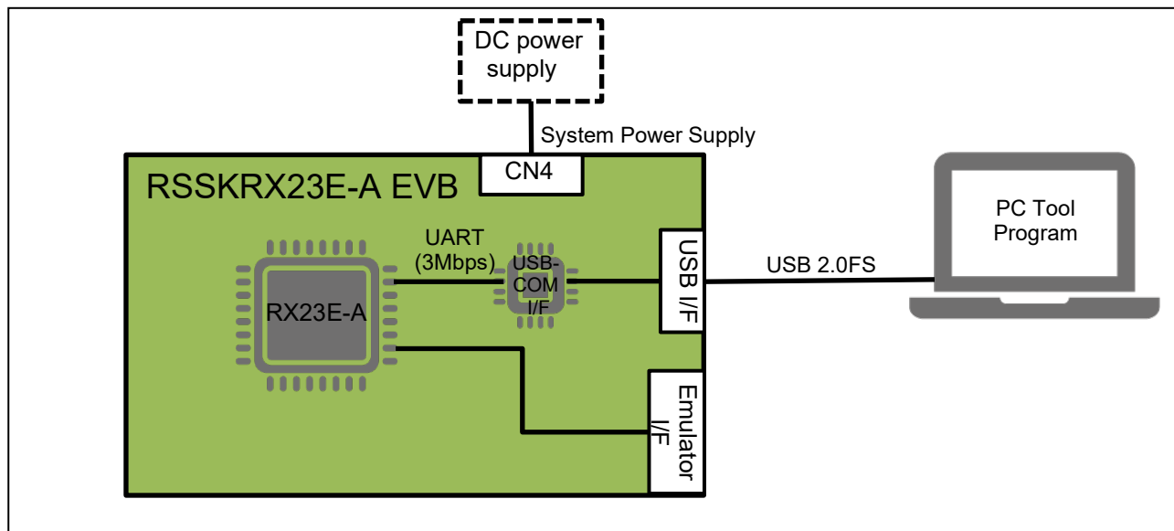
Figure 3-3 System Connection
