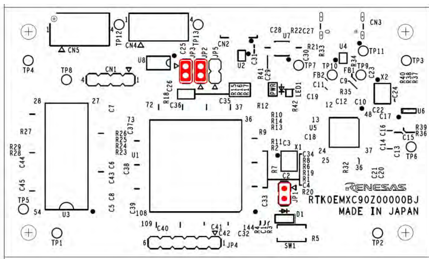
Figure 4-8 Default jumper pin setting of Communication board
