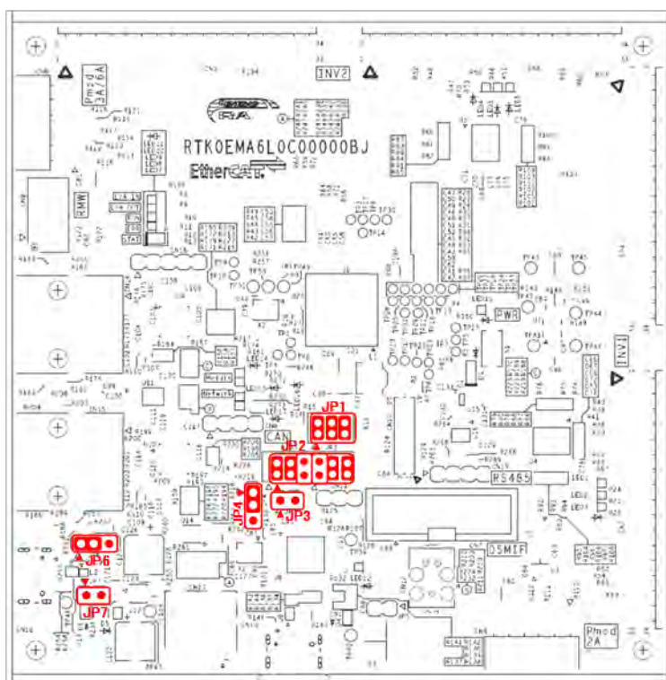
Figure 4-7 Default jumper pin setting of CPU board
