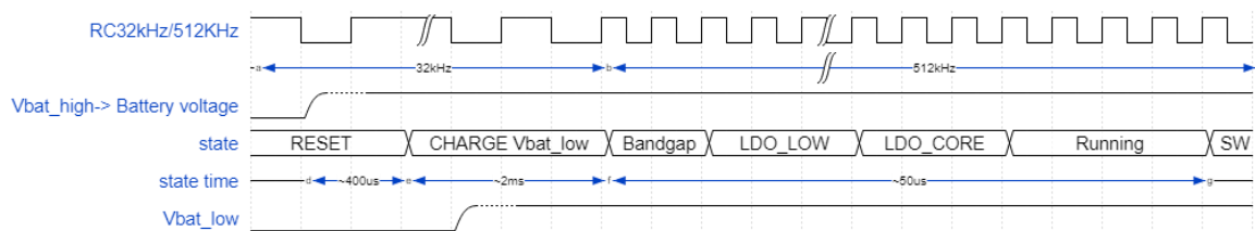
Figure 7. Powerup (Buck)
