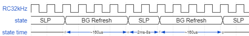
Figure 10. Go-to-sleep and bandgap refresh
