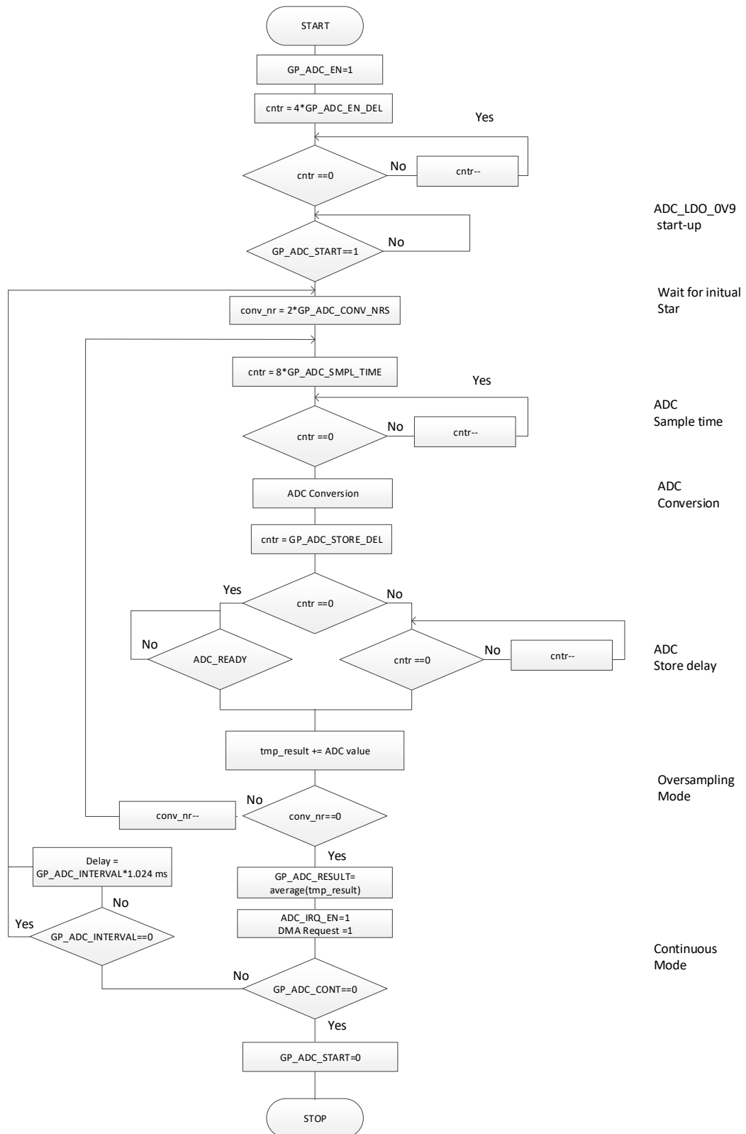
Figure 64. GPADC operation flow diagram
