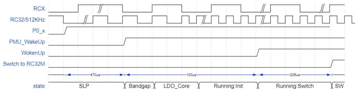
Figure 9. Wake-up (Buck)
