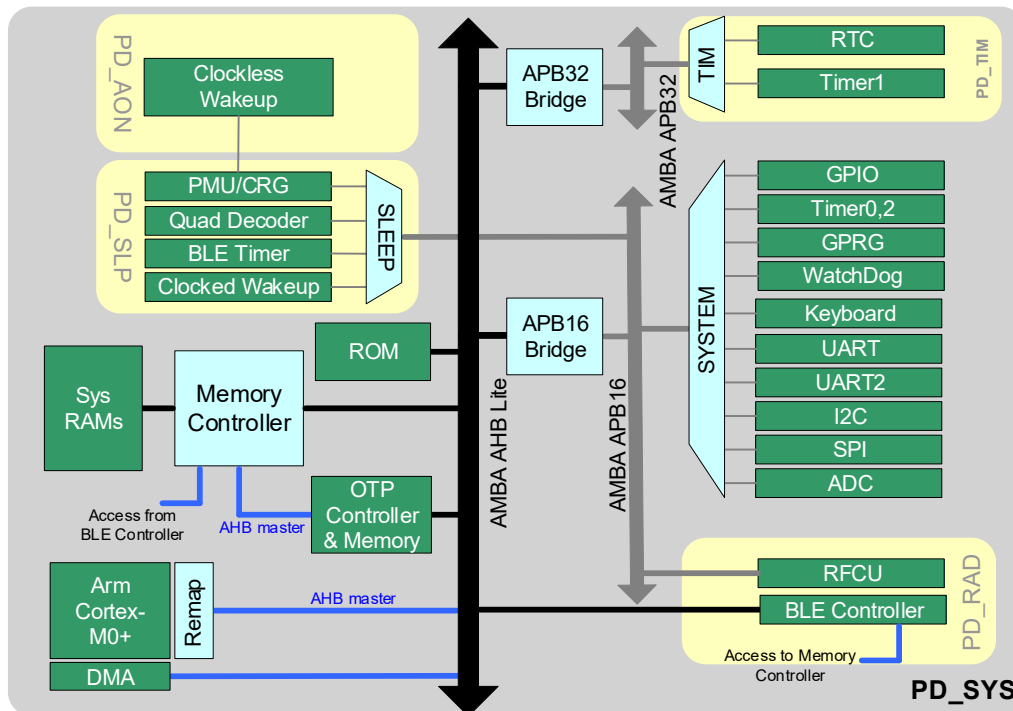
Figure 16. AMBA bus architecture and power domains
