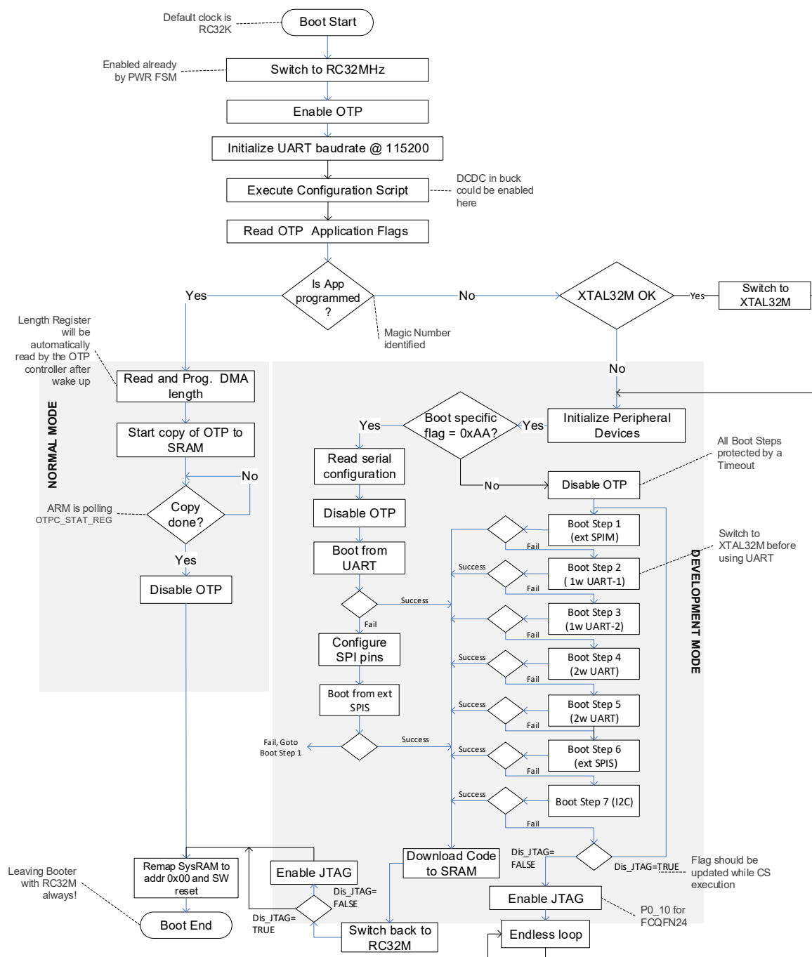
Figure 12. BootROM sequence
