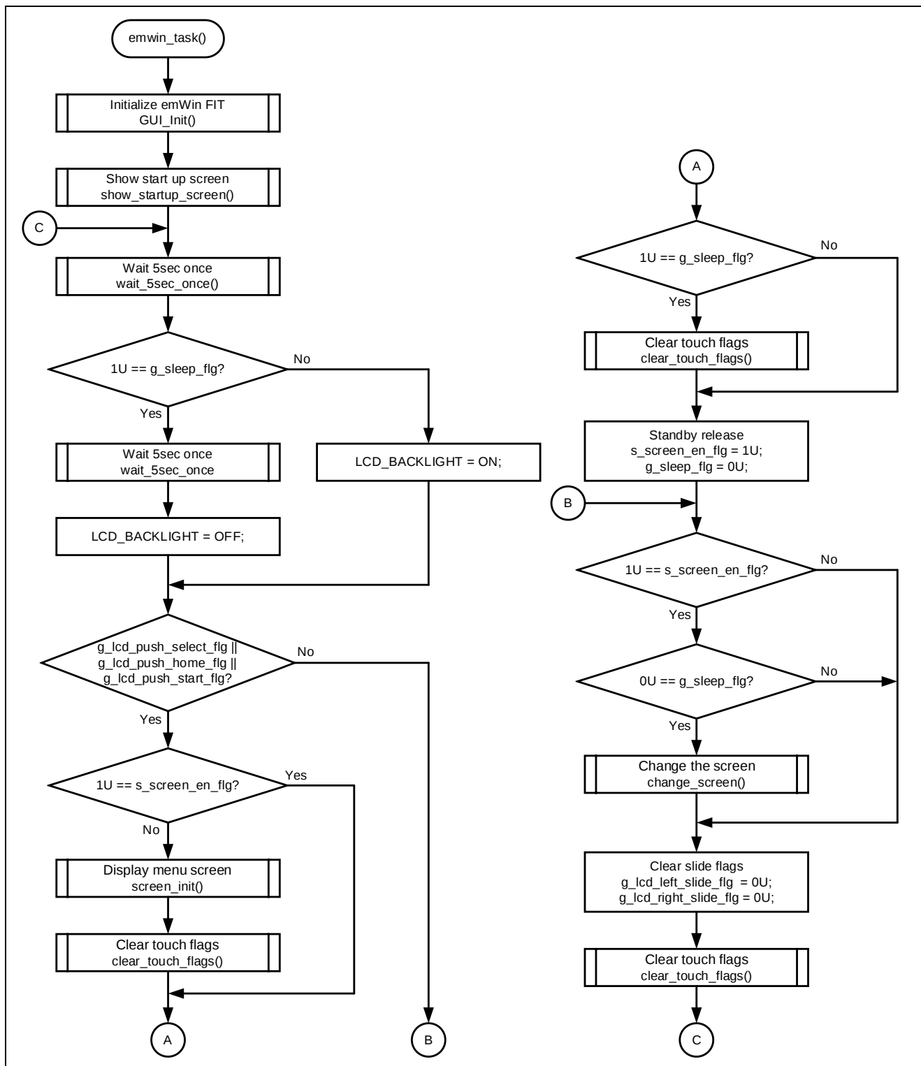
Figure 3-4 Overall flowchart of LCD control
