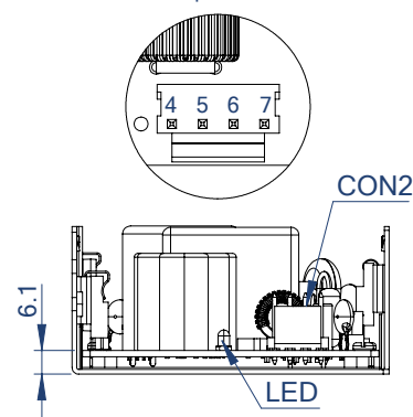
Detail CON2
