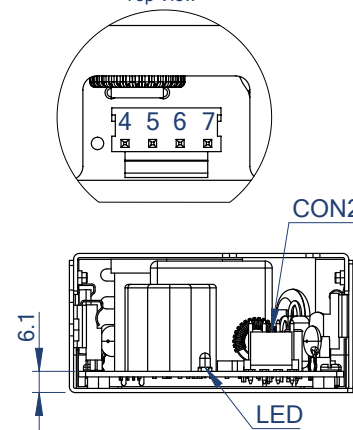
DETAIL CON2 Top View
