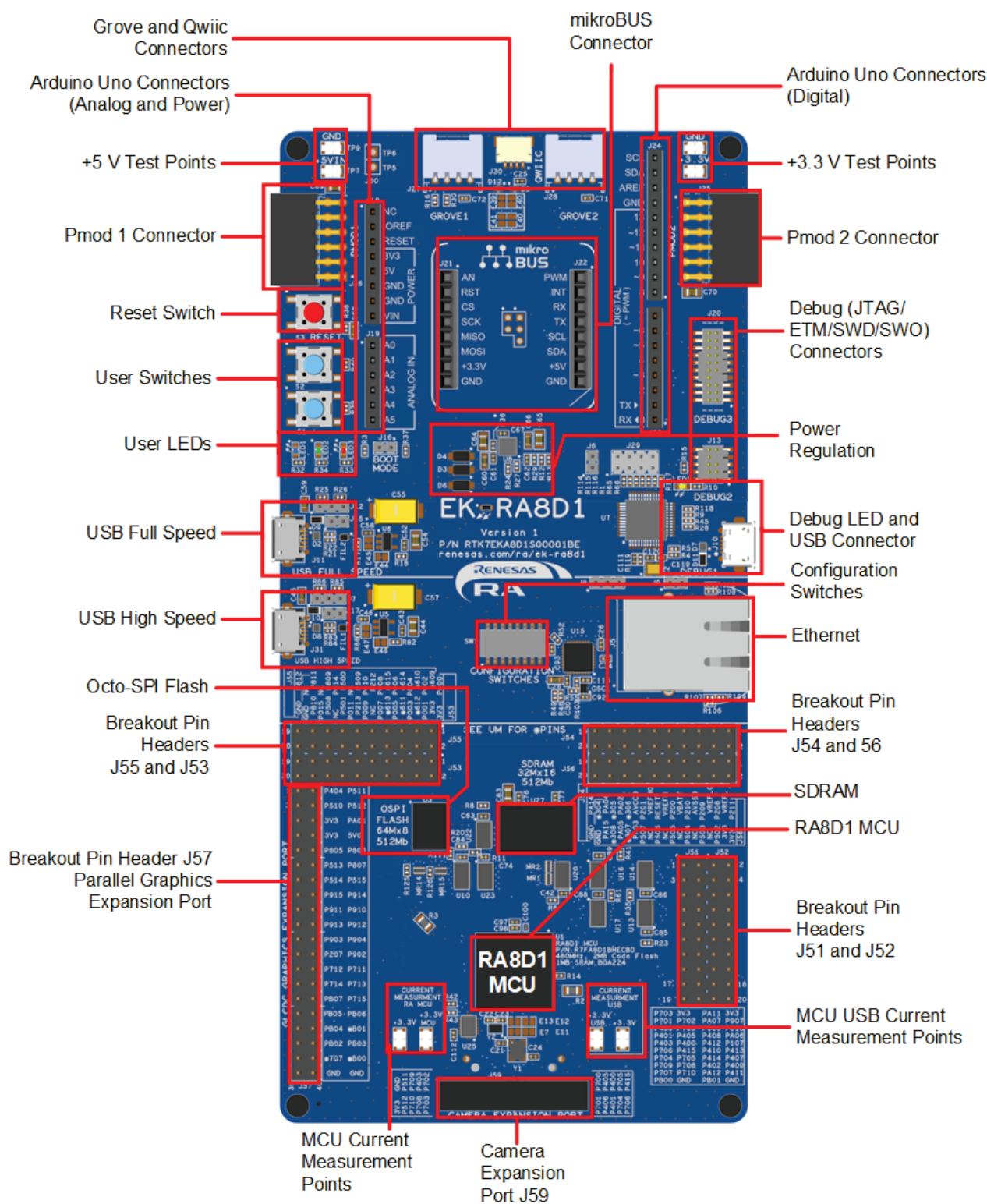
Figure 1. EK-RA8D1 Board Top Side
