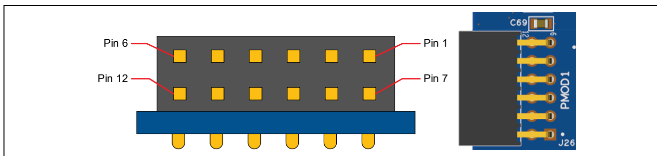
Figure 12. Pmod 1 Connector
