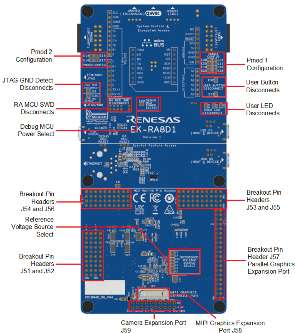
Figure 2. EK-RA8D1 Board Bottom Side
