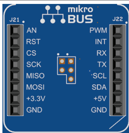
Figure 15. mikroBUS Connector
