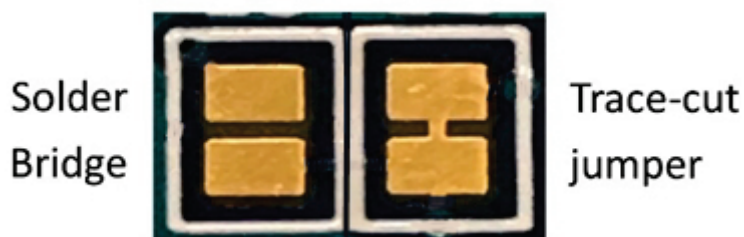
Figure 6. Copper Jumpers
