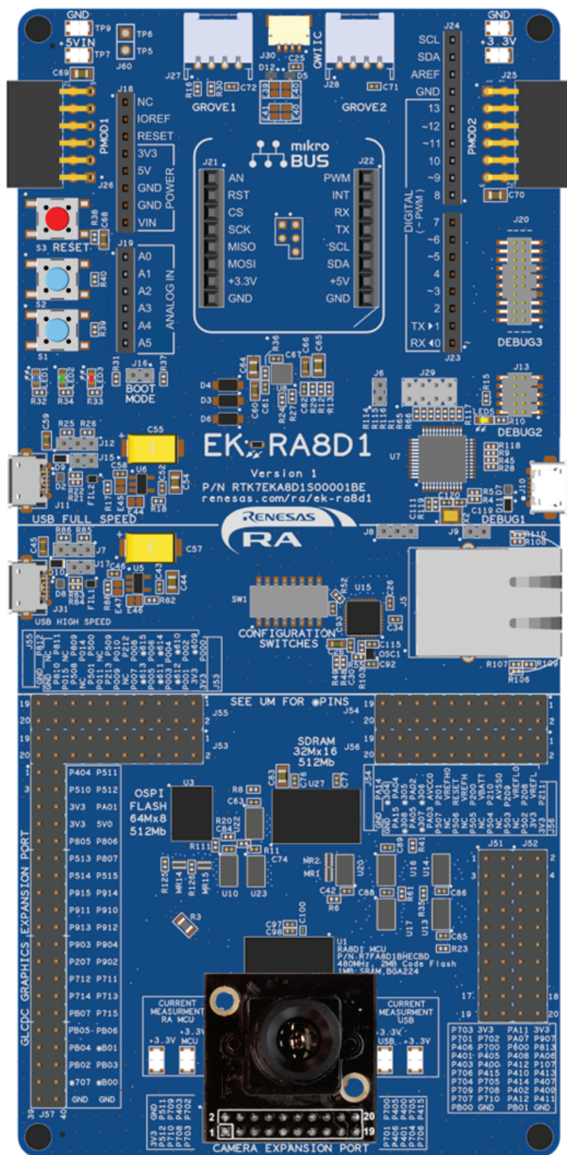
Figure 32. EK-RA8D1 Board Connected with Camera Expansion Board
