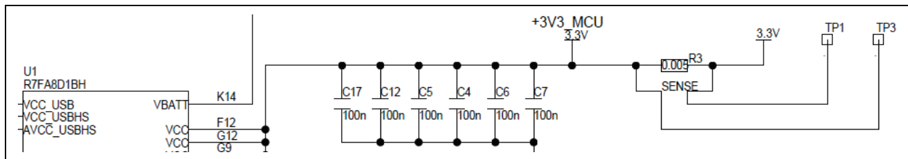
Figure 29. RA +3.3 V Current Measurement Circuit
