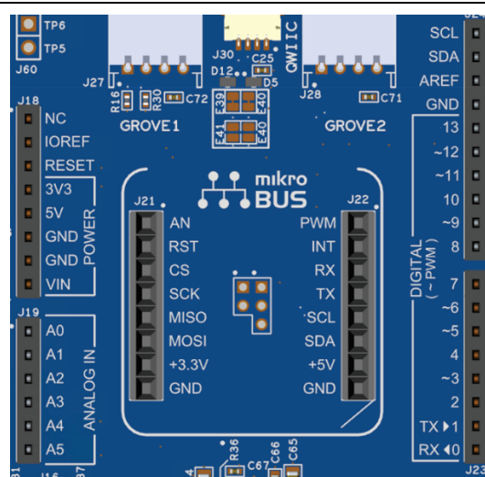
Figure 14. Arduino Uno Connectors
