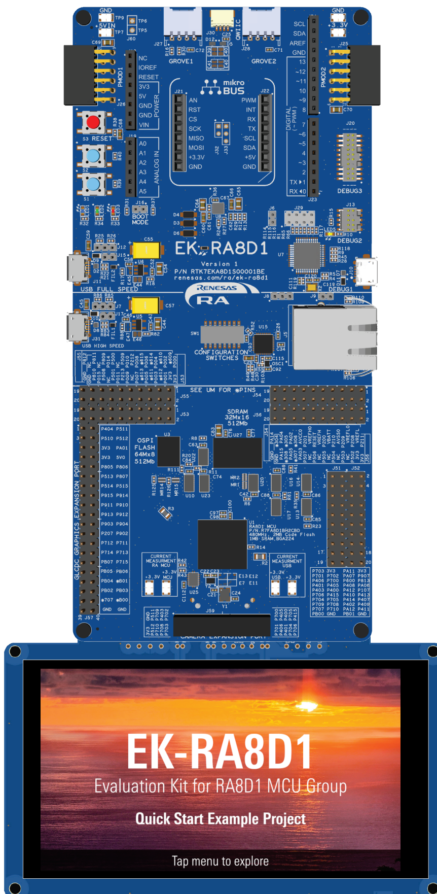
Figure 31. EK-RA8D1 Board Connected with MIPI Graphics Expansion Board
