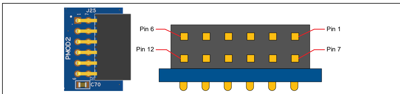
Figure 13. Pmod 2 Connector
