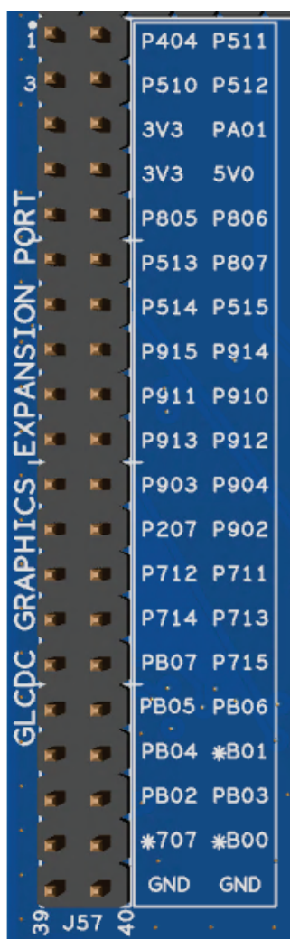
Figure 26. Parallel Graphics Expansion Port
