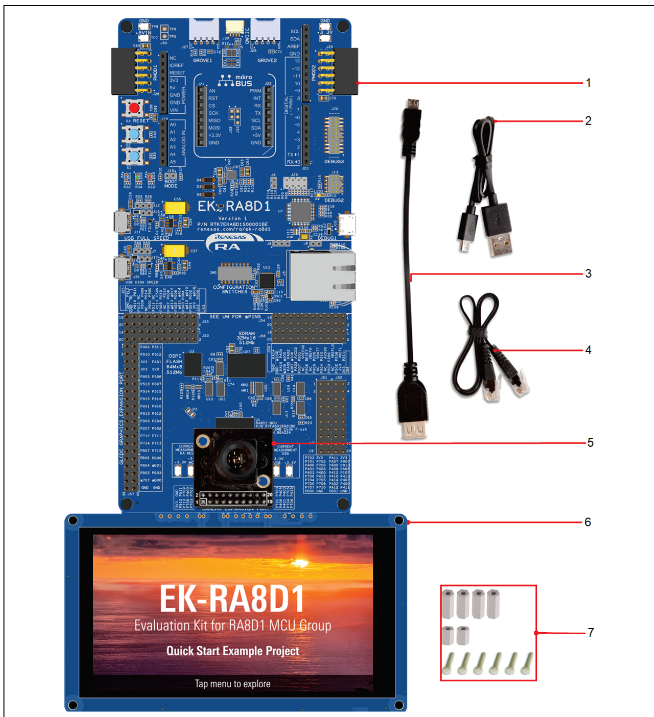
Figure 3. EK-RA8D1 Kit Contents
