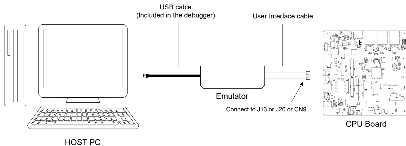
Figure 4-2: Emulator Connection Diagram (External Emulator)
