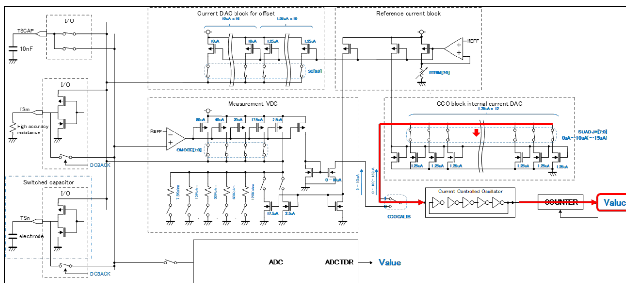
Figure 3.6 Circuits of SENSCLK Frequency Gain Test
