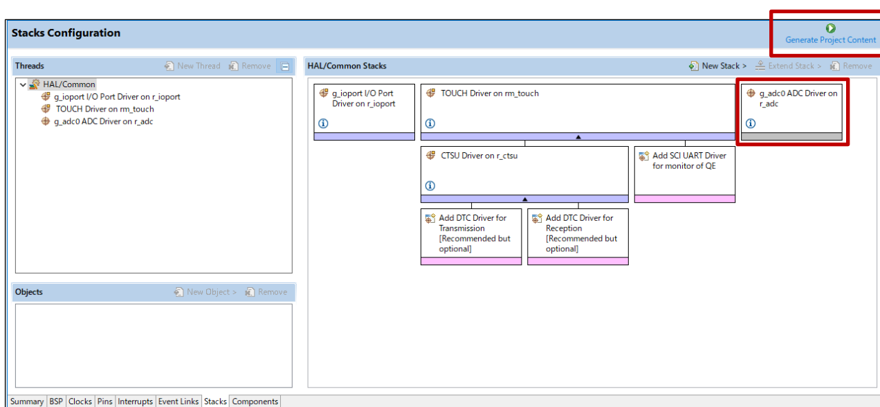
Figure 6.1 Stacks Configurations view
