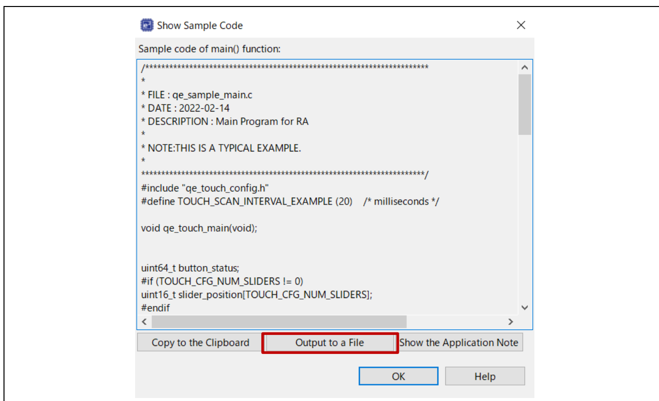
Figure 6.10 “Cap Touch Main (QE)”
