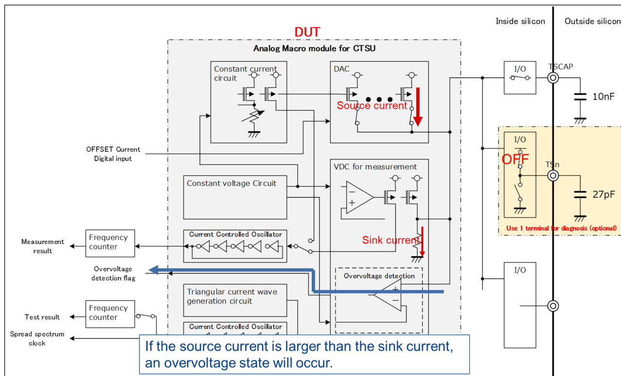
Figure 2.2 Circuits of Overvoltage Detection Test
