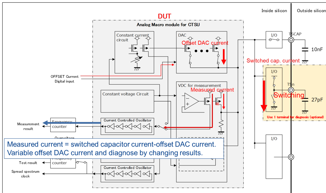
Figure 2.6.1 Circuits of Current Offset DAC Test
