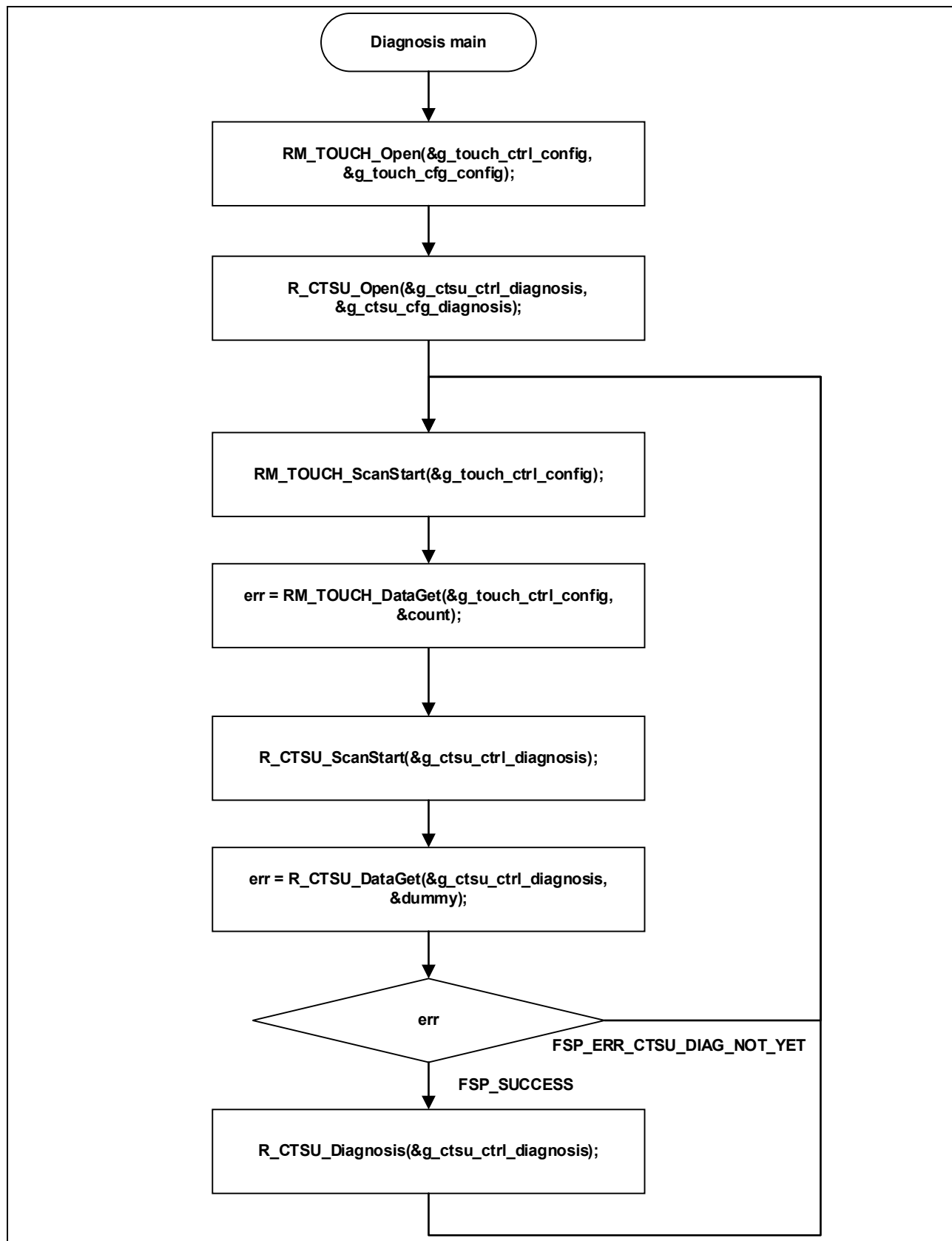
Figure 5.1 Flowchart of sample application for CTSU diagnosis
