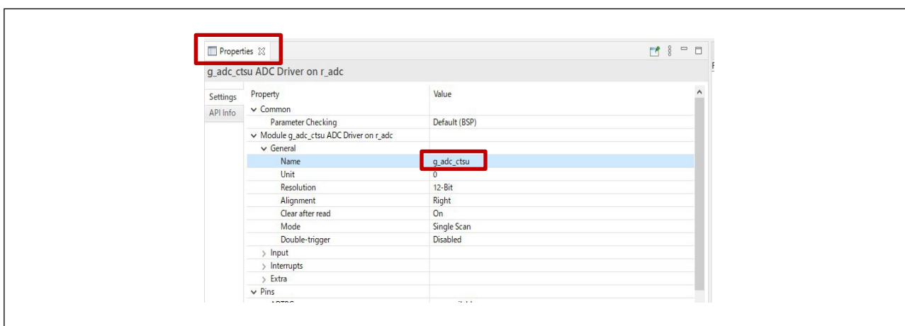
Figure 6.2 Change the name of “g_adc0”
