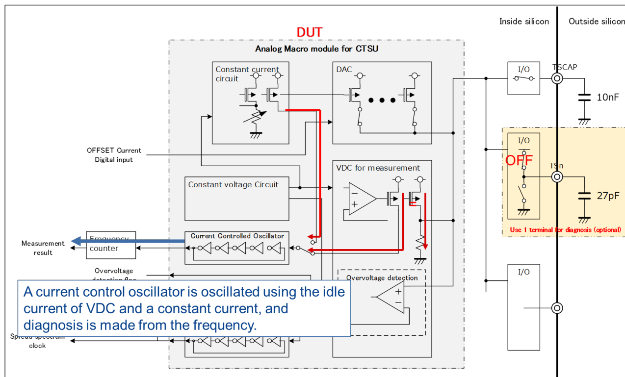
Figure 2.4 Circuits of Current Controlled Oscillator Test (2.5uA Correction Mode)
