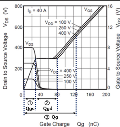
Figure 11. Gate Charge Characteristics (Ex: 500V/40A/0.102Ωtyp)
