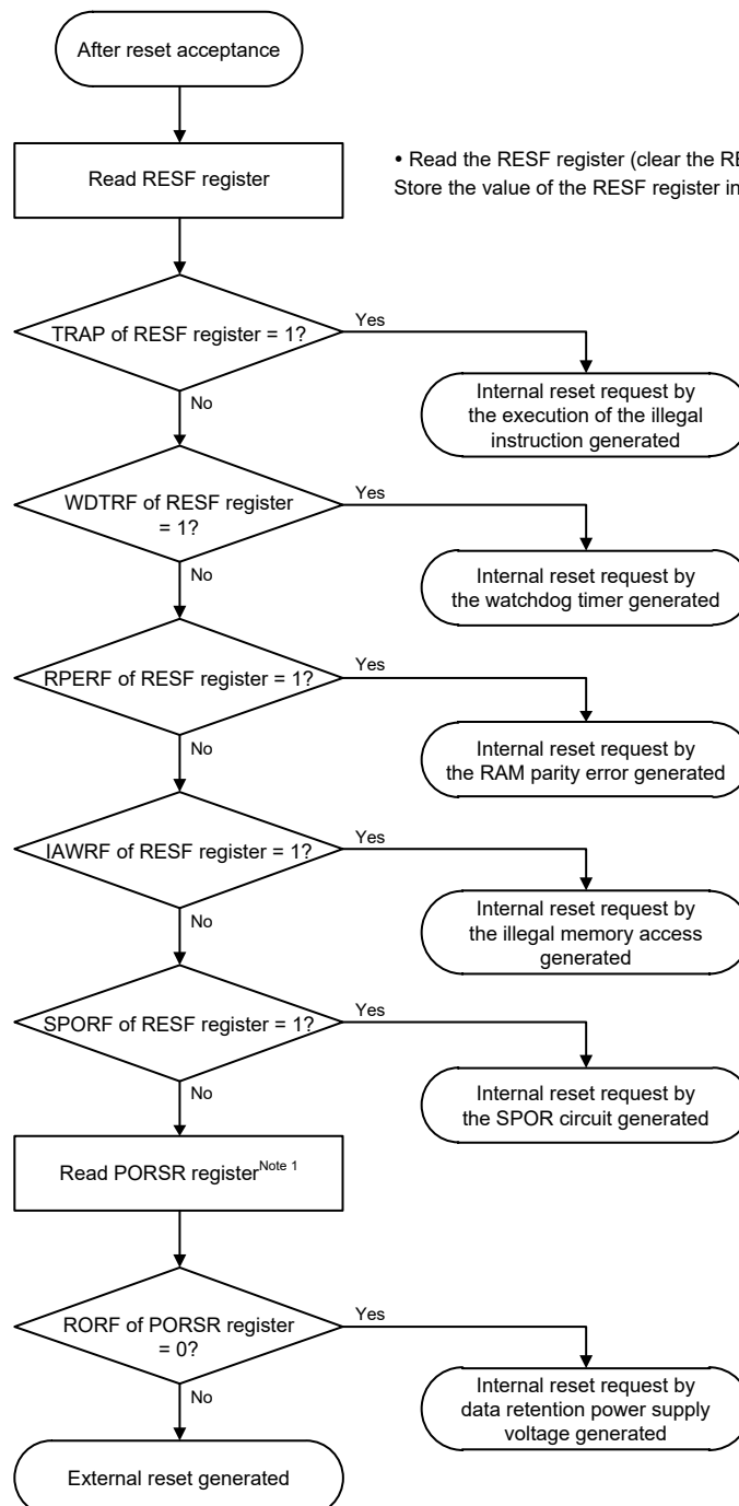
Figure 18-6. Example of Procedure for Checking Reset Source
