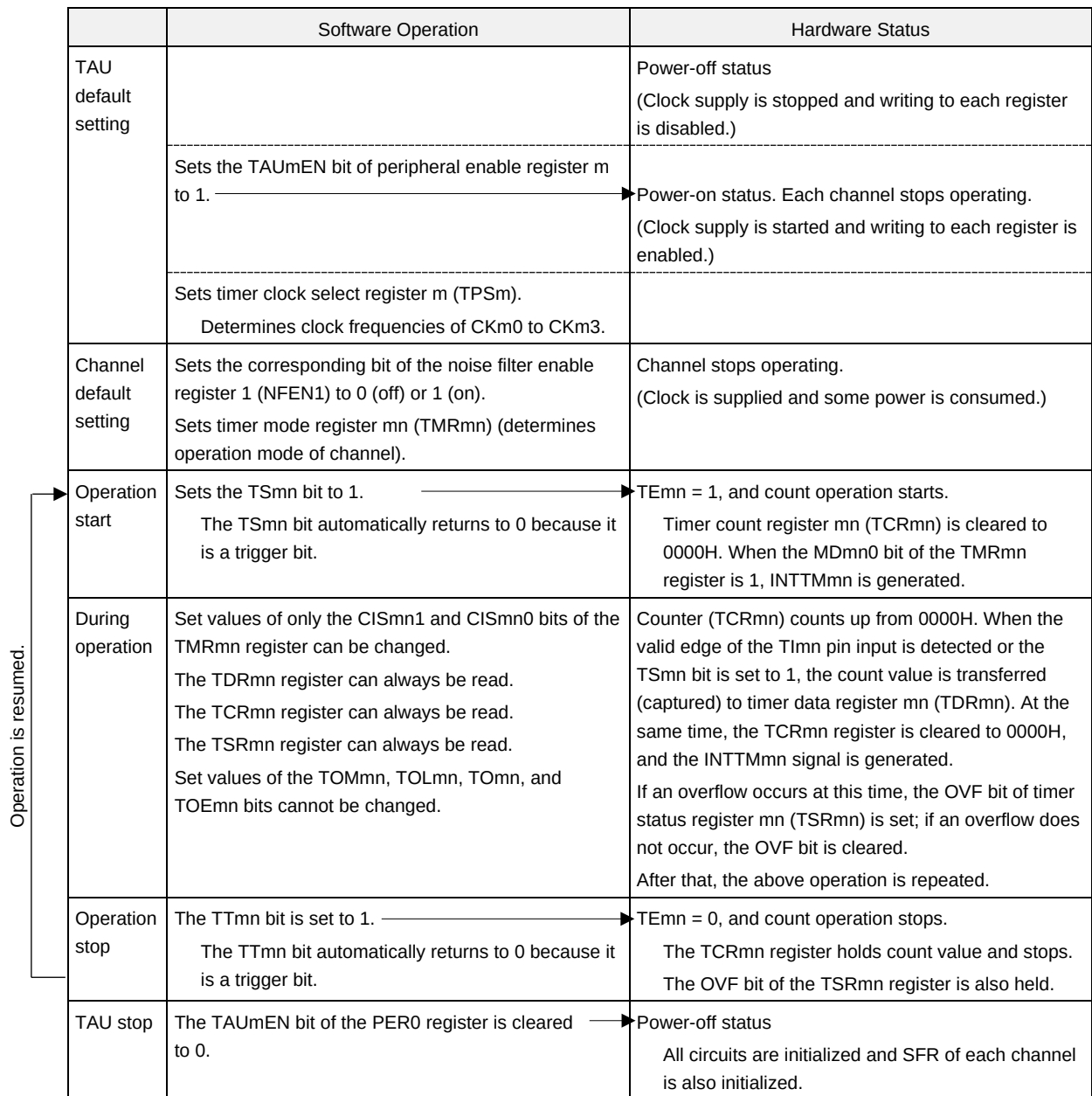
Figure 6-57. Operation Procedure When Input Pulse Interval Measurement Function Is Used
