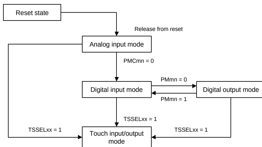
Figure 4-10. State Transition Diagram of ANIxx/TSxx/Port Pin Function
