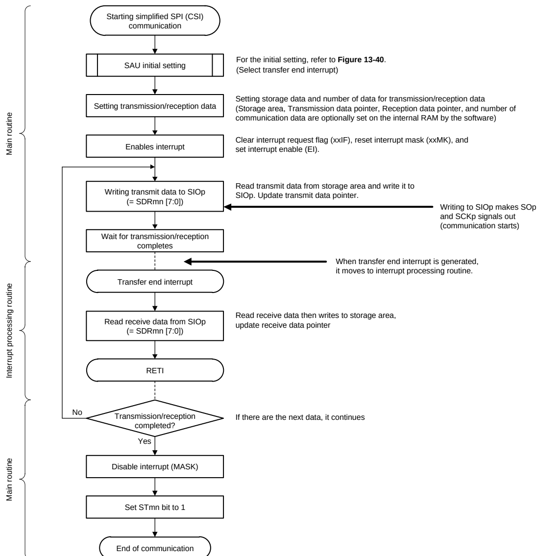
Figure 13-44. Flowchart of Master Transmission/Reception (in Single-Transmission/Reception Mode)
