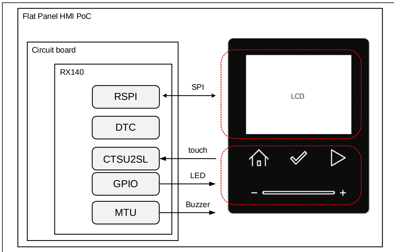
Figure 1-2 System configuration
