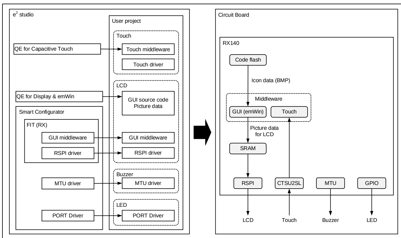
Figure 1-3 Software configuration
