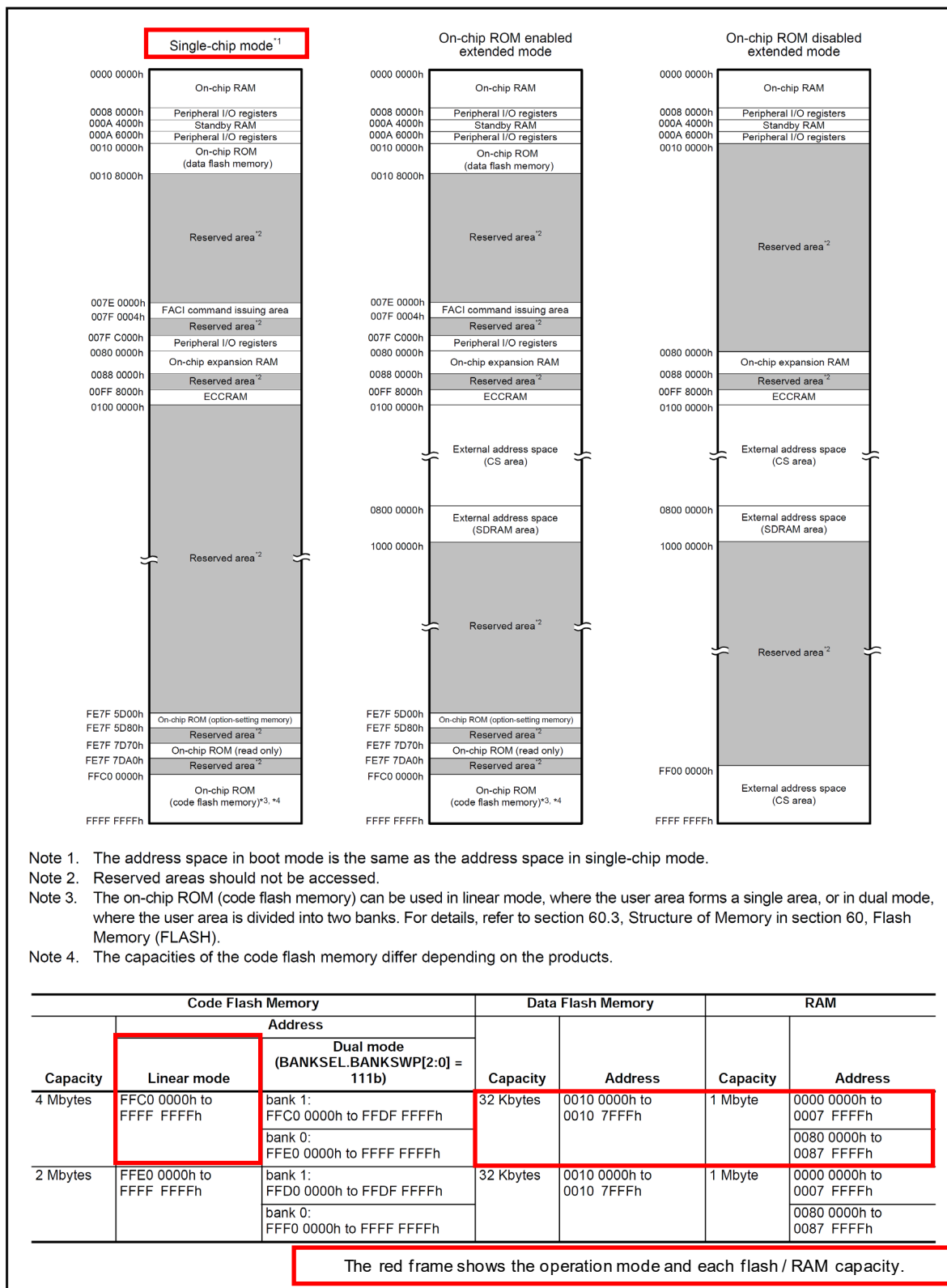
Figure 4-1: RX66N Memory map
