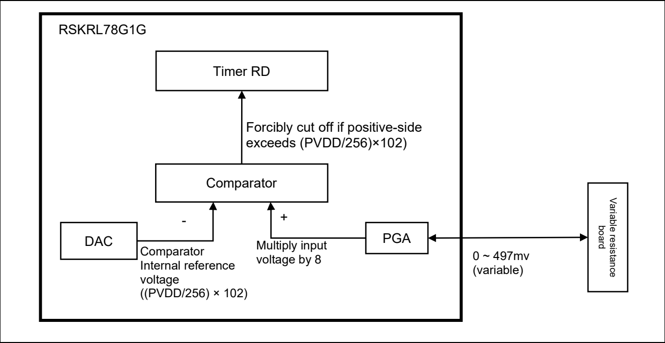
Figure 1.1 Operation Outline
