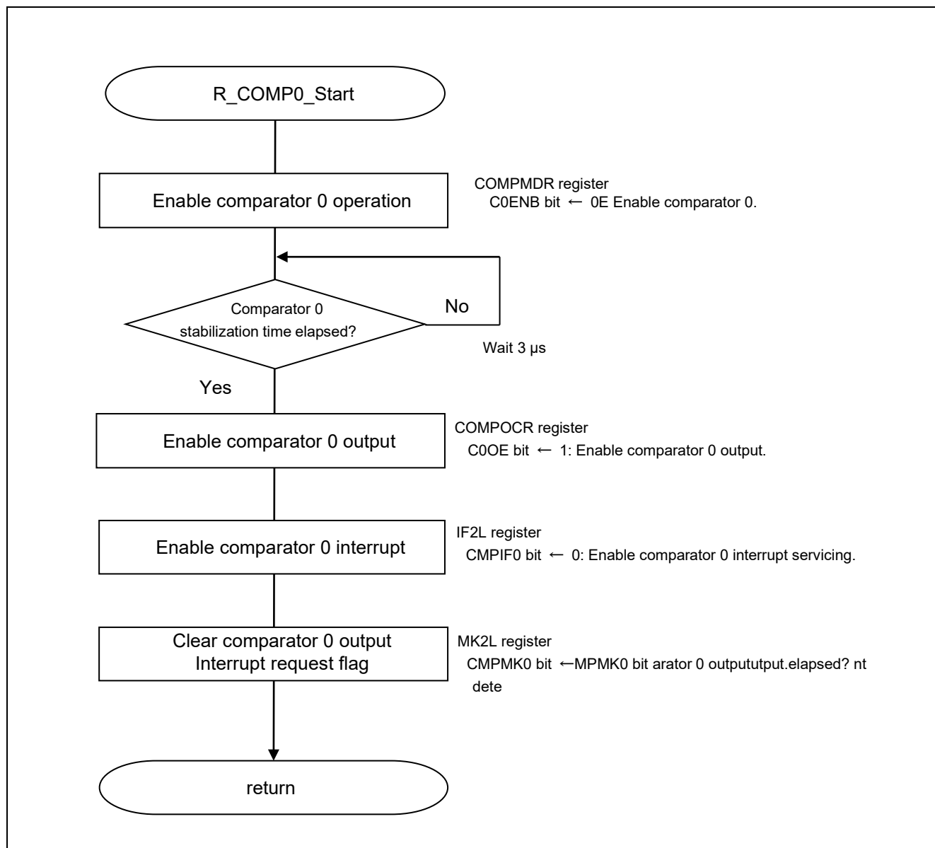
Figure 4.24 Comparator 0 Startup
