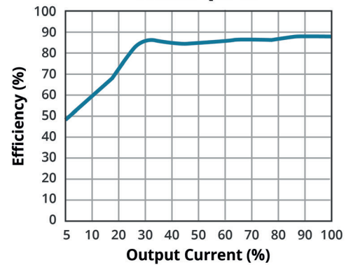
EFFICIENCY VS OUTPUT LOAD ( V_{in} = 24V ) PYBE30-Q24-S5
