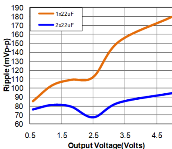
Figure 38. Input ripple voltage for various output voltages with 1x22 \mu F or 2x22 \mu F ceramic capacitors at the input (6A load). Input voltage is 12V.
