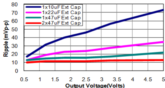
Figure 39. Output ripple voltage for various output voltages with external 1x10 \mu F, 1x22 \mu F, 1x47 \mu F and 2x47 \mu F ceramic capacitors at the output (6A load). Input voltage is 12V.
