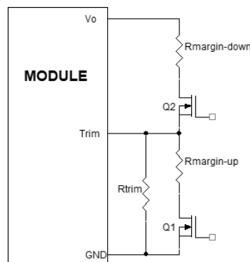
Figure 44. Circuit Configuration for margining Output voltage.
