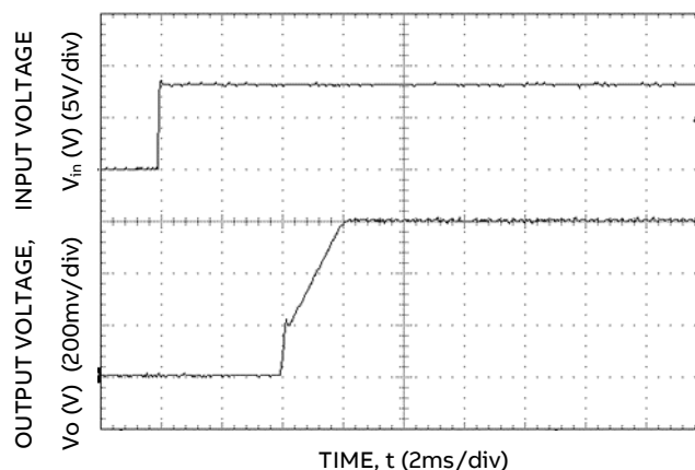
Figure 6. Typical Start-up Using Input Voltage ( V_{IN}=8\text{V} , I_o=I_{o,max} ).
