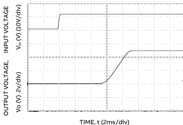
Figure 36. Typical Start-up Using Input Voltage ( V_{IN}=12V , I_o=I_{o,max} ).
