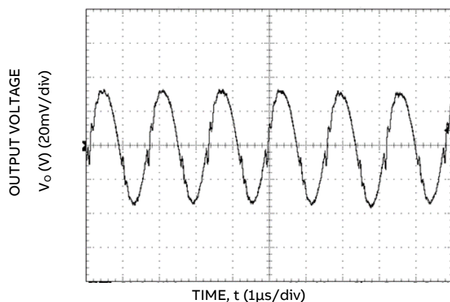
Figure 33. Typical output ripple and noise ( C_O=10\mu F ceramic, V_{IN}=12V , I_o=I_{o,max} ).
