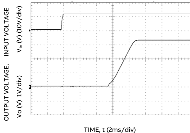
Figure 30. Typical Start-up Using Input Voltage ( V_{IN}=12V , I_O=I_{O,max} ).
