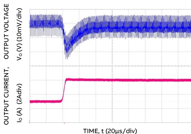
Figure 10. Transient Response to Dynamic Load Change from 50% to 100% at 12Vin, C_{out}=1x47\mu\text{F}+3x330\mu\text{F} , CT_{tune}=12\text{nF} , RT_{tune}=178
