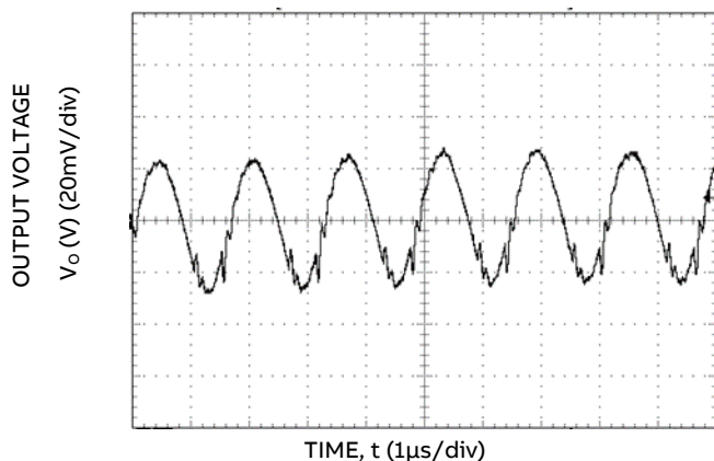
Figure 27. Typical output ripple and noise ( C_O=10\mu F ceramic, V_{IN}=12V , I_O=I_{O,max} ).
