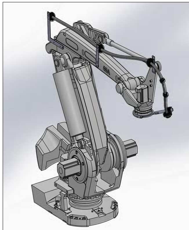
34.36.021.01 Complete robotic dresspack, Axis 1-3, without retraction system, high-flex conduit with ID 28.7mm
