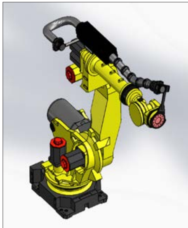
23.70.120.01 Complete robotic dresspack, Axis 3-6, TecLiner retraction system, 350mm stroke, high-flex conduit with ID 64mm
