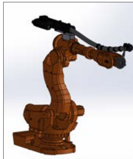
25.70.321.01 Complete robotic dresspack, Axis 3-6, TecBox retraction system, 600mm stroke, high-flex conduit with ID 64mm
