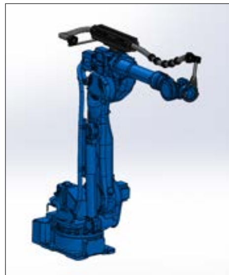
20.48.421.01 Complete robotic dresspack, Axis 3-6, TecLiner retraction system, 400mm stroke, high-flex conduit with ID 36.7mm
