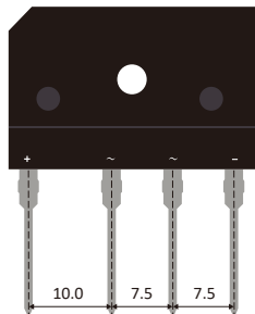
GBL-2
