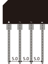
GBL-2
