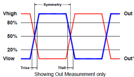
Test Waveform
