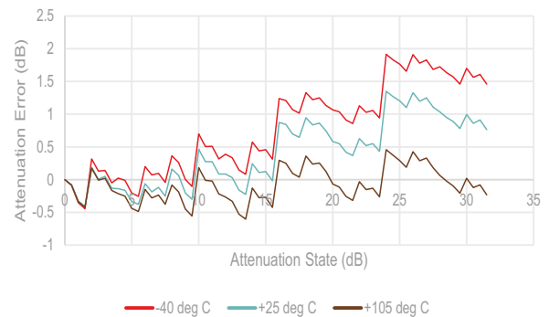
Figure 24 ■ Attenuation Error @ 43.5 GHz vs. Temperature
