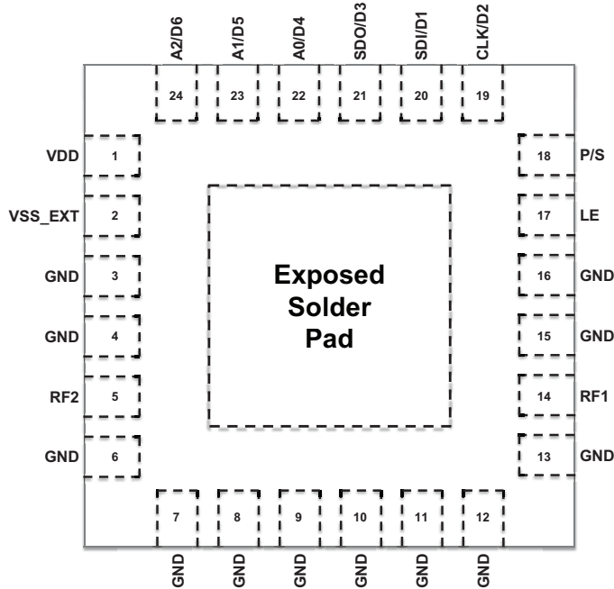
Figure 37 ■ Pin Configuration (Top View) for the PE43614
