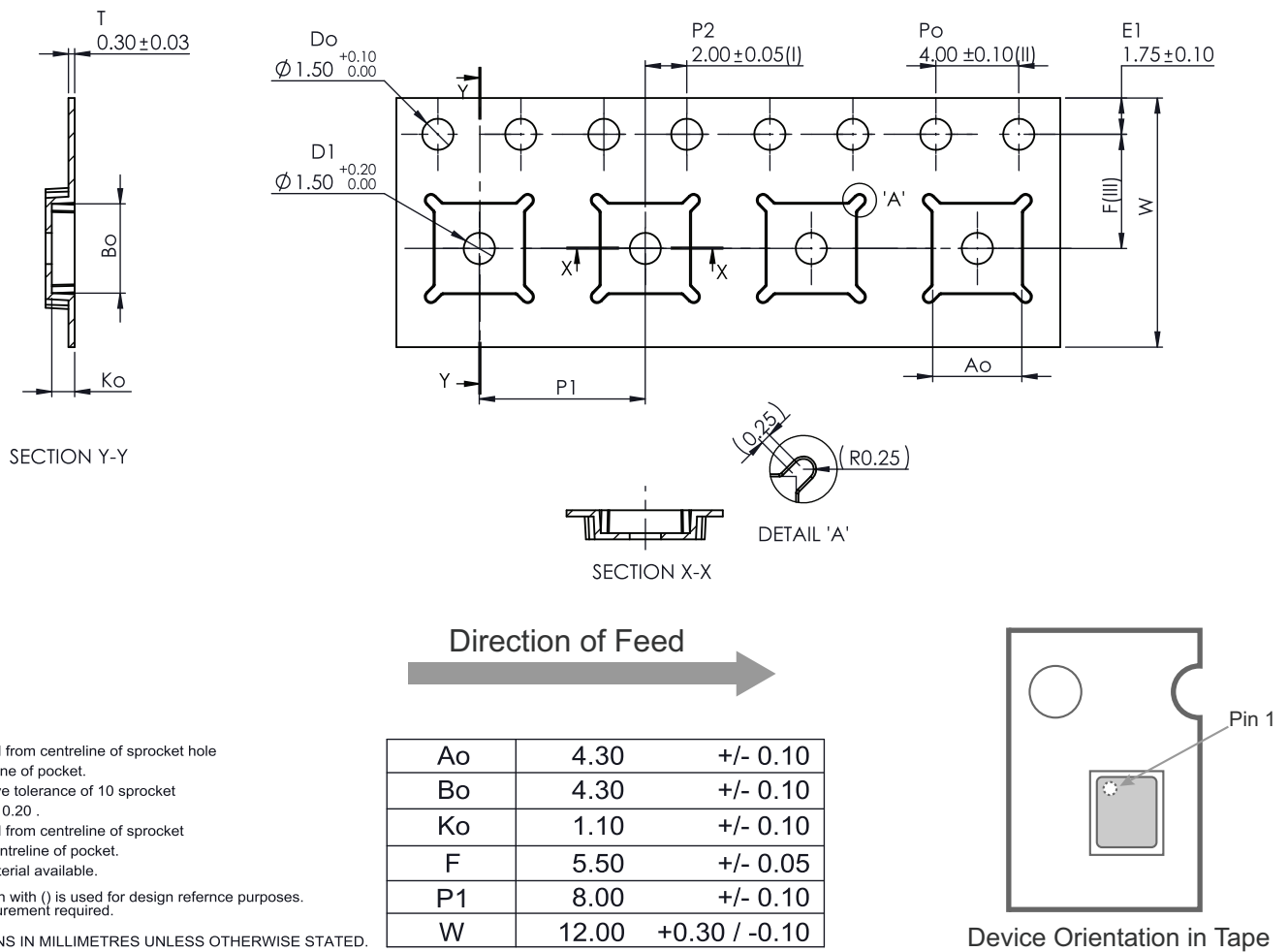
Figure 40 ■ Tape and Reel Specifications for 24-lead 4 x 4 mm LGA
