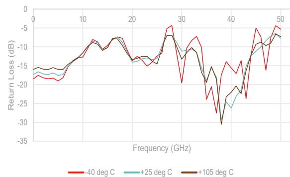
Figure 10 ■ Output Return Loss (Ref State) vs. Temperature
