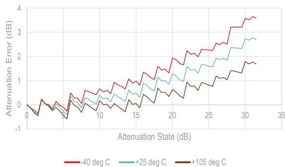
Figure 23 ■ Attenuation Error @ 40 GHz vs. Temperature
