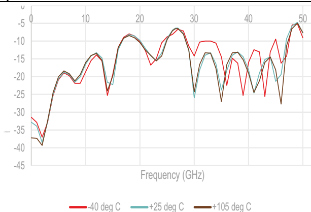
Figure 11 ■ Output Return Loss (Ref State) vs. Temperature
