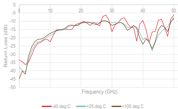
Figure 11 ■ Output Return Loss (Ref State) vs. Temperature
