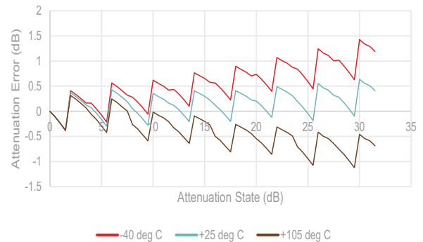
Figure 22 ■ Attenuation Error @ 26.5 GHz vs. Temperature
