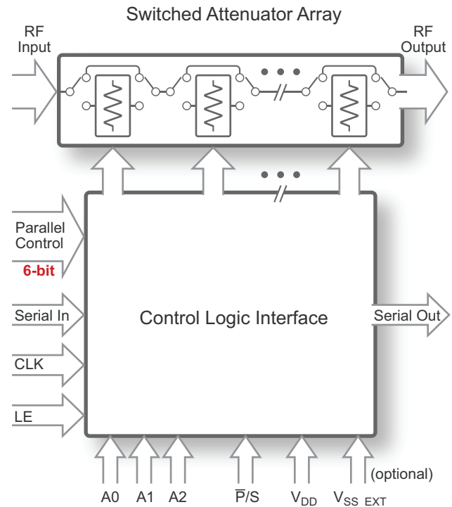
Figure 1 ■ PE43614 Functional Diagram
