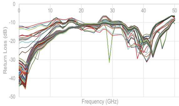
Figure 15 ■ Output Return Loss (All Attenuation States)
