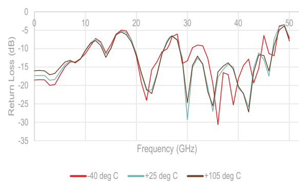
Figure 12 ■ Input Return Loss (Major Attenuation States)
