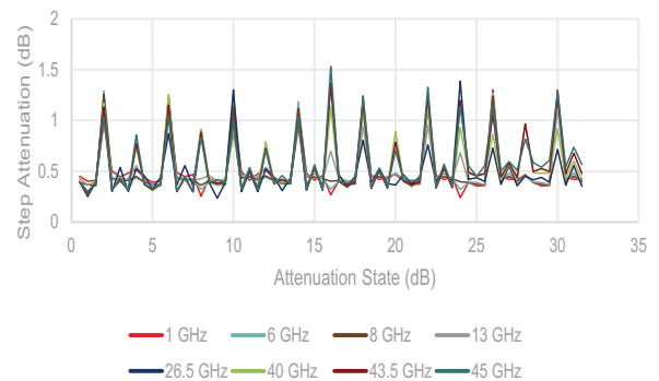
Figure 28 ■ 0.5 dB Step Actual vs. Frequency
