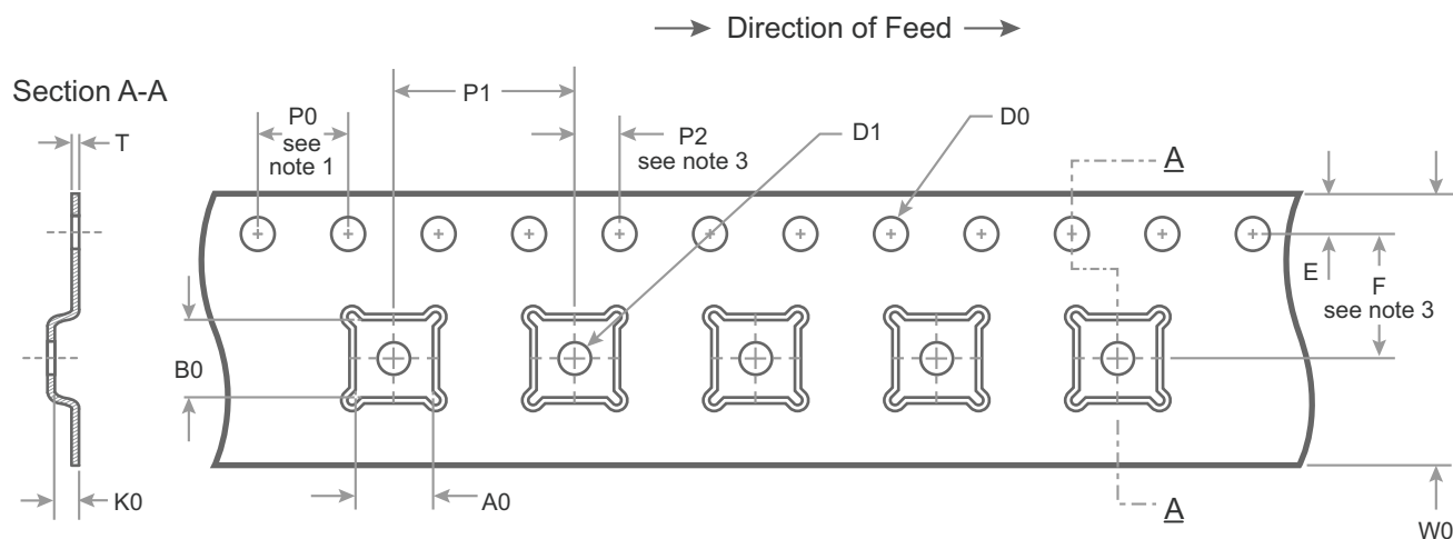
Figure 24 • Tape and Reel Specifications for 32-lead 5 \times 5 \times 0.85 mm QFN
