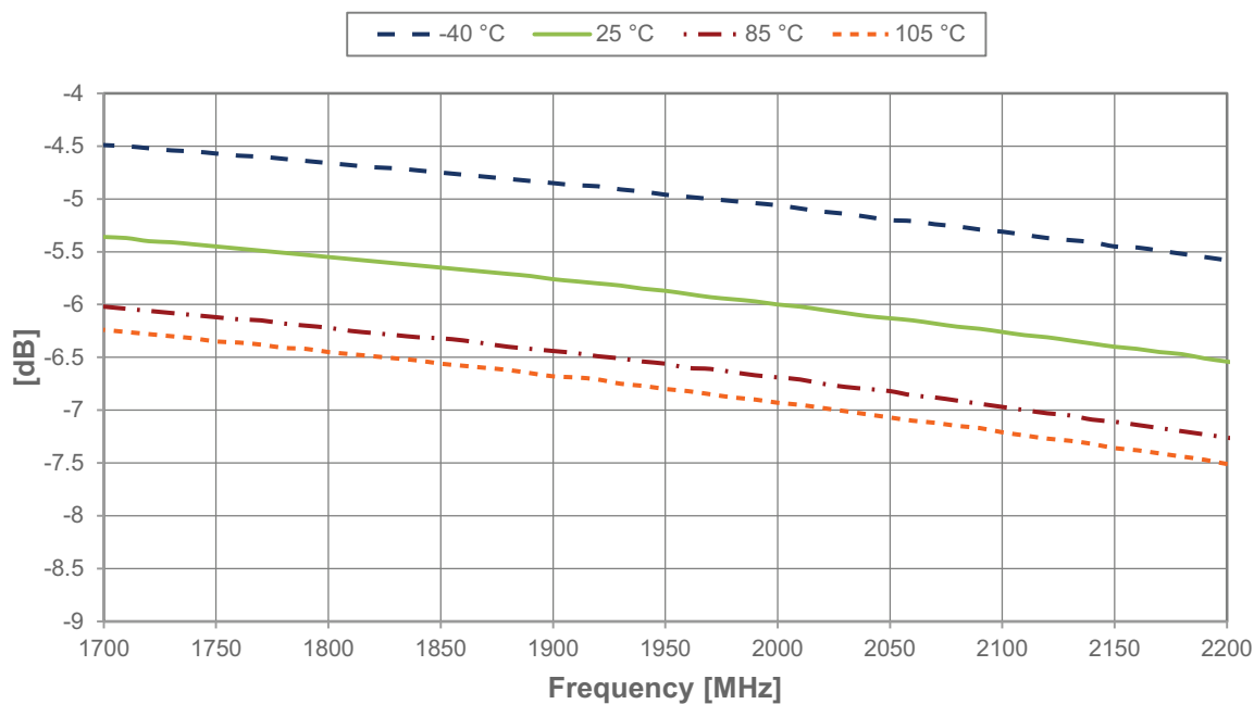
Figure 19 • Insertion Loss—Reference States
