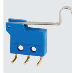
B2-5: Single Break, Subminiature with Integral Lever
