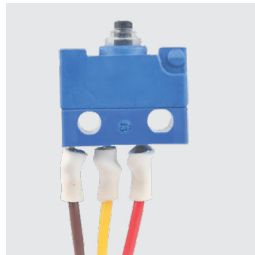
B3S: Double Break, Sealed, Snap Action Subminiature
