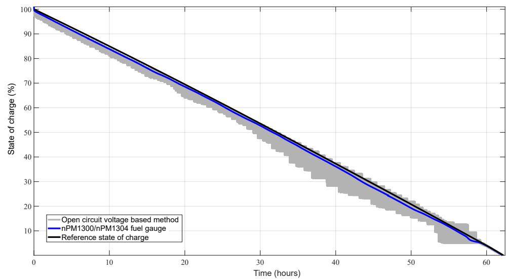
Figure 5: Comparing fuel gauge estimates against OCV based look-up table method
