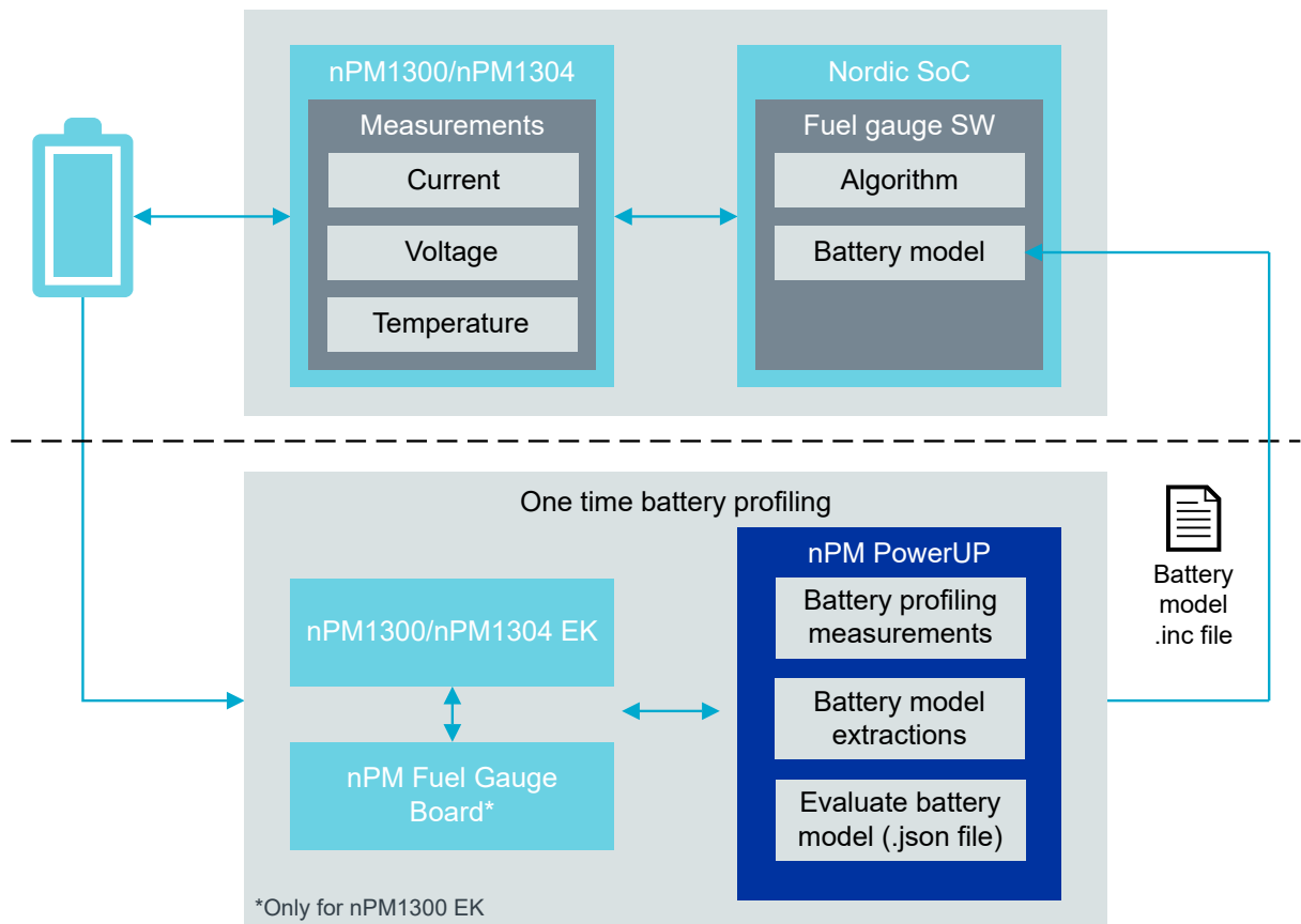
Figure 1: nPM1300 and nPM1304 fuel gauge with battery profiling
