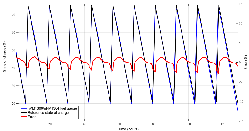
Figure 4: Estimated and measured state of charge (%) over several charge and discharge cycles
