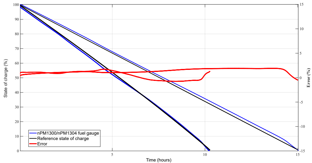
Figure 3: Estimated and measured state of charge (%) at different loads
