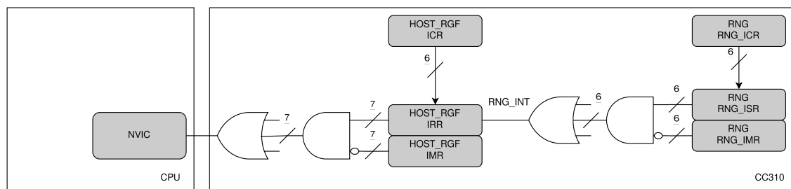
Figure 15: CRYPTOCELL interrupt handling
