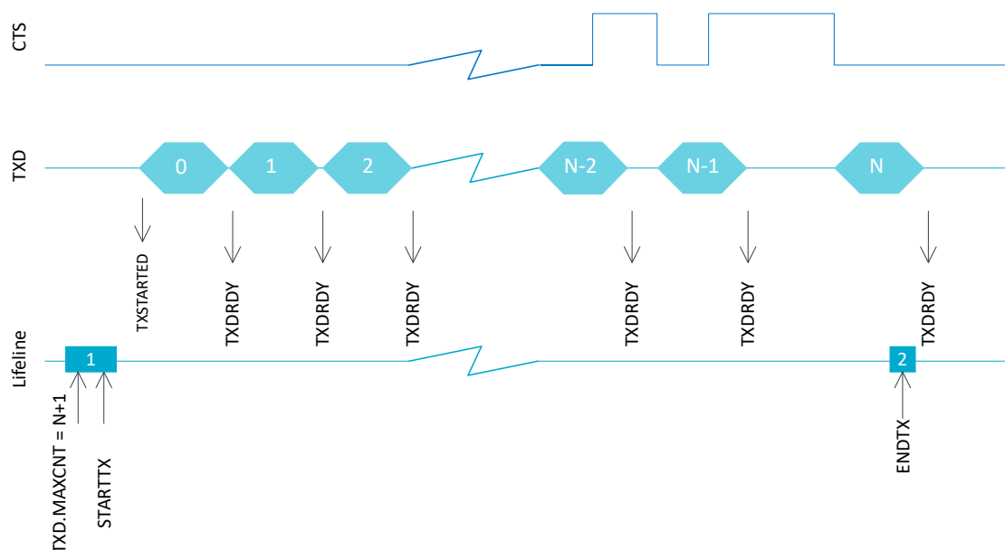
Figure 110: UART transmission
