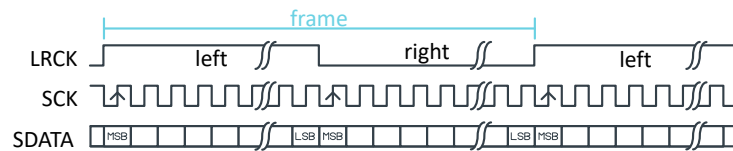
Figure 32: Aligned format. CONFIG.SWIDTH equaling half-frame size.
