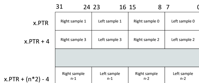
Figure 33: Memory mapping for 8 bit stereo. CONFIG.SWIDTH = 8Bit, CONFIG.CHANNELS = Stereo.
