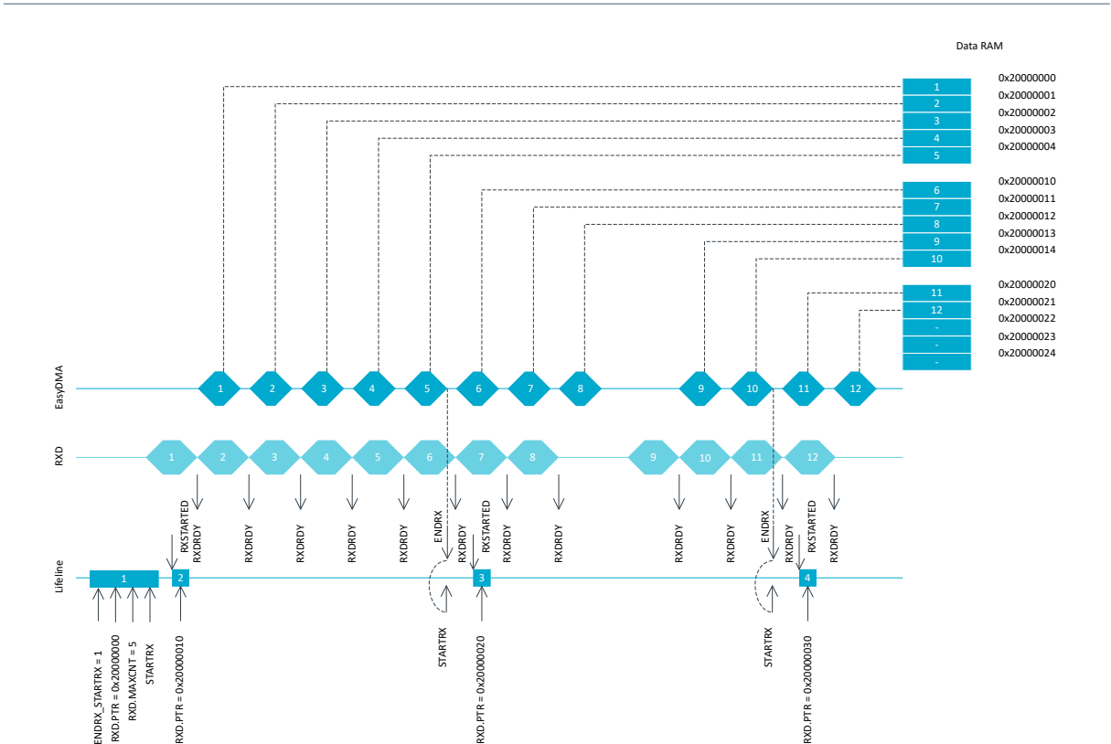
Figure 111: UARTE reception
