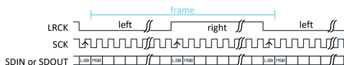
Figure 31: I2S format. CONFIG.SWIDTH equaling half-frame size.
