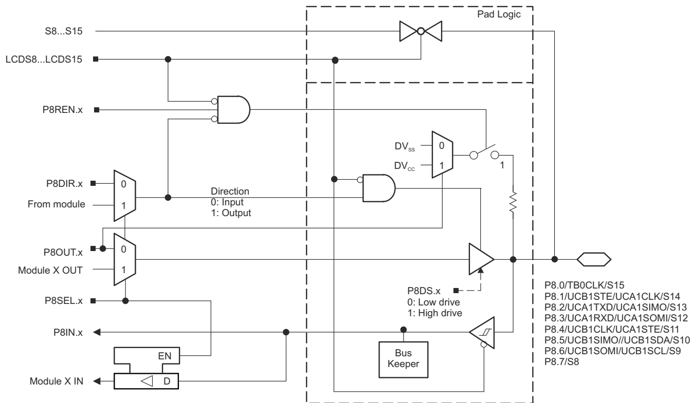
Figure 9-22. Port P8 (P8.0 to P8.7) Diagram
