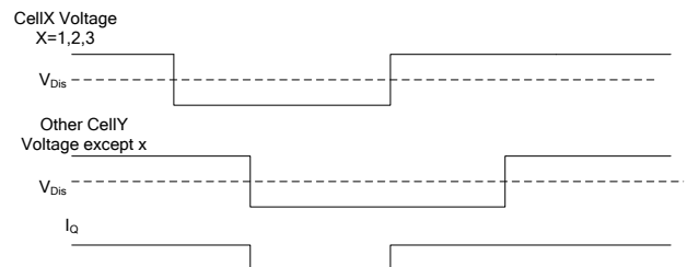
Figure 3: Over-Discharge Status
