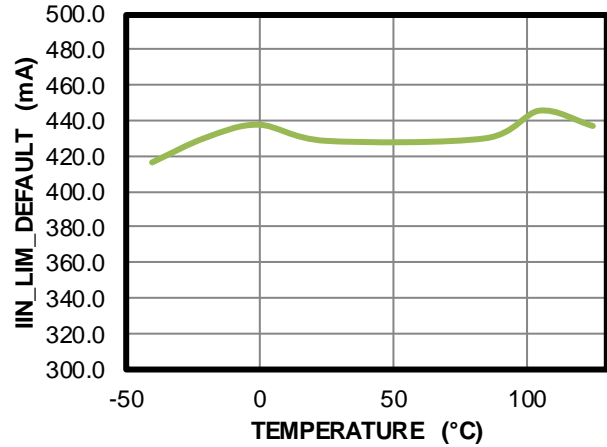
I Limit_455mA vs. Temperature
