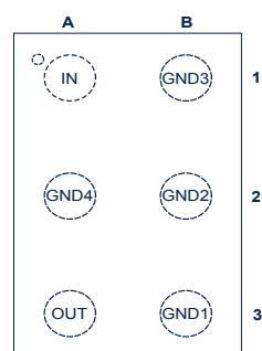
Figure 11. Top view
