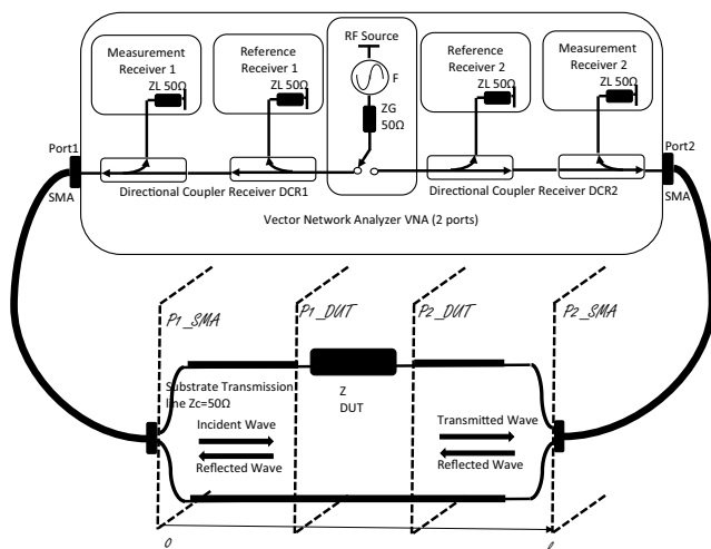
Fig. 4a - Test setup for S parameter measurement with 2 port VNA. Port1 is connected to the RF source.
