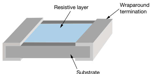
Fig. 6 - Wraparound design
