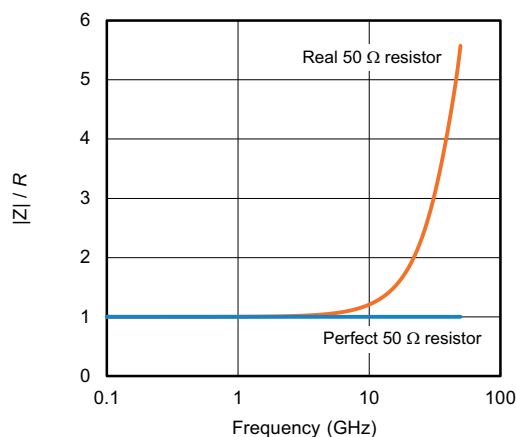
Fig. 3 - As the frequency increases, the impedance deviates from 50 \Omega
