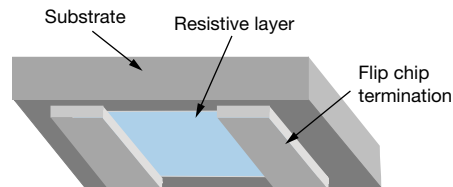
Fig. 7 - Flip chip design
