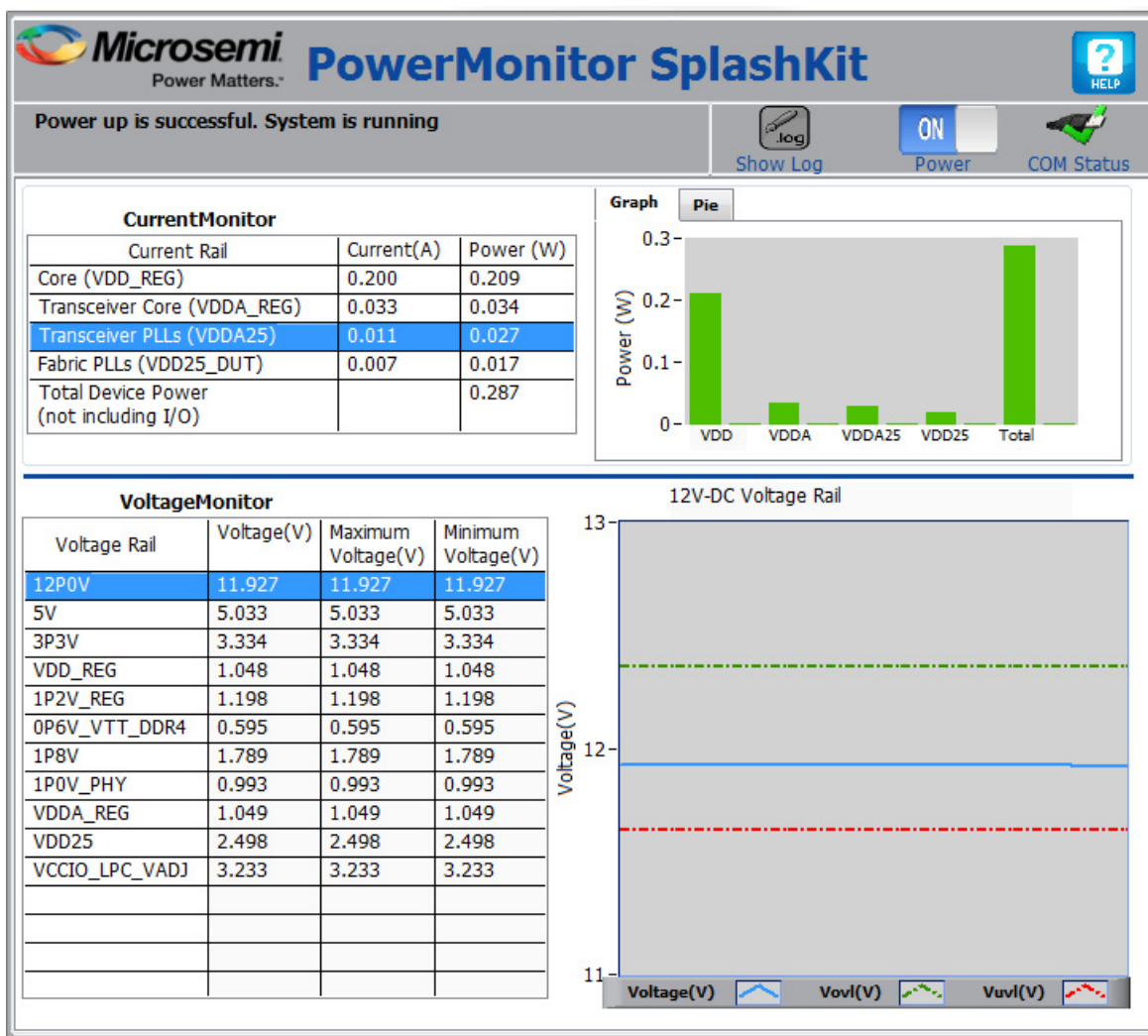
Figure 21 • PowerMonitor GUI
