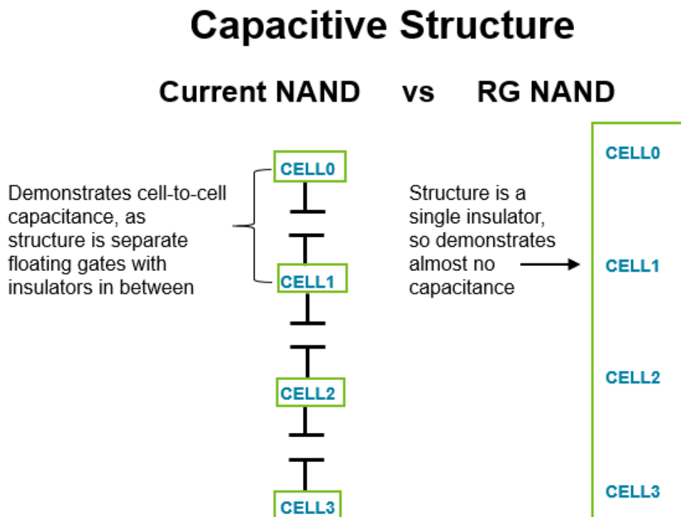
Figure 1: Current Traditional Gate NAND Capacitive Structure vs. Replacement Gate
