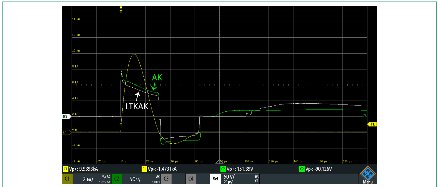
Low Vclamp Performance (SMD LTKAK vs. Axial Leaded AK)
